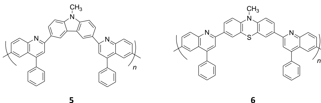
Figure 1.4 – Structures of alternating D-A co-polymers
