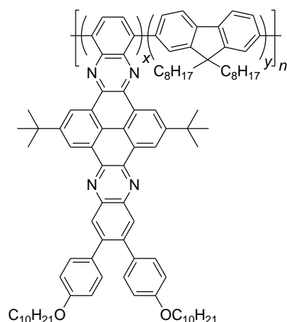
Figure 1.24 – Structure of F/bisphenazine co-polymers
