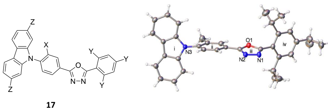
Figure 1.11 – Structure of high triplet level bipolar molecules where X = H, Me; Y = H, Me, i Pr, t Bu; Z = H, OMe and X-ray molecular structure of molecule with X = Me; Y = i Pr; Z = H, showing the twist between carbazole and phenyl/oxadiazole moieties
