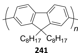
Figure 5.1 – Structure of PFO
