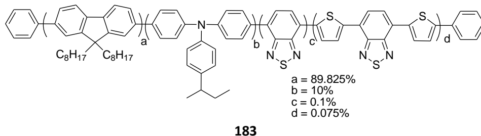
Figure 3.23 – Structure of analogous co-polymer without S
