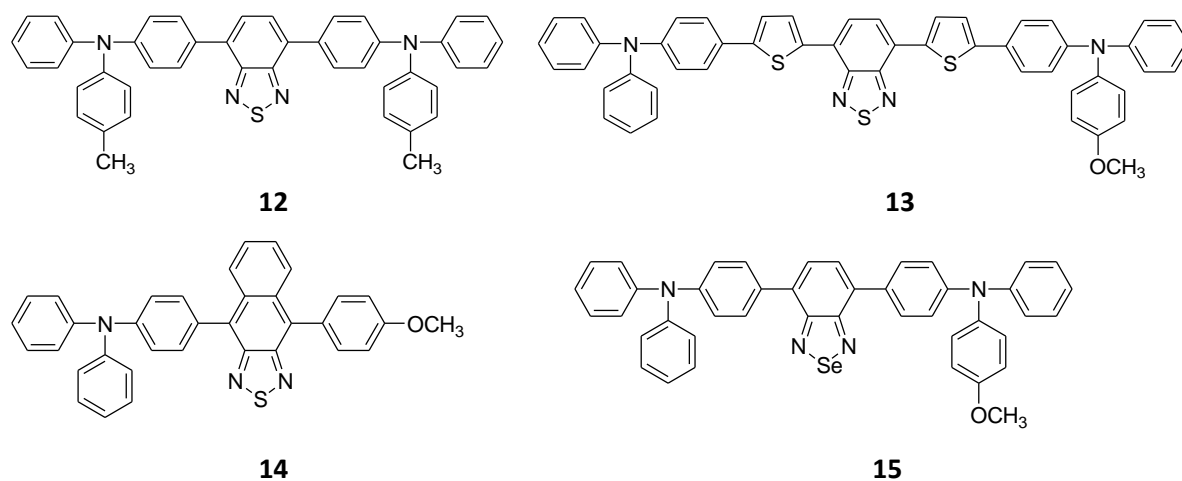
Figure 1.9 – Structures of red-emitting D-A systems
