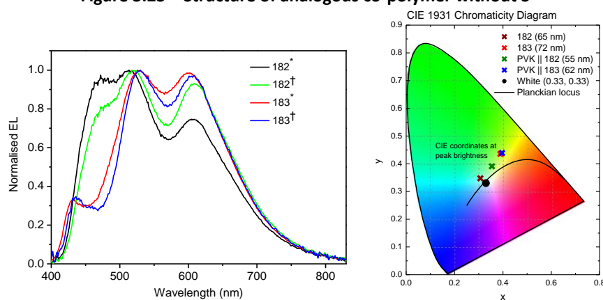
Figure 3.24 (a) – EL of devices with S (182) and without S (183); (b) Corresponding CIE diagram Device architectures: *ITO // PEDOT:PSS (50 nm) // 182 or 183 // Ba (4 nm) // Al (100 nm); †ITO // PEDOT:PSS (50 nm) // PVK (30 nm) // 182 or 183 // Ba (4 nm) // Al (100 nm)
