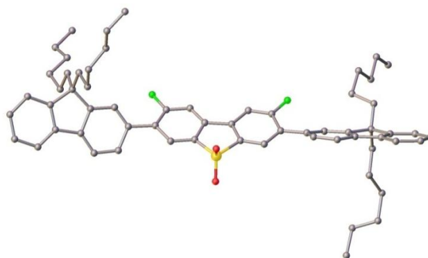
Figure 2.7 – The single crystal molecular structure of the FS r F trimer (126) (H atoms omitted; F, S and O atoms are shown in green, yellow and red, respectively) (Structure determined by Dr. A. S. Batsanov)
