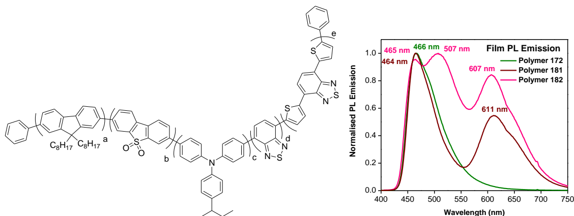
Figure 3.19 – Structure and thin film PL emission of the arylamine-based co-polymers
