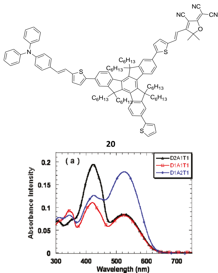
Figure 1.13 – Structure of a star-shaped donor- \pi -acceptor system and absorption spectra of this compound (= D1A1T1) and analogous compounds in THF solution ( 10^{-6} M)
