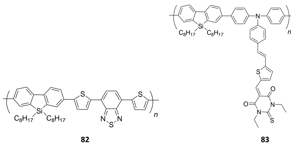
Figure 1.39 – Structures of dibenzosilole-based co-polymers for solar cell applications
