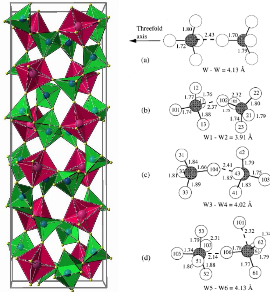
Figure 4-6 Left. Polyhedral representation of the pressure induced \gamma - ZrW_2O_8 phase. Right. a) representation of the linear orientation of the WO_4 tetrahedra in \alpha - ZrW_2O_8 ; b), c) and d). representation of the three different pairs of WO_n polyhedra and bond lengths in the \gamma - ZrW_2O_8 (Oxygen atoms are white and tungsten atoms are shaded).
