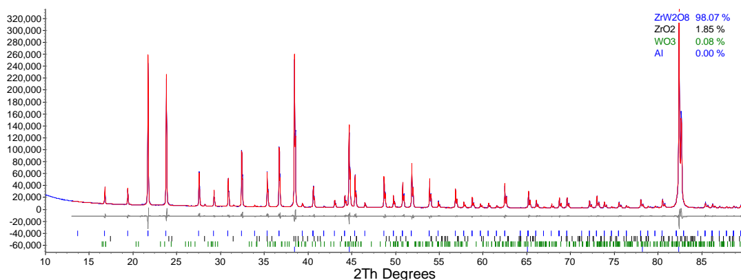
Figure 4-11 Rietveld refinement plots of the X-ray diffraction data from the room temperature enriched \alpha - ZrW_2O_8 (d5_01959). Rwp = 5.576 %
