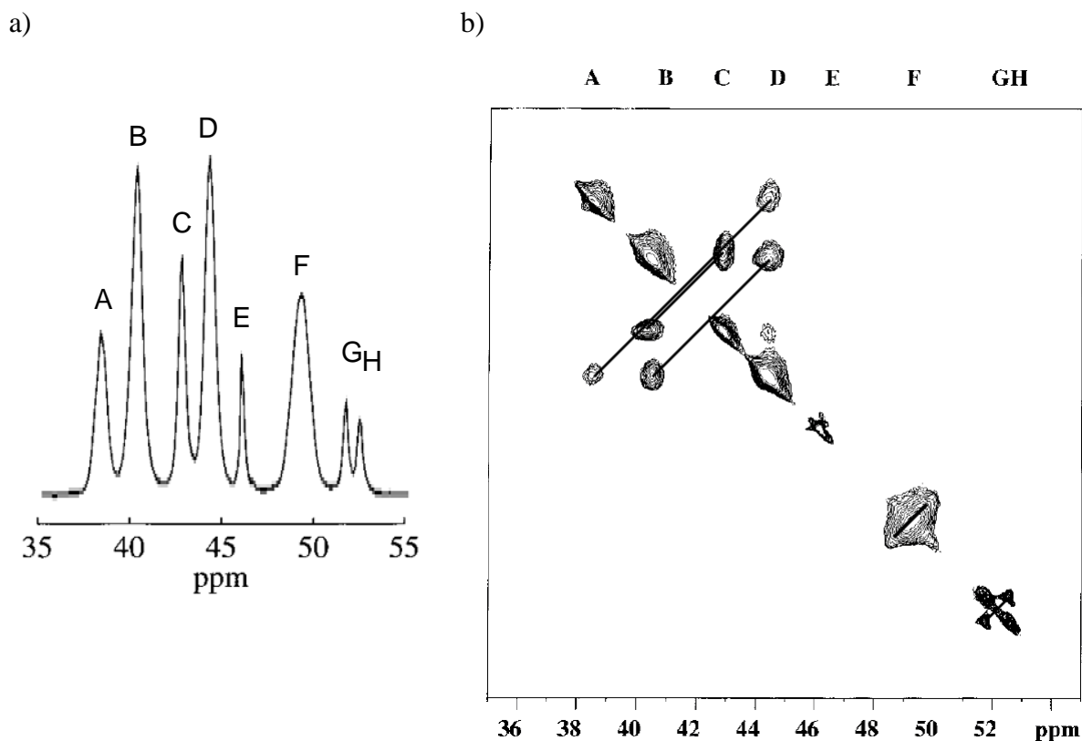
Figure 2-3 1D ^{31}\text{P} NMR spectra (a) and 2D TOBSY MAS ^{31}\text{P} NMR experiment (b) on \text{TiP}_2\text{O}_7 recorded at 5.2 kHz (14) . The solid line show the through bond P-O-P connectivities.
