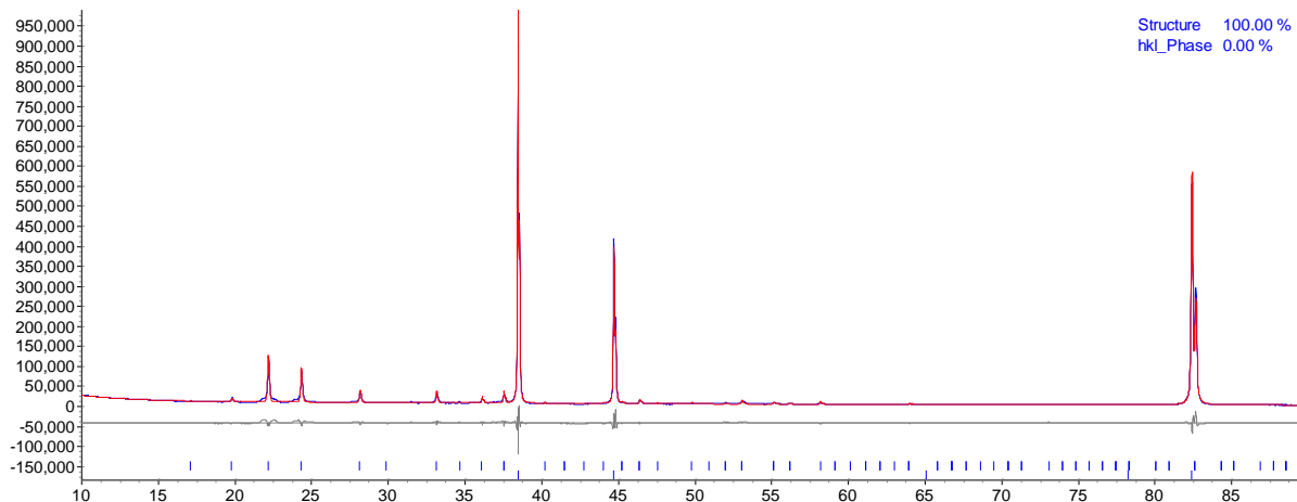
Figure 4-10 Rietveld refinement plots of the X-ray diffraction data from the room temperature enriched ZrW_2O_8 \cdot xH_2O (d9_01958). Rwp = 9.56 %
