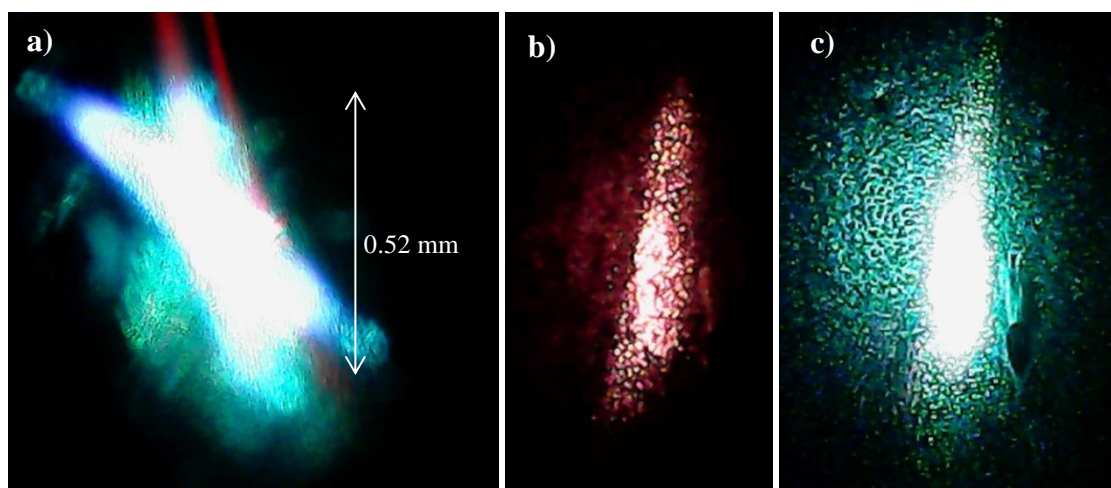
Figure 3.6. Image of a) spatially overlapping pump and probe beams, and b) probe and c) pump beams by their own on the surface of a glass window.
