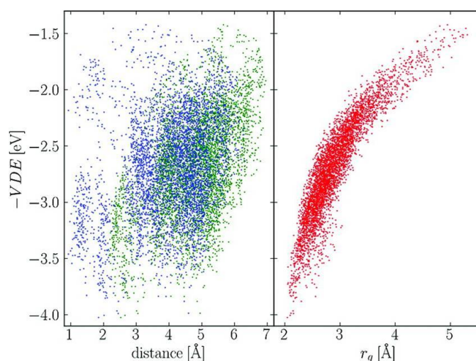
Figure 1.17. Dependence of the VDE on the distance of the excess electron from the centre of the water cluster (green- data using the average distance of the electron from the cluster centre of mass; blue- using the distance between the centre of the electron and the cluster centre of mass) and its radius of gyration. Reprinted with permission from ref. [99]. Copyright (2015) American Chemical Society.
