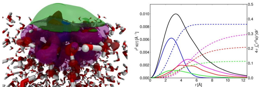
Figure 1.18. Left: Snapshot from the performed QM/MM MD simulations. Green sphere represents electrons spin density sticking out to the vapour phase. Right: The excess electrons spin density distribution (black), with indicated contributing parts from inner cavity 37% (blue), overlapping with water molecules 21% (red), diffuse part 31% (magenta) and part in the vapour phase 11% (green). Reprinted with permission from ref. [101]. Copyright (2015) American Chemical Society.
