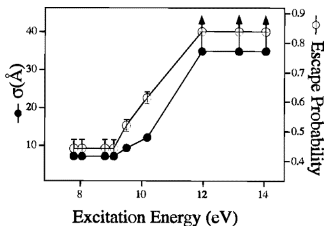
Figure 1.4. Escape probability (open circles) and the width of initial electron distribution (filled circles) due to the excitation energy. Reprinted with permission from ref. [29] Copyright (2015) American Chemical Society.
