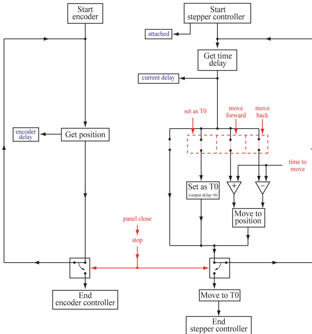
Figure 3.16. Scheme of the operations performed by program ‘Stage control’ as described in text, with controls showed in red and indicators showed in blue.
