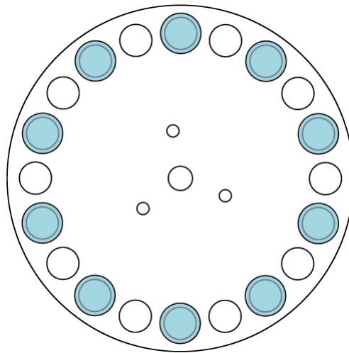
Figure 3.12. Custom chopper wheel made out of Teflon with a SF10 or CaF 2 glass window, for 1320 nm and 800 nm fundamental beam respectively, placed in every second hole. The technical drawing is shown in appendix B.
