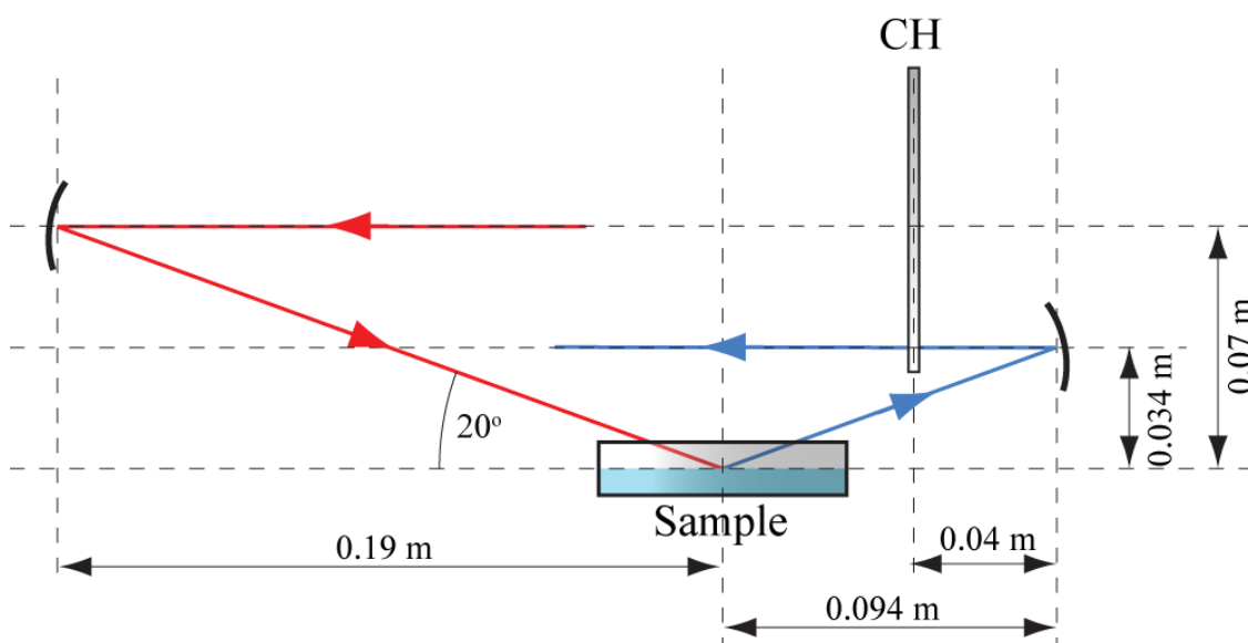
Figure 3.8. Scheme of the relative distances and angles at which curved mirrors CM3-CM4, sample and chopper wheel are kept between each other.
