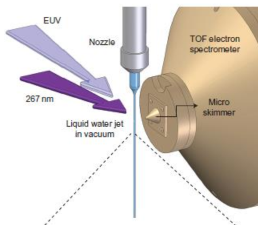
Figure 1.16. Graphic representation of the liquid microjet experiment. A beam of water is generated by pressing a liquid solution through a micrometre diameter nozzle using a high pressure pump. The hydrated electron is produced by a pump light beam in distance around 1-2 mm from the nozzle. Subsequently, electron is probed by its photoemission induced by an ultraviolet beam. Kinetic energy as a function of time can be then detected through the time of flight spectrometer, into which emitted photoelectrons access through the skimmer. Reprinted by permission from Macmillan Publishers Ltd: Nature Chemistry ref. [66], copyright (2015).
