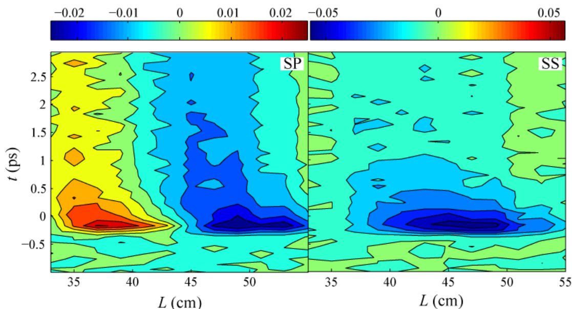
Figure 4.8. Kinetics observed for SP (left) and SS (right) polarization combinations in case when pump and probe has planes of incidence different by \sim 3.5^\circ . Instead of measuring directly, due to the risk of the signal originating from the mixture of p and s polarization, data here were obtained by taking a number of small perturbations ( < 5^\circ ) from the purely p or s polarization of the incident fundamental beam and picking the component that varies as \cos^2 \vartheta_p , where \vartheta_p indicates the angle away from the pure polarization.
