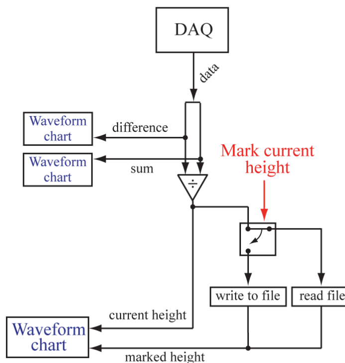
Figure 3.15. Scheme of the operations performed by the “Quadrant Photodiode” program as described in text, with indicators showed in blue.
