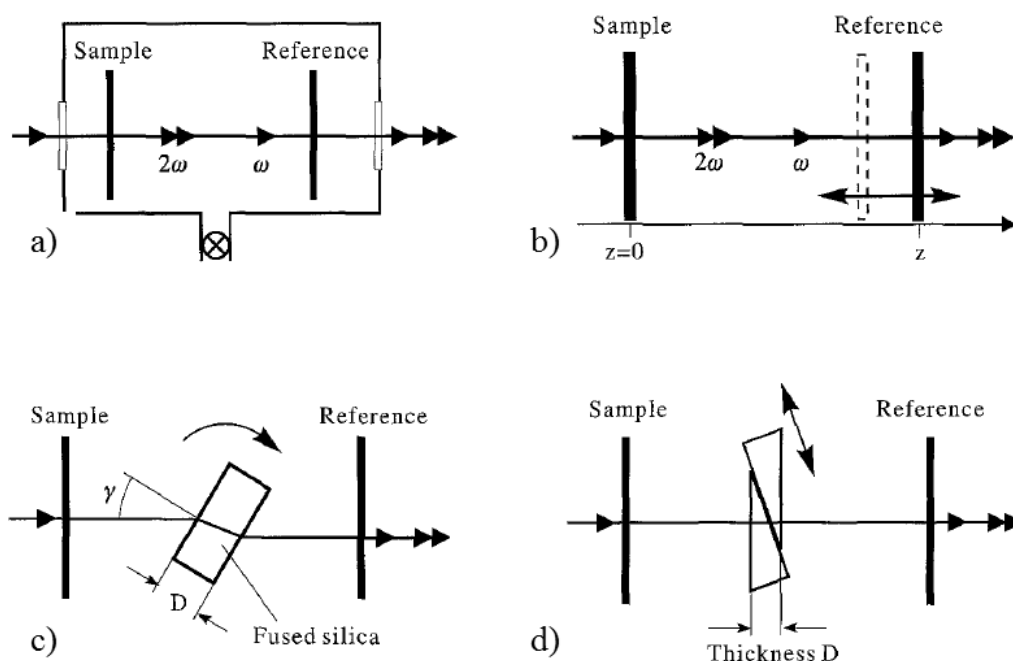
Figure 2.5. Basic schemes of four illustrative methods of controlling the phase difference in the interference SHG measurement. a) Gas cell, beams propagate in the gas cell, with the phase difference altered by a change of the gas pressure; b) variation of the distance, the phase difference is controlled here by changing the path length over which SH and fundamental beams propagate before generating the LO; c) rotating plate, both beams go through a glass or fused silica plate, and the phase is altered by change of the propagation length in glass plate, which is achieved by rotation of the plate; d) pair of wedges, both beams go through glass or fused silica wedges, the phase change controlled by adjusting the thickness D as shown. Reprinted from ref. [165] with permission of Springer.
