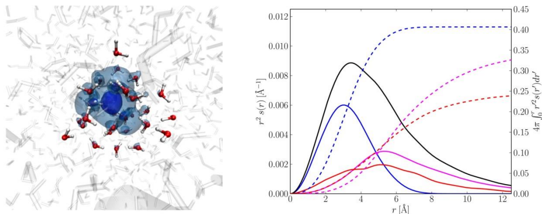
Figure 1.12. Left: snapshot from the performed simulation. The blue sphere represents the electron spin density distribution, the colour and transparent ball and stick models represents water molecules treated quantum mechanically and molecular mechanically, respectively. Right: The excess electron spin density distribution (black) with indicated contributing parts from inner cavity (blue), overlapping with water molecules (red) and diffuse part (magenta). Full lines correspond to spin density and dashed lines to integrals. Adapted with permission from ref. [70]. Copyright (2015) American Chemical Society.
