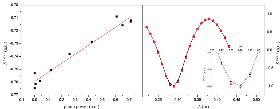
Figure 3.25. Left: Interference signal obtained with the varied pump power, taken at the distance between the surfaces L = 0.29 m, with the red line indicating linear fit. Right: The interference signal, with varying distance L , in absence of pump beam (red circles) and with a pump beam at maximum power (black squares), with a magnification of the destructive interference peak in the inset.
