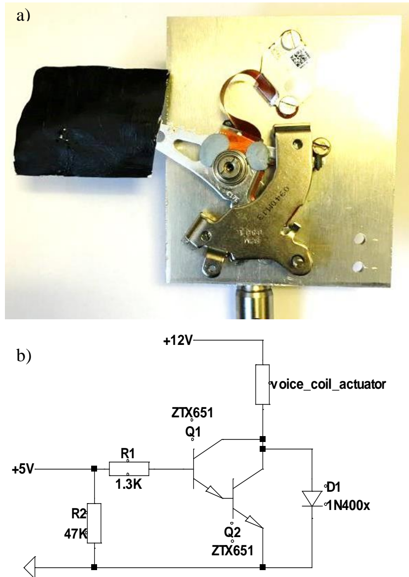
Figure 3.3. a) Picture of the shutter. b) Scheme of the circuit diagram for the shutter. A 5 V TTL input triggers transistors to enable a 12 V supply to flow through the system and thus move the shutter. R1 is 1.3 k \Omega resistor, R2 is 47 k \Omega resistor, Q1 and Q2 are ZTX651 bipolar (BJT) single transistors and D1 is 1N400x series diode.
