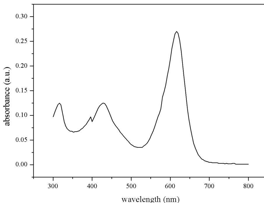
Figure 3.22. Absorption spectrum of MG solution in water.
