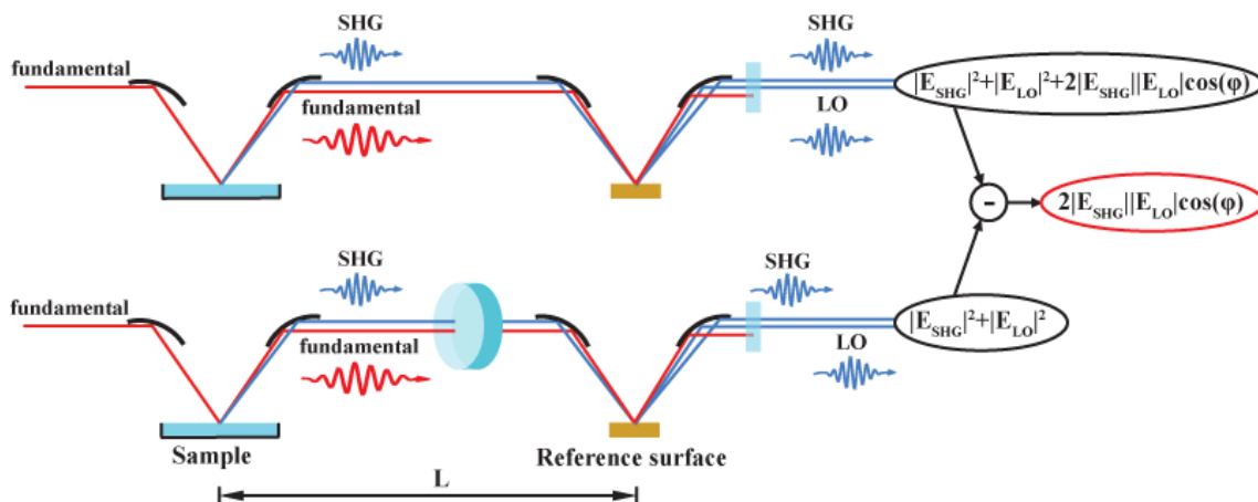
Figure 3.10. Schematic representation of the lock-in measurement. The top path shows the interference of a SHG field generated from the surface of interest with a LO from a reference surface. The bottom path shows the same, but the SHG and fundamental that will generate the LO are offset in time by the presence of a dispersive material leading to a group-velocity mismatch. In such a case, no interference takes place. The difference between the measurements recovers the interference term of interest.
