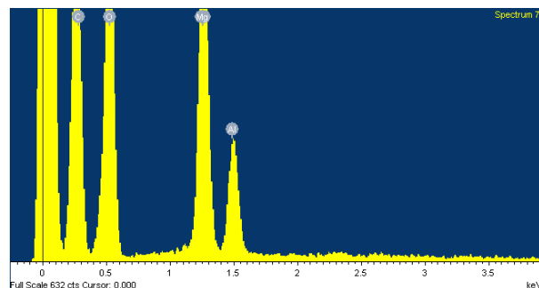
Figure 2.10 Typical analysis using scanning electron microscope energy dispersive X-ray spectroscopy showing a) MgAl(CO_3) -layered double hydroxide of Mg:Al 3:1, prepared by co-precipitation as described in section 3, with area of analysis marked and b) EDX analysis element plot.
