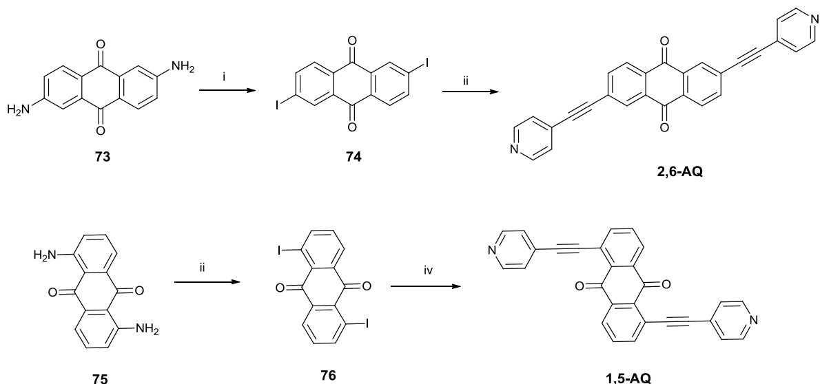
Scheme 6.1 synthesis of 2,6-AQ and 1,5-AQ
