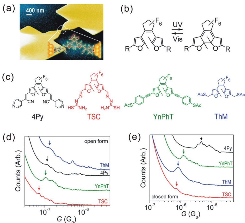
Fig. 1.14 (a) An illustration of an Au – 4Py – Au junction. (b) Sketches of open (left) and closed (right) forms of photochromic molecules (difurylenes). (c) Structures of the four different molecules, 4Py, TSC, YnPhT, and ThM, respectively, (d,e) Conductance histograms of photochromic molecular junctions for open and closed forms of all four molecules. (Reproduced from reference 41 )
