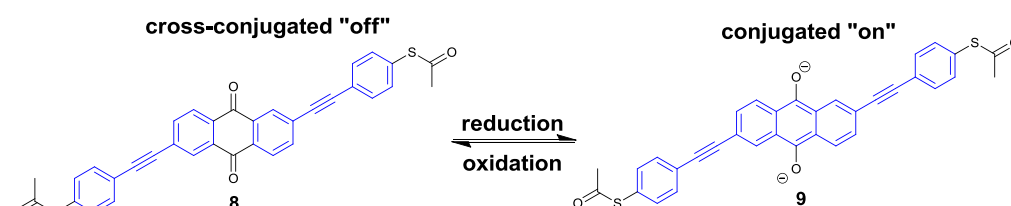
Fig. 1.16 “On” and “off” states of anthraquinone centred OPE molecules with sulfur anchoring groups.
