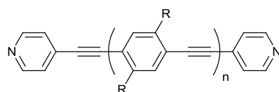
Chart 2.1. Structures of the OAE derivatives studied in this work.
