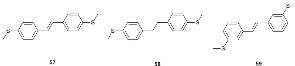
Fig. 3.5 Molecular structures of molecules studied in Aradhya's work. (Reproduced from reference 110 )
