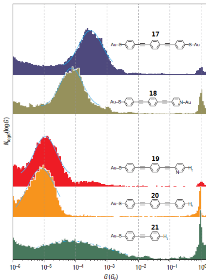
Fig. 1.22 Conductance histograms for molecules 17-21 . (Reproduced from reference 53 )
