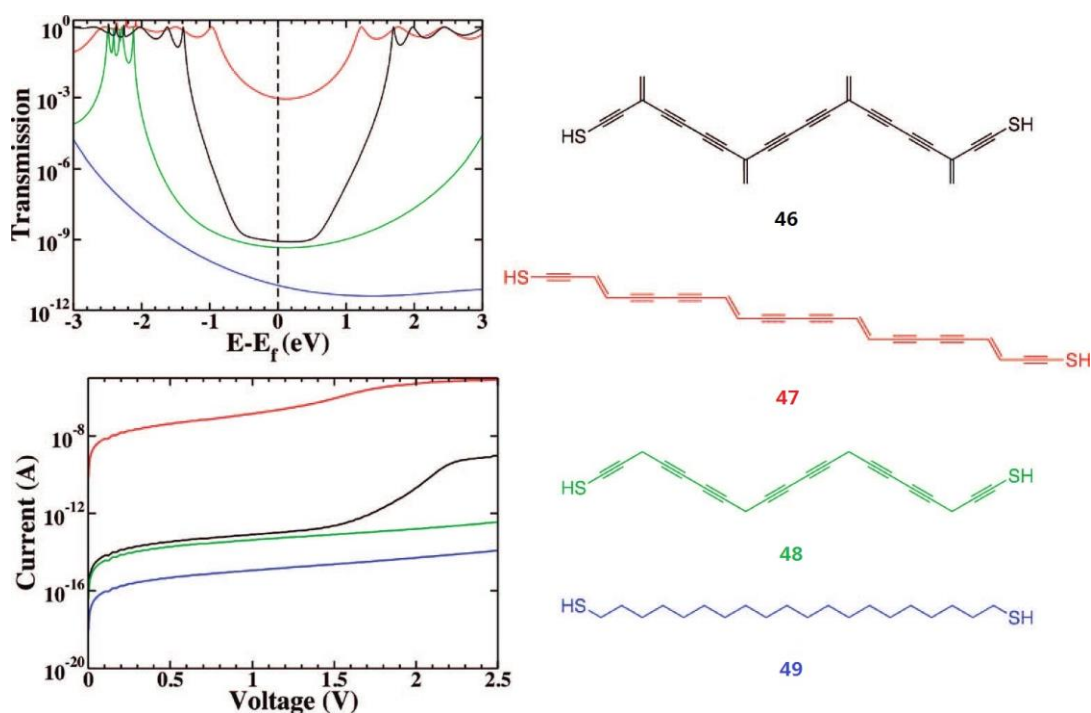
Fig. 3.1 Zero bias transmission as a function of energy, and current as a function of voltage, for a group of comparable molecules, illustrating the unusual transport characteristics of a cross-conjugated system. Specifically, an extended cross-conjugated molecule (46) is compared with its linearly conjugated counterpart (47) and with a partially conjugated (48) and a saturated (49) system of a similar length. (Reproduced from reference 107 ).
