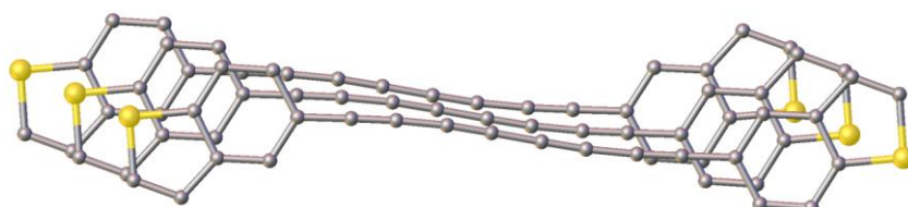
Fig. 5.3 Crystal packing of BTh4
