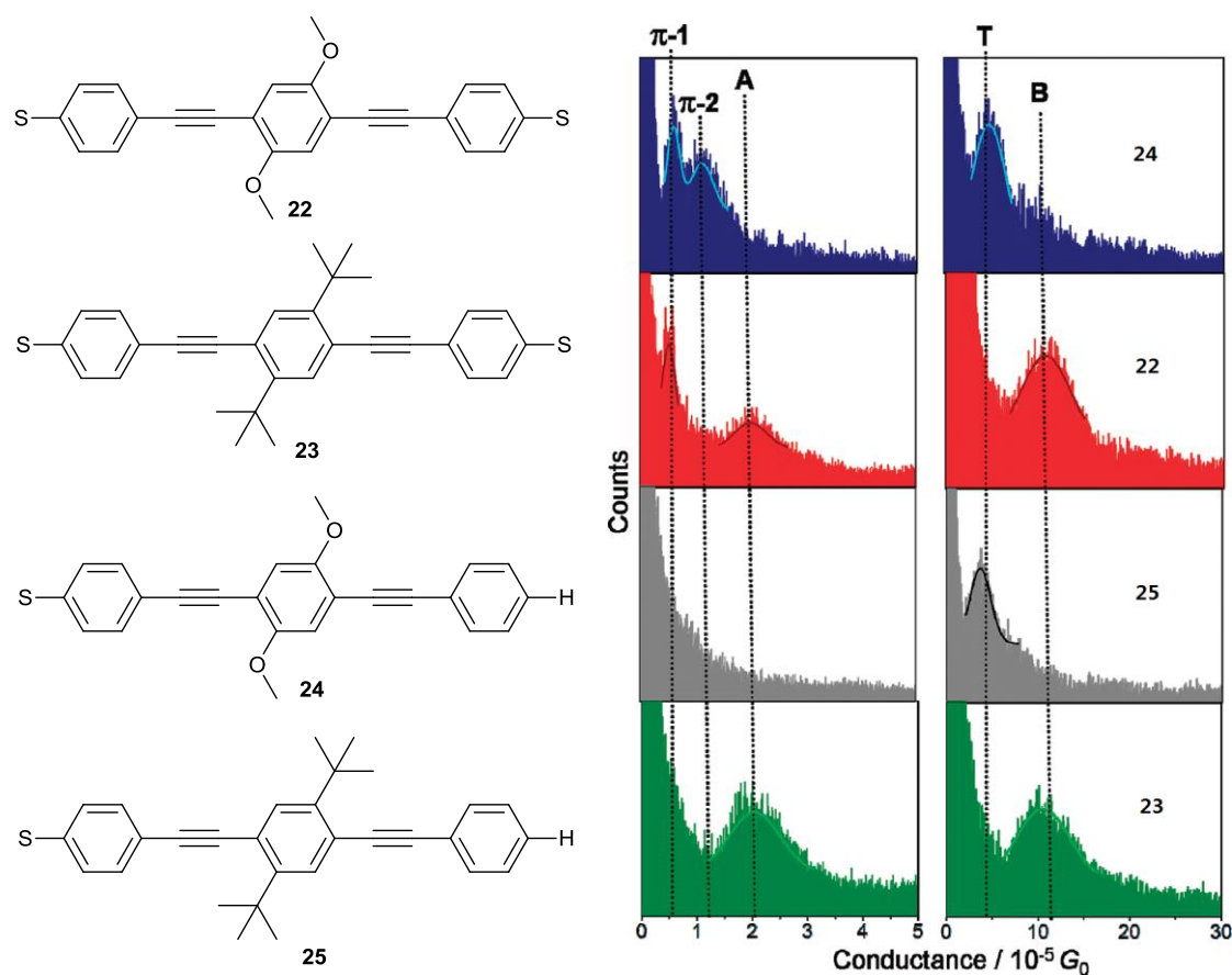
Fig. 1.23 Molecular structures and histograms for conductance. Left panel: low set point current ( I_0=5 nA, and U_t=0.6 V). Right panel: high set point current ( I_0=60 nA, and U_t=0.6 V). (Reproduced from reference 54 )
