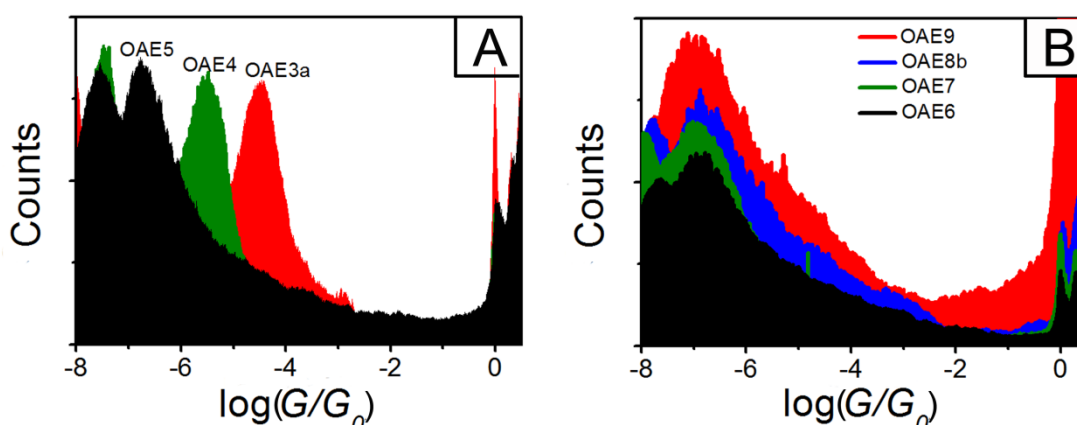
Fig. 2.11 All-data point 1D conductance histograms of OAE-derivatives as constructed from 2000 individual conductance vs. relative distance traces as plotted in Fig. 2.12.
