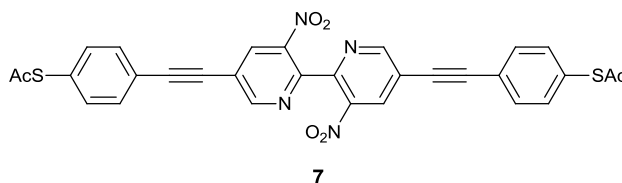
Fig. 1.13 Molecular structure of bipyridyl-dinitro oligo(phenyleneethynylene) dithiol (BPDN-DT) investigated in Lörtscher's work. (Reproduced from reference 37 )
