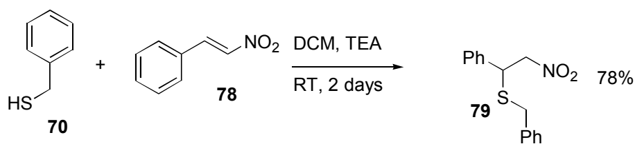
Scheme 26
