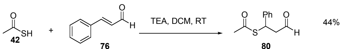
Scheme 27
