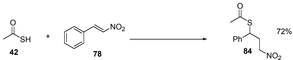
Scheme 31
