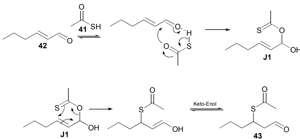
Scheme 20 – proposed mechanism
