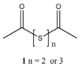
Figure 15 – possible structures
