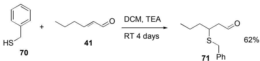
Scheme 22
