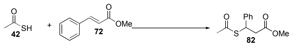
Scheme 29
