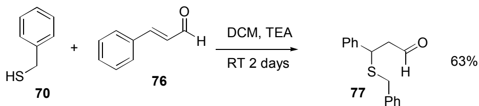
Scheme 25
