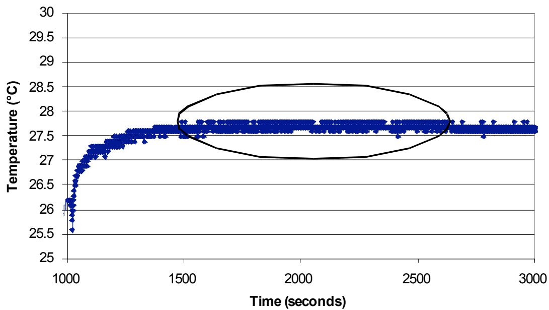
Figure 13 Investigation of effect of amine catalysis, with expansion to show plateau
