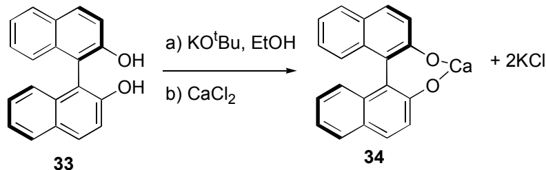
Scheme 15 Production of calcium-BINOL
