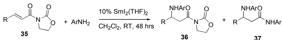
Scheme 16 Use of a samarium iodide complex as an effective aza-Michael catalyst
