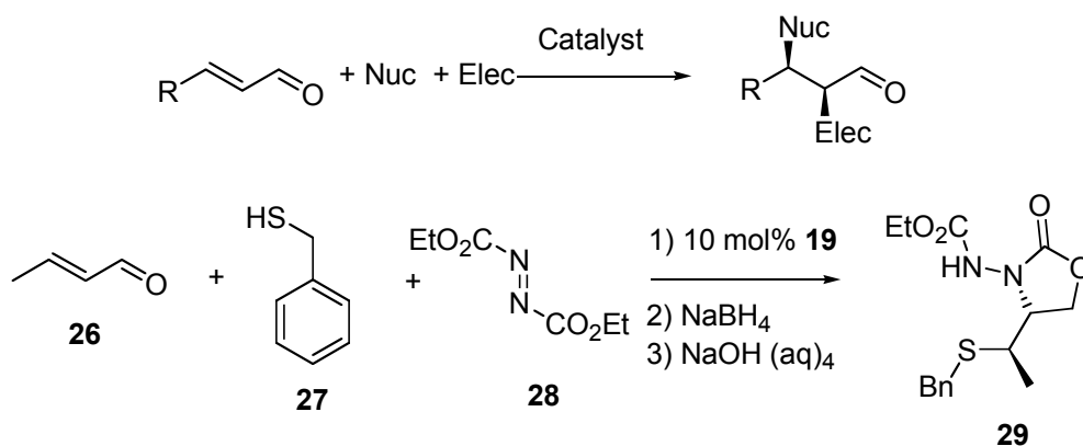
Scheme 9 Principle of MCR, with example
