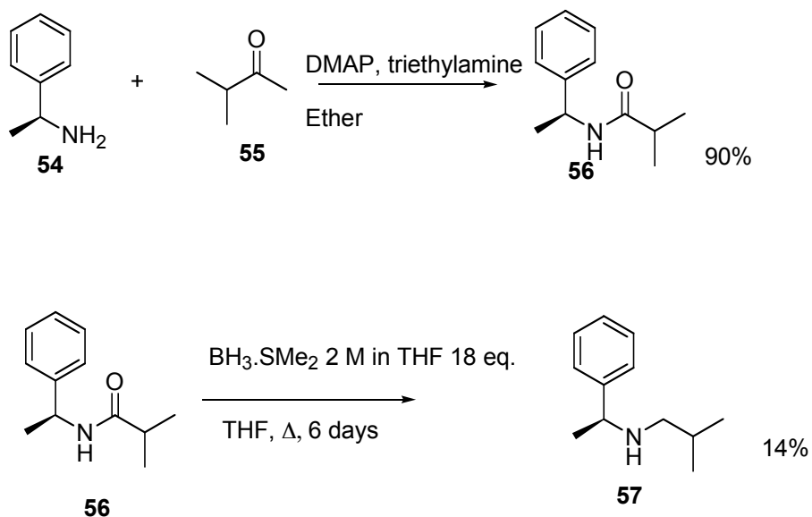
Scheme 19 Synthesis of N-isobutyrylamino catalyst
