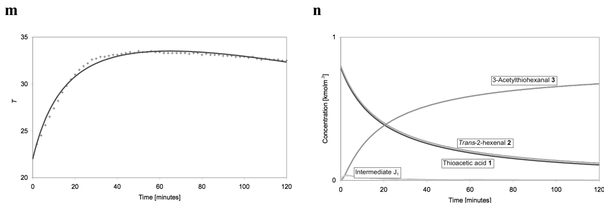
Figure 10. Actual and simulated temperature profiles, and predicted composition profiles for reaction of thioacetic acid 42 with trans -2-hexenal 41 . a ; Actual and simulated temperature profile in toluene. b ; Predicted composition profile in toluene. c ; Actual and simulated temperature profile in chloroform. d ; Predicted composition profile in chloroform. e ; Actual and simulated temperature profile in propionitrile. f ; Predicted composition profile in propionitrile. g ; Actual and simulated temperature profile in THF. h ; Predicted composition profile in THF. i ; Actual and simulated temperature profile in petroleum ether. j ; Predicted composition profile in petroleum ether. k ; Actual and simulated temperature profile in acetonitrile. l ; Predicted composition profile in acetonitrile. m ; Actual and simulated temperature profile in DMF. n ; Predicted composition profile in DMF.
