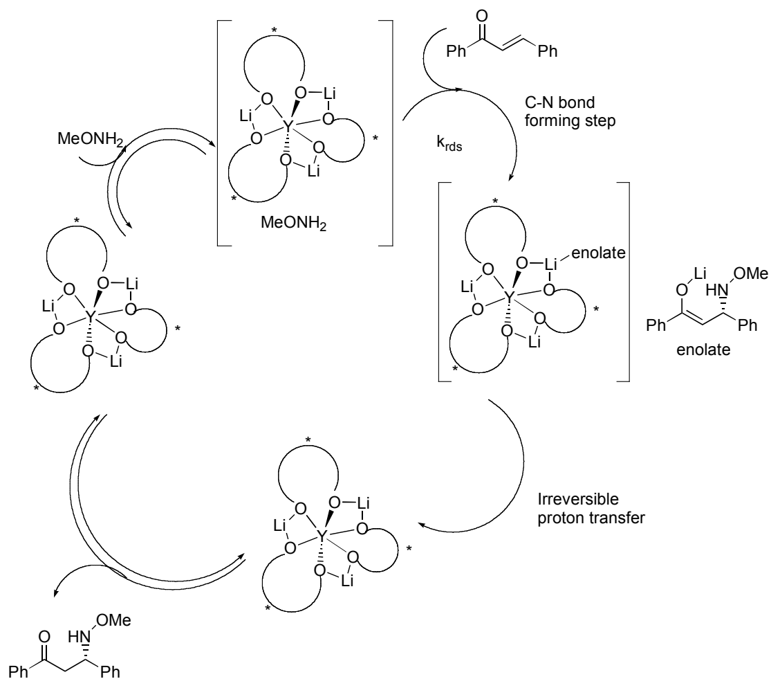
Scheme 18 Postulated catalytic cycle
