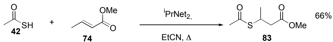
Scheme 30
