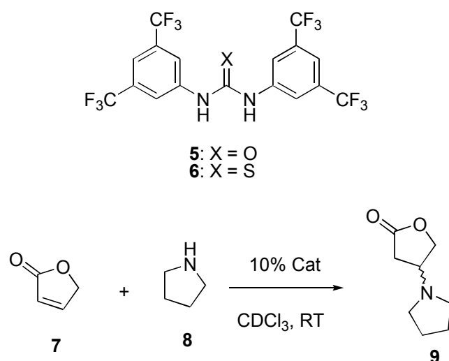
Scheme 3 catalysing the reaction of pyrrolidine with \gamma -crotonolactone
