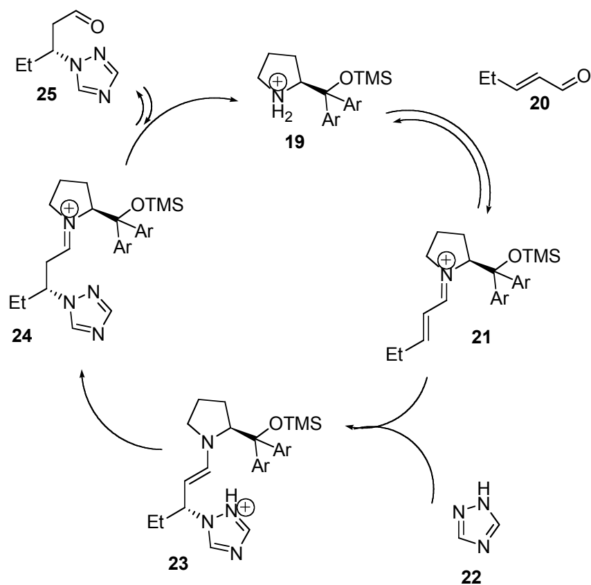
Scheme 8 Proposed mechanistic scheme, supported by DFT calculations
