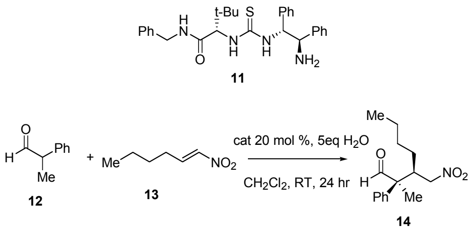
Scheme 4 Catalyst 11 shows high activity
