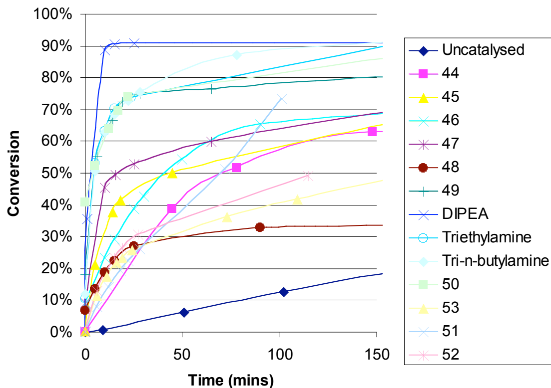
Figure 4 Graph of kinetic data for bifunctional and mono-functional catalysts, in D-chloroform, as listed in Table 1
