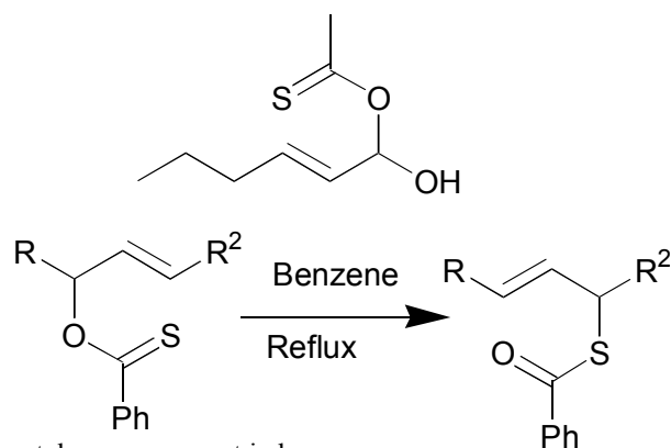
Scheme 21 hemi-thioacetal rearrangement in benzene
