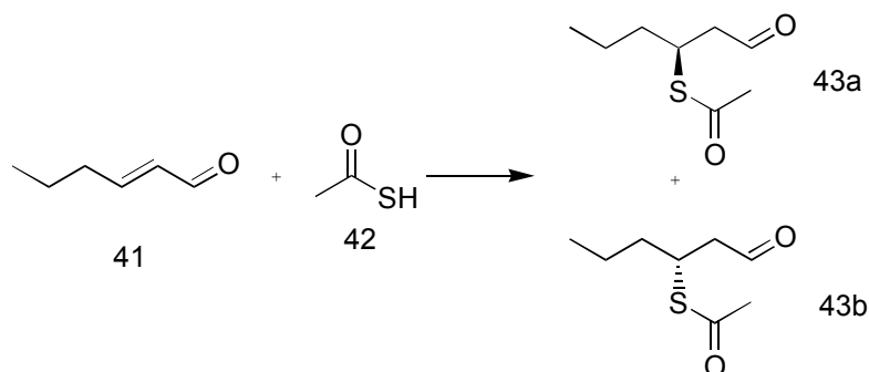
Scheme 18
