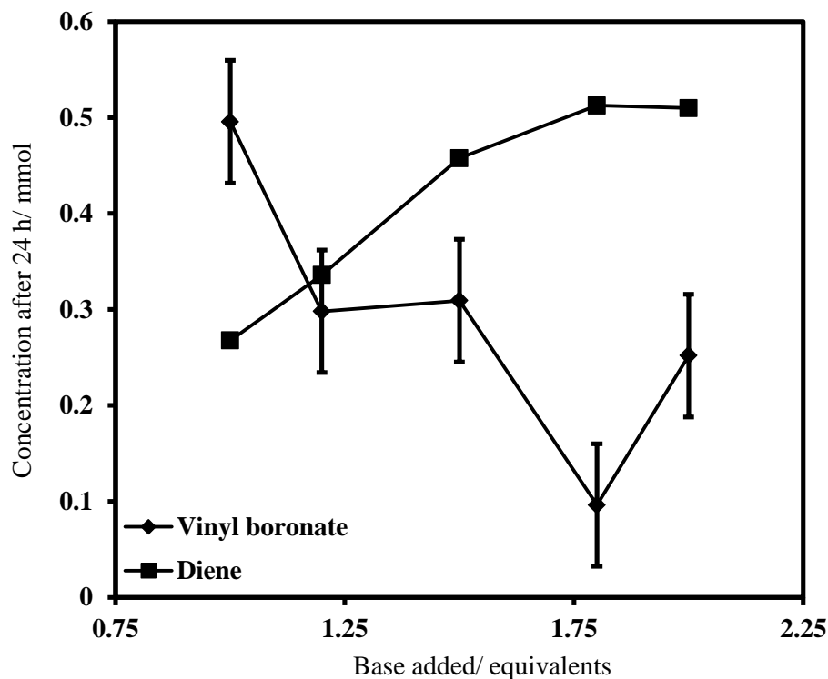
Figure 25 Graph showing the effect of base loading on the mmol concentration of vinyl boronate 42 and diene 276
