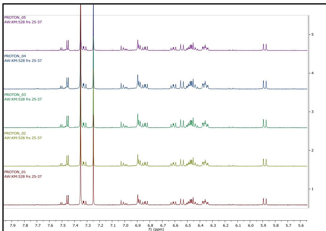
Figure 19 Stacked ^1\text{H} NMR spectra for debrominated pentaenyl xanthomonadin 234 , showing stability overnight.
