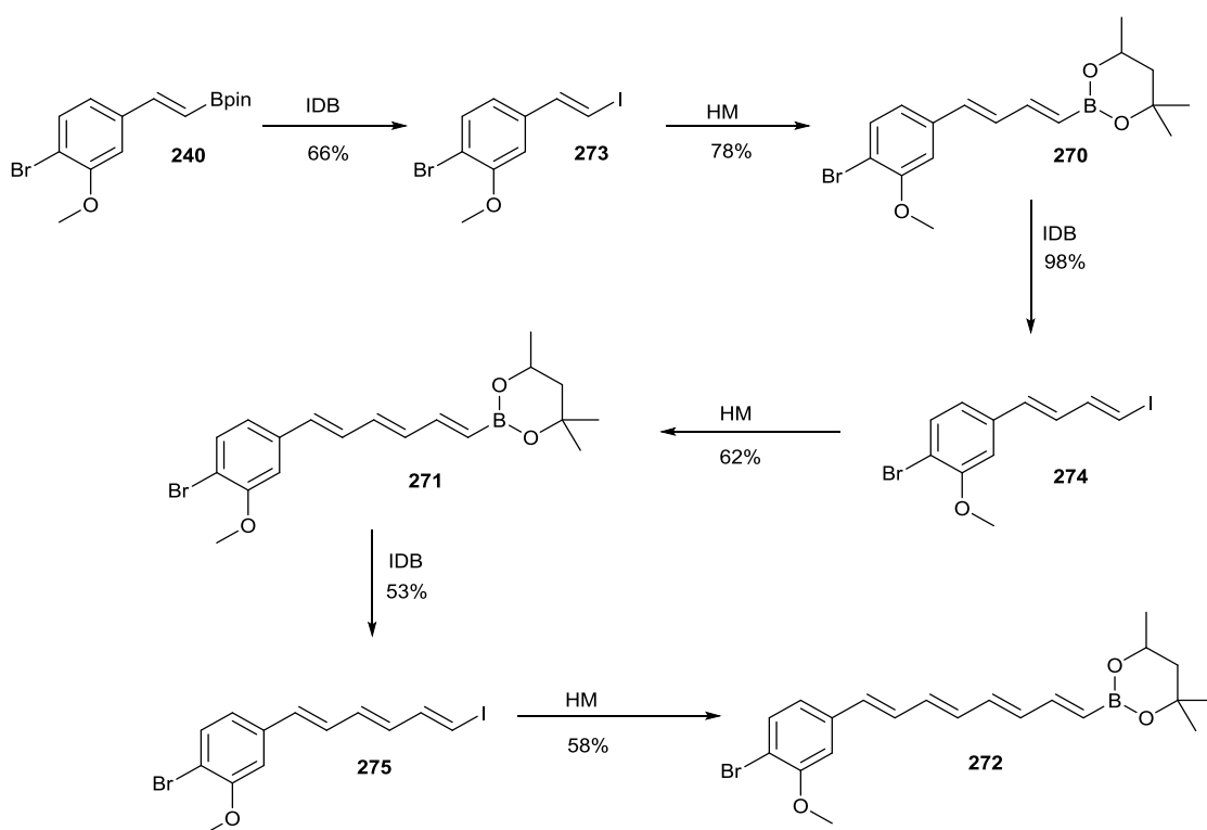
Scheme 51 Improved yields for the construction of aryl tetraenyl boronate 272
