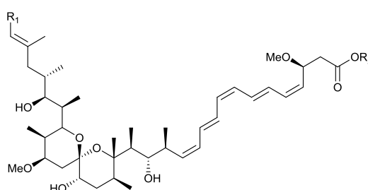
spirangien A 98 R_1 = \text{Me} , R_2 = \text{H} spirangien B 99 R_1 = \text{Et} , R_2 = \text{H}
