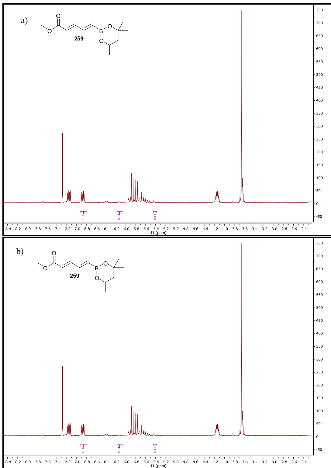
Figure 29 ^1\text{H} NMR spectra for the HM coupling between iodoacrylate 229 and vinyl boronate 42 under a ) the group's original conditions and b ) the newly optimised conditions.
