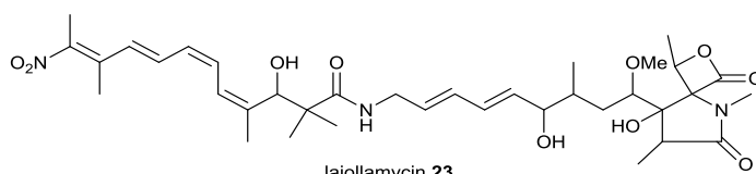
lajollamycin 23
