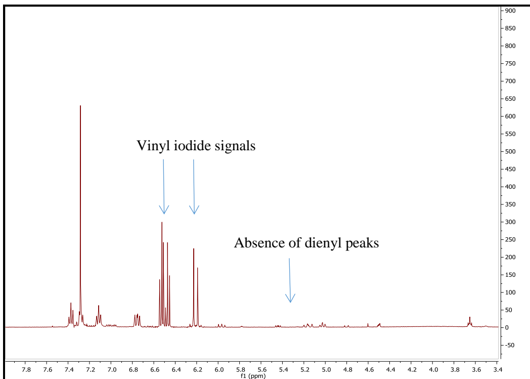
Figure 24 Crude ^1\text{H} NMR spectrum, showing the unreactivity of vinyl iodide 269 towards itself under HM conditions.
