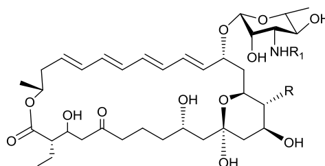
CE-108 13 R = COOH CE-108B 14 R = CONH 2 CE-108C 15 R = CH 3
