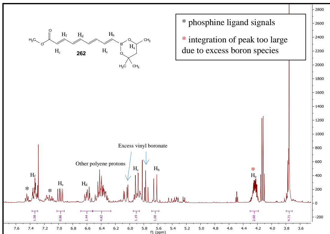
Figure 4 ^1\text{H} NMR spectrum for crude tetraenyl boronate 262
