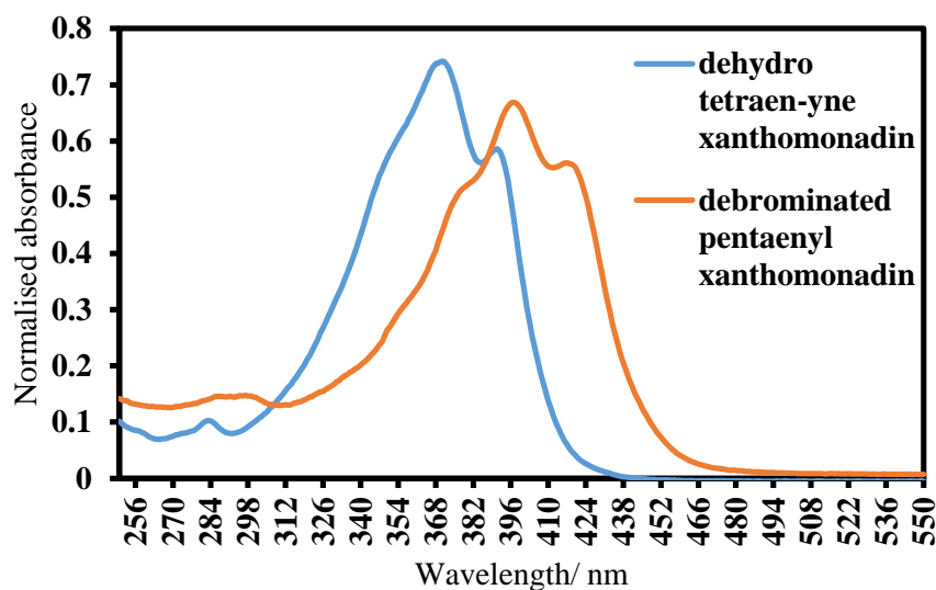
Figure 21 UV-Vis spectra obtained for dehydro tetraen-yne xanthomonadin 235 and debrominated pentaenyl xanthomonadin 234
