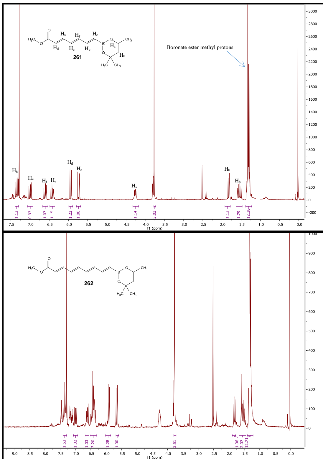
Figure 5 ^1\text{H} NMR spectrum for a ) crude trienyl boronate 261 and b ) crude tetraenyl boronate 262 (see Figure 4 for assignments)
