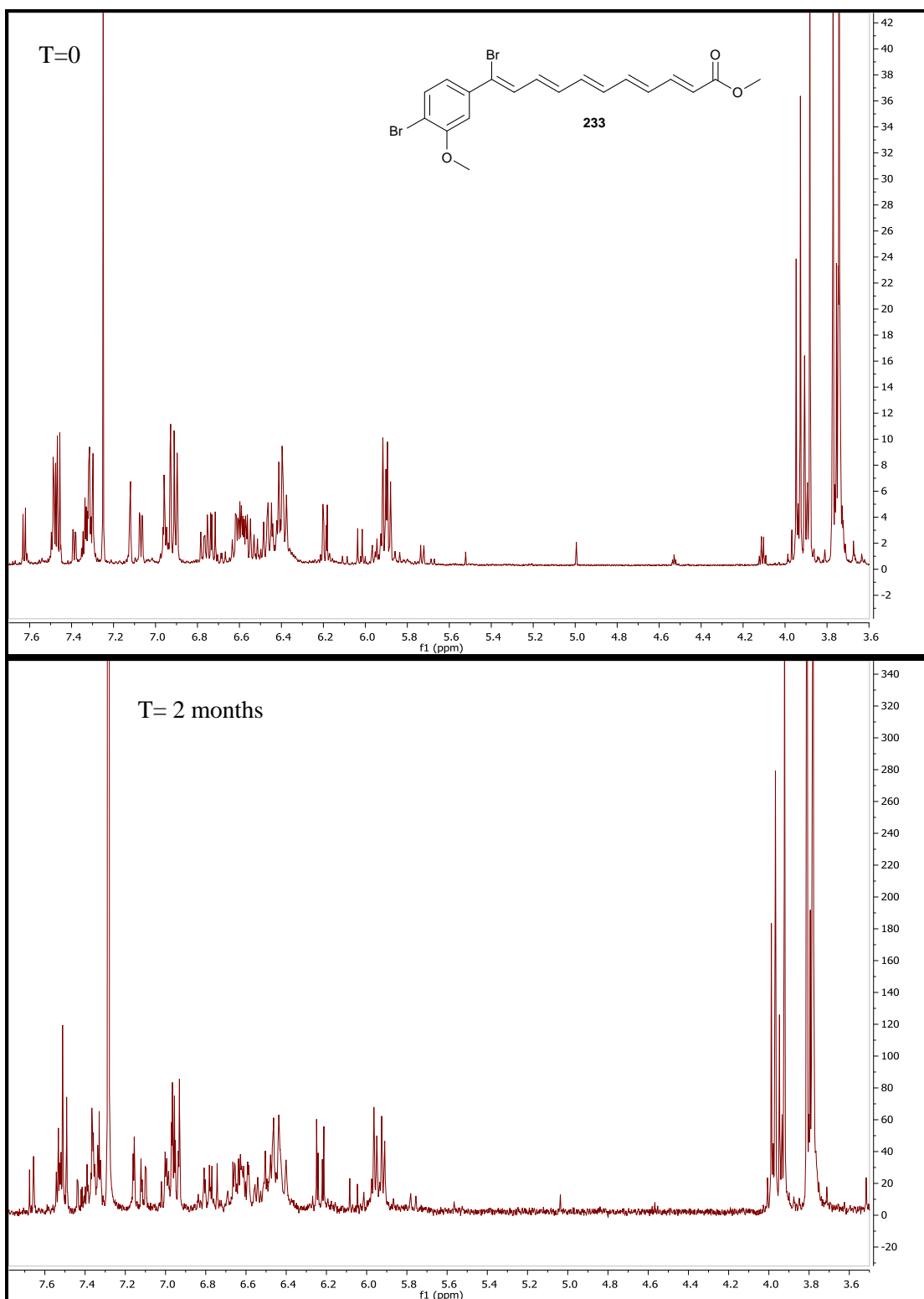
Figure 17 1 H NMR spectra for dibrominated pentaenyl analogue 233 , indicating stability over 2 months
