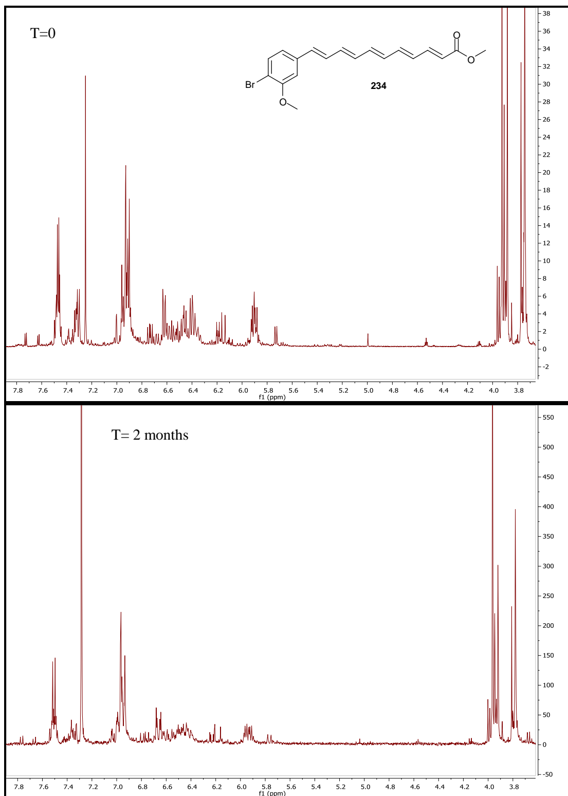
Figure 18 1 H NMR spectrum for debrominated pentaenyl xanthomonadin 234 , indicating stability over 2 months
