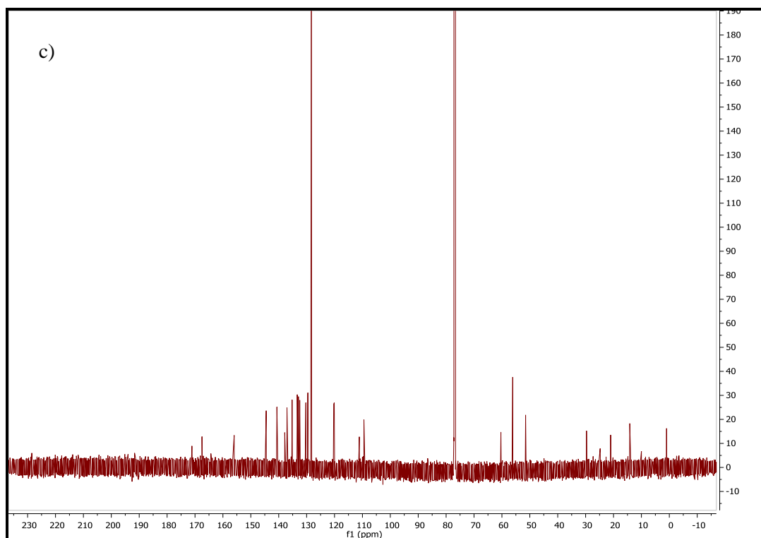
Figure 20a) HSQC 2D NMR b) HMBC 2D NMR and c) ^{13}\text{C} NMR spectra for a sample of debrominated pentaenyl xanthomonadin 234 , isolated using benzene
