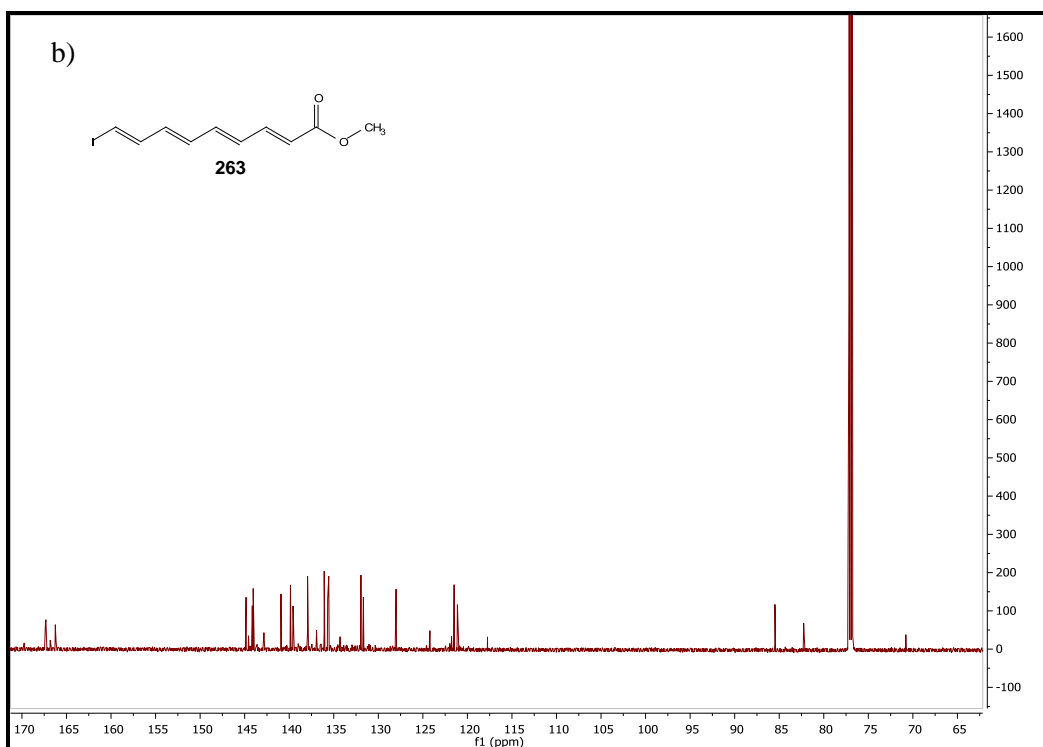
Figure 15a) Stacked ^1\text{H} NMR spectra for tetraenyl iodide 263 , showing change over time and b) ^{13}\text{C} NMR spectrum for tetraenyl iodide 263
