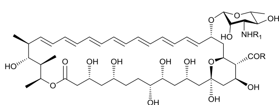
amphotericin B 150 R = OH, R 1 = H
