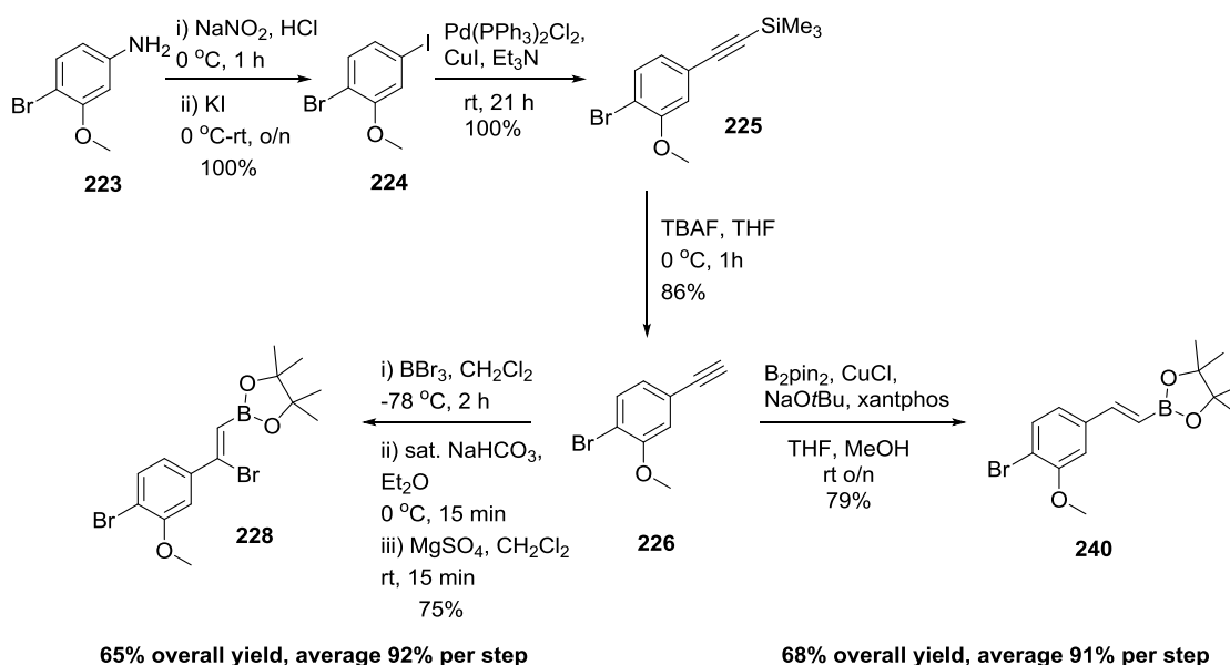
Scheme 39 Current route to key aryl intermediates 226 , 228 and 240
