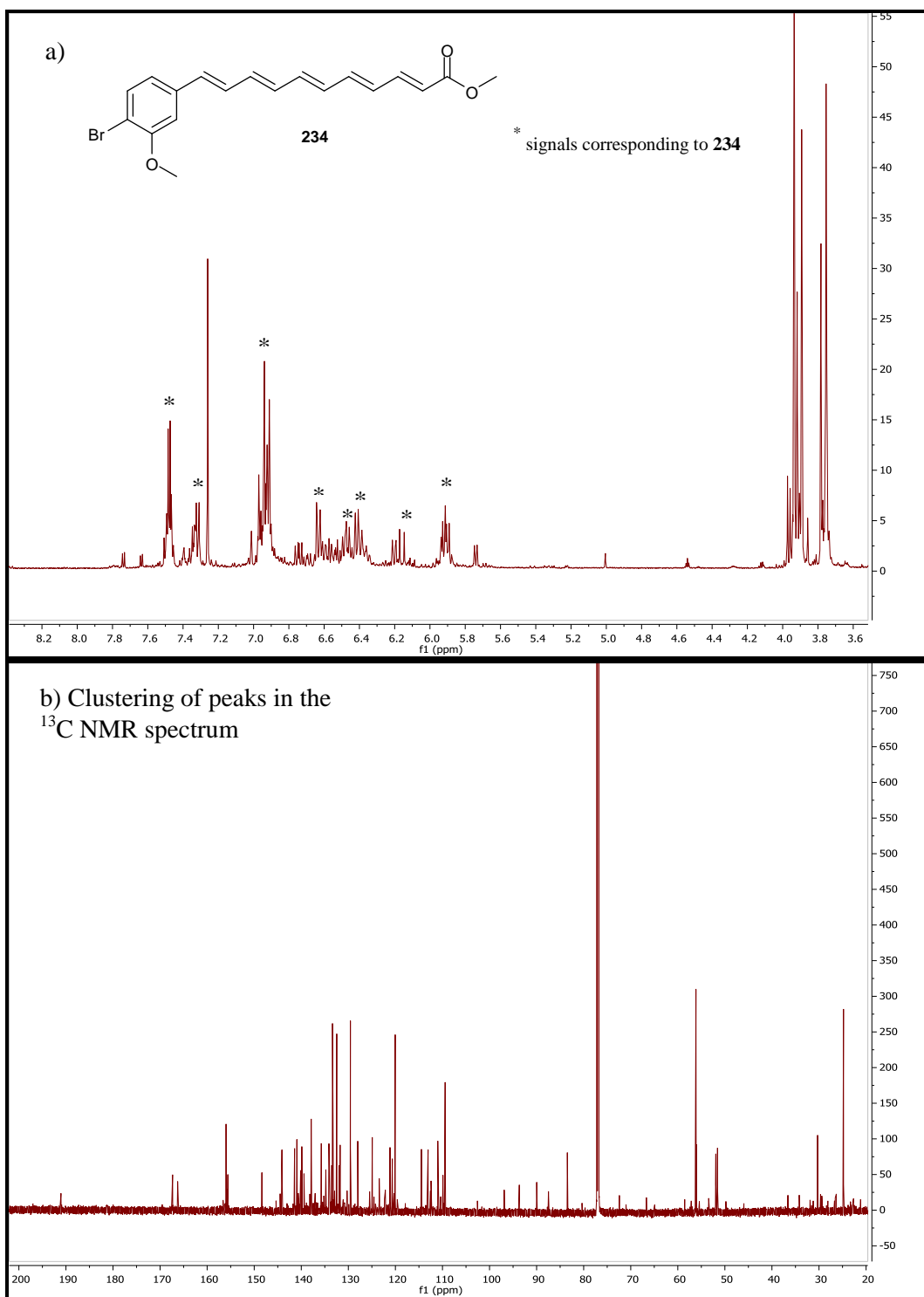
Figure 14a) ^1\text{H} NMR and b) ^{13}\text{C} NMR spectra for debrominated pentaenyl xanthomonadin 234
