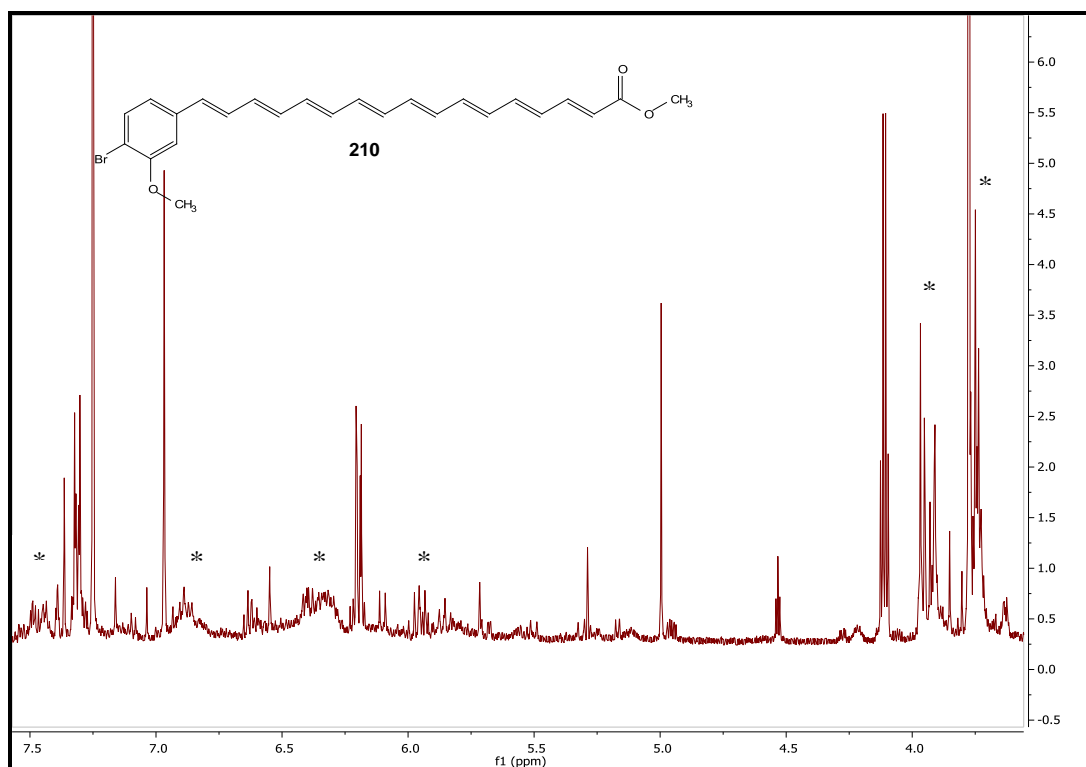
Figure 10 ^1\text{H} NMR spectrum showing the presence of monobrominated xanthomonadin 210
