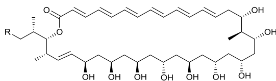
dermostatin A 124 R = H
