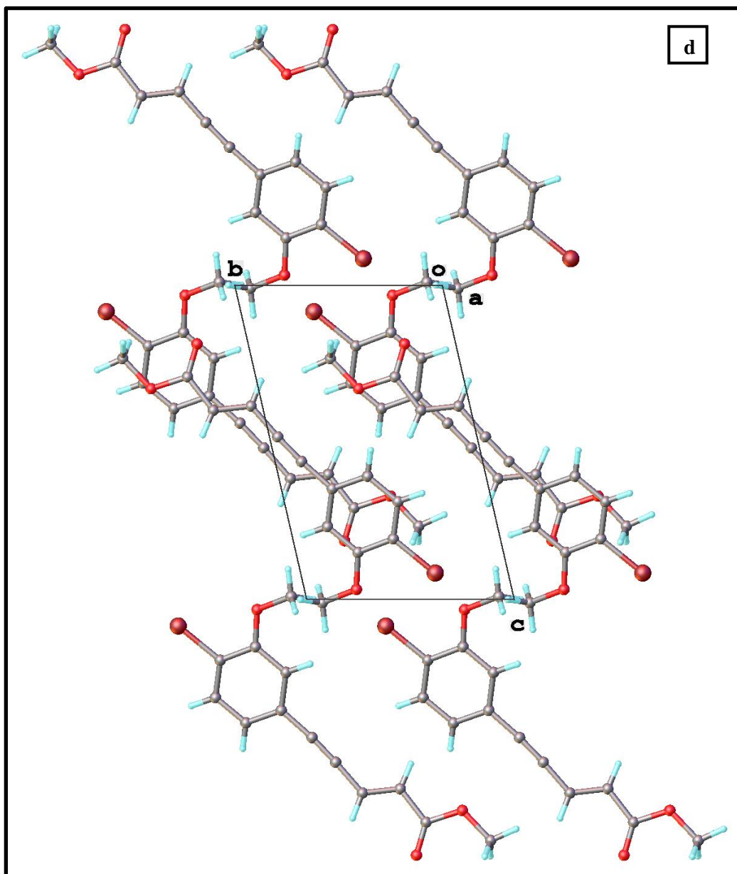
Figure 7 Pictures obtained from X-ray crystallography on analogue 252
