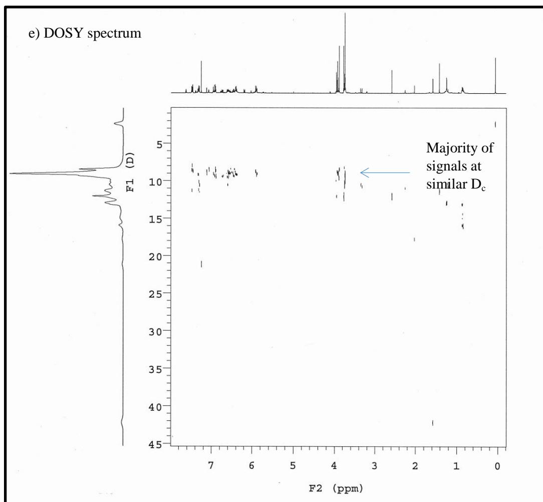
Figure 13a) ^1\text{H} NMR, b) ^{13}\text{C} NMR, c) HMBC 2D NMR, d) HSQC 2D NMR and e) DOSY NMR spectra for dibrominated pentaenyl analogue 233
