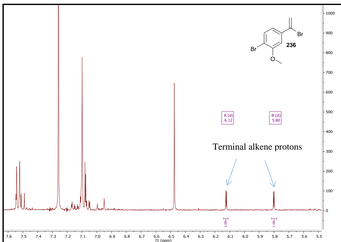
Figure 1 ^1\text{H} NMR spectrum of boronic acid 227 , showing the characteristic peaks of side product 236
