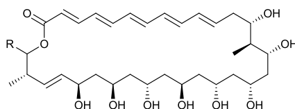
mycoticin A 82 R = i -Pr
