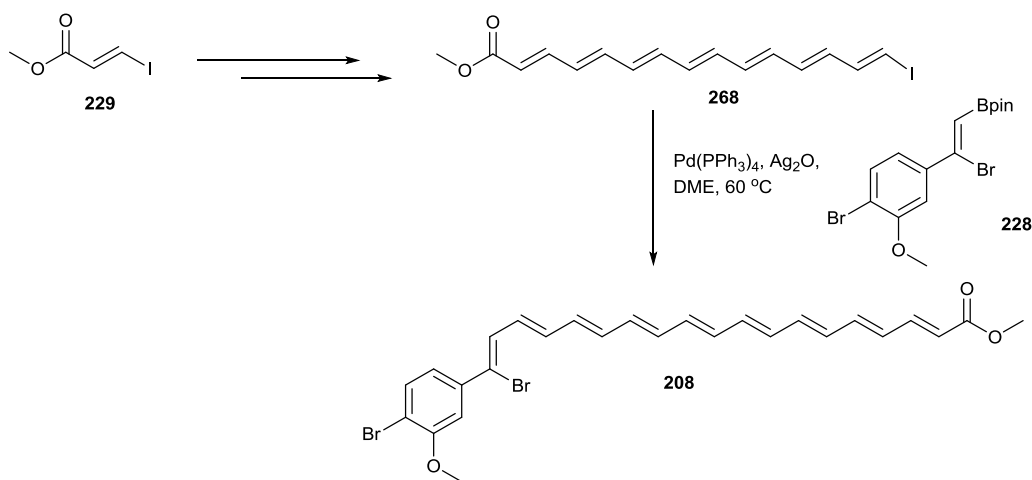
Scheme 58 Attempted synthesis of xanthomonadin 208 using brominated boronate ester 228
