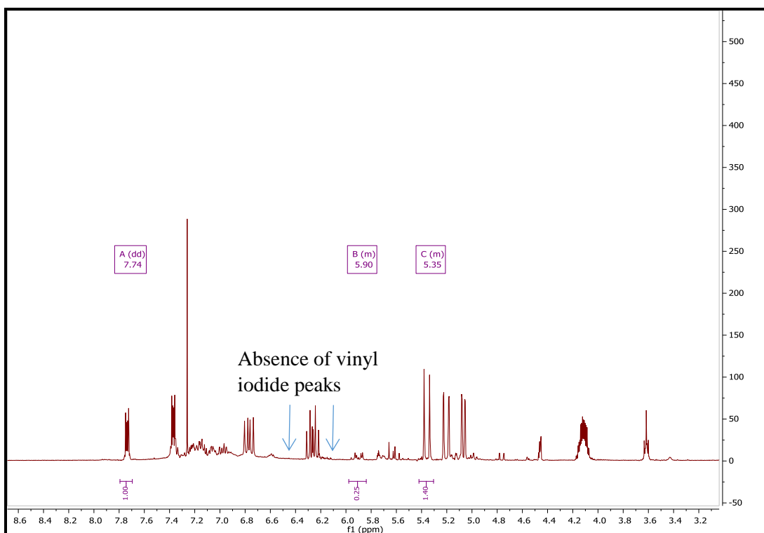
Figure 22 Crude ^1\text{H} NMR spectrum ( Table 16, Entry 7 ) highlighting the consumption of vinyl iodide 269 . Vinyl iodide gives signals of a doublet of doublets at \delta 6.22 ppm and a multiplet between \delta 6.43 and 6.58 ppm.
