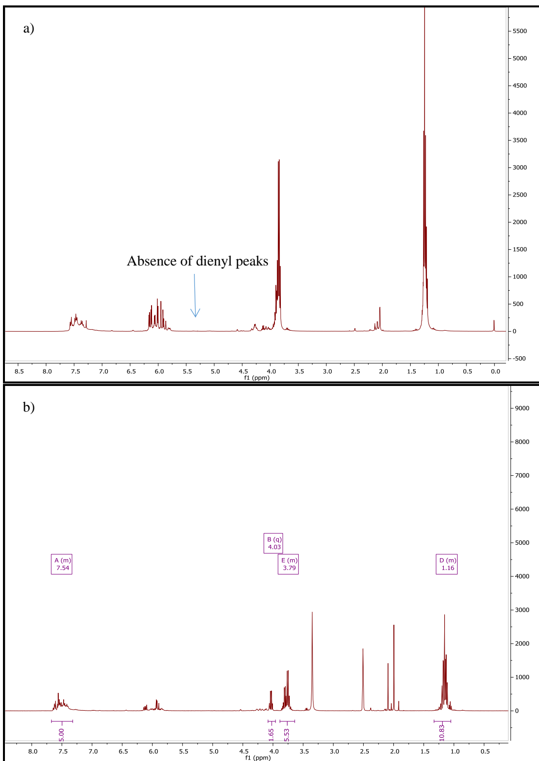
Figure 27 ^1\text{H} NMR spectrum of a) the attempted Diels-Alder cycloaddition, showing complete consumption of diene 316 and b) the precipitate formed during the reaction.
