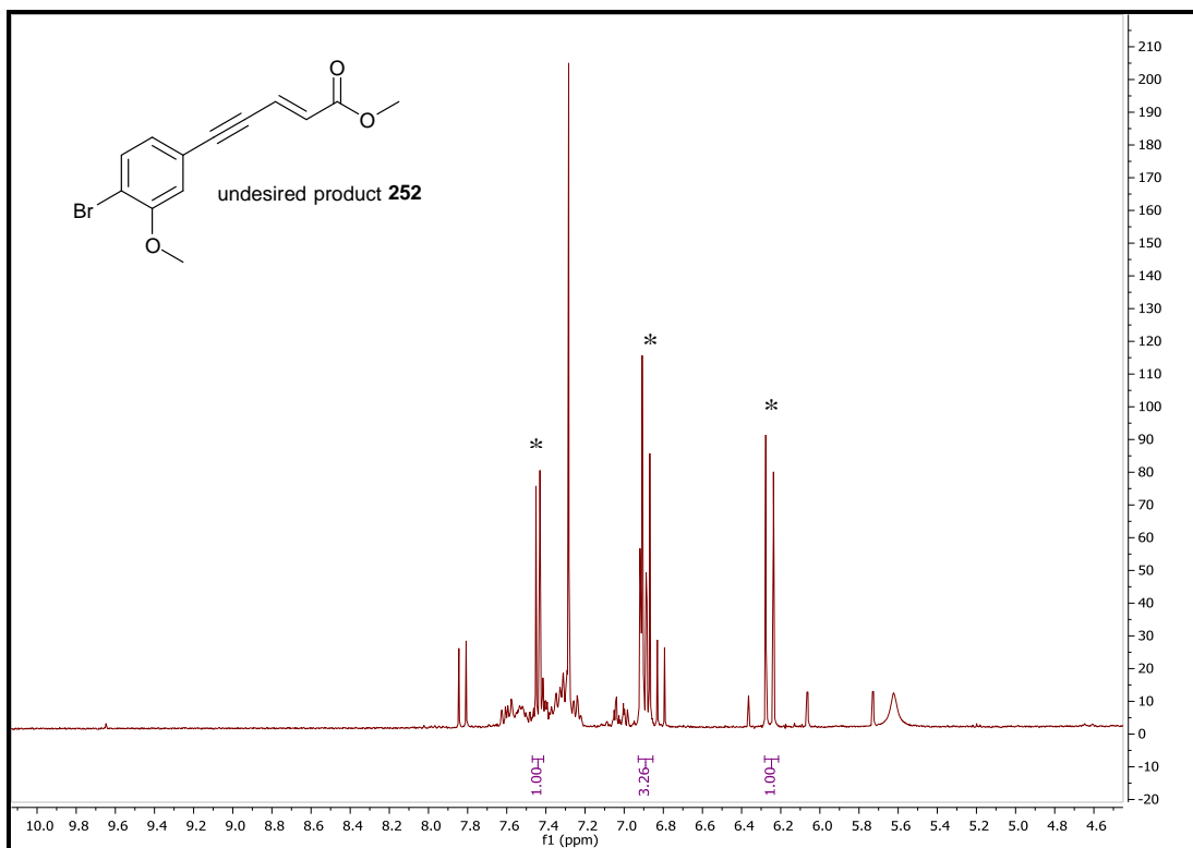
Figure 2 ^1\text{H} NMR spectrum of undesired product 252 formed by subjecting brominated styrenyl Bpin 228 and iodoacrylate 229 to SM conditions, showing that not enough proton signals are present.
