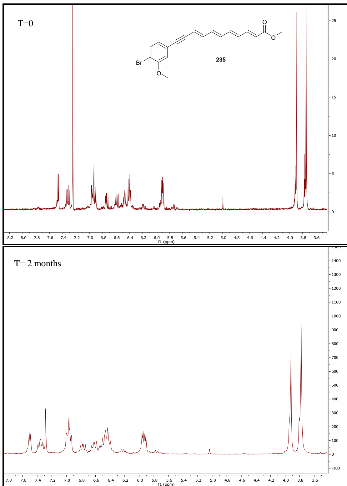
Figure 16 1 H NMR spectra for dehydro-tetraen-yne xanthomonadin 235 , indicating stability over 2 months
