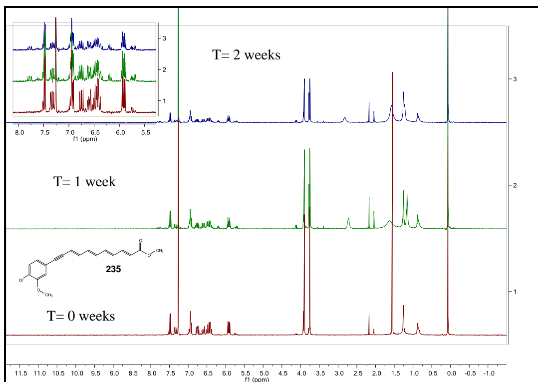
Figure 12 ^1\text{H} NMR spectra showing the change in dehydro tetraen-yne xanthomonadin 235 over a period of 2 weeks.
