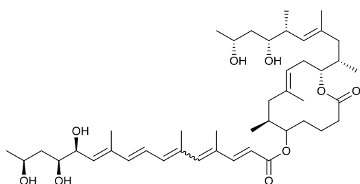
mycolactone A 96 : \Delta 4',5' = Z mycolactone B 97 : \Delta 4',5' = E
