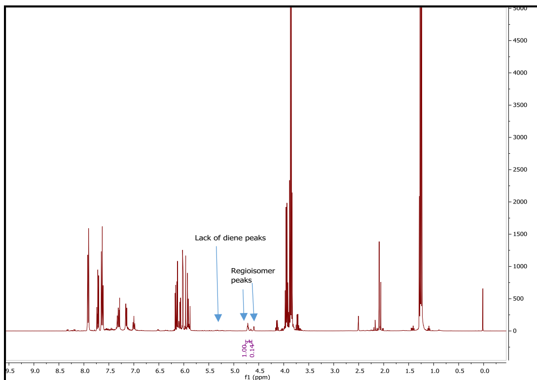
Figure 26 ^1\text{H} NMR of attempted nitrosocycloaddition onto diene silane 316 (Table 22, Entry 1), showing the consumption of diene and the two supposed regioisomers 321 and 322
