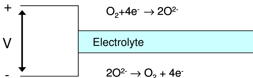
Figure 1.7: Diagram of an oxygen pump. 20
