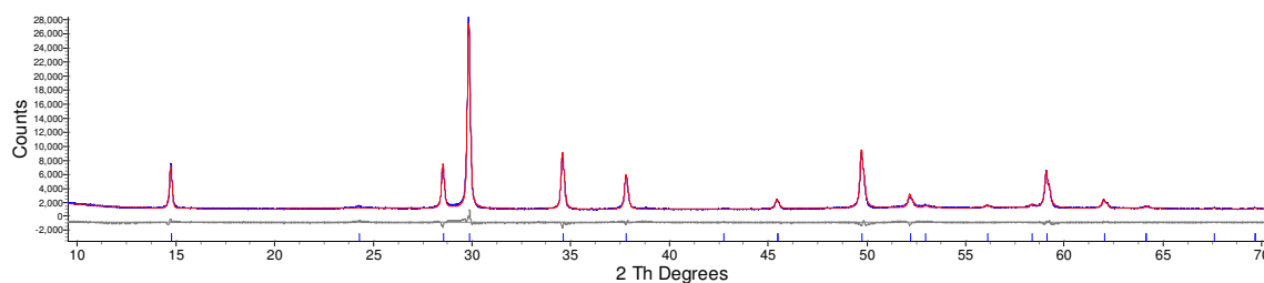
Figure 3.12: d9_03133: Rietveld refinement of \text{Bi}_2\text{Ti}_2\text{O}_7 . R_{\text{wp}} = 4.639\% , a = 10.3579(1) \text{ \AA} .
