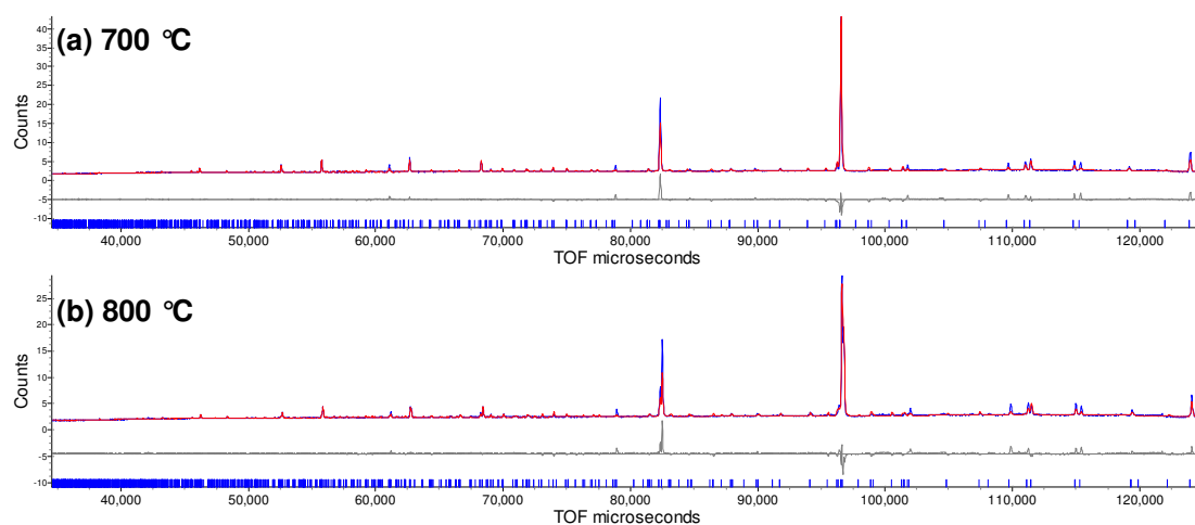
Figure 6.8: Rietveld fit of \text{Bi}_6\text{WO}_{12} at (a) 700 °C, R_{wp} = 4.167\% (b) 800 °C, R_{wp} = 3.779\% .
