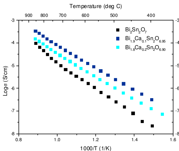
Figure 4.27: Variation of conductivity with temperature for the Bi 2-x Ca x Sn 2 O 7-x/2 system.
