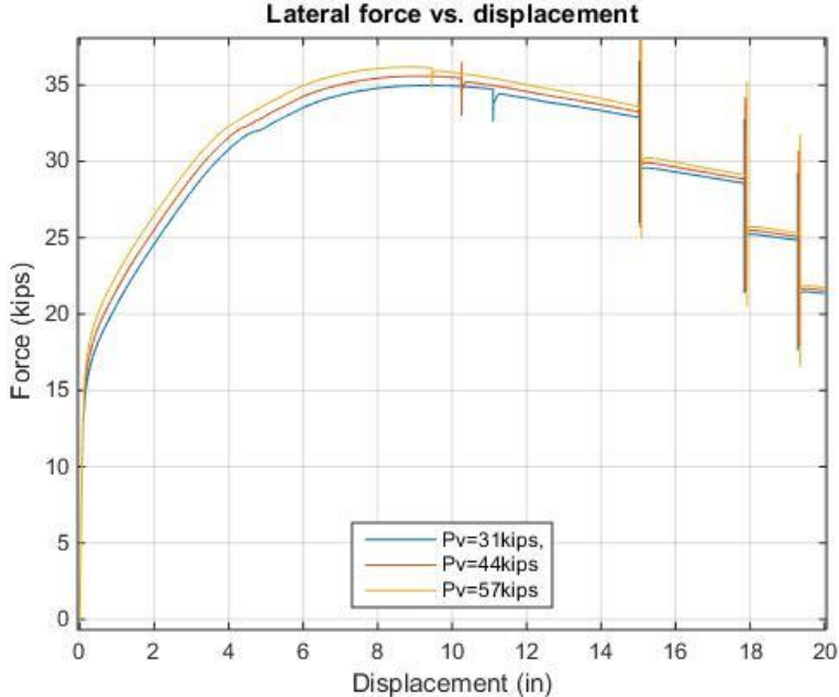
Figure 49 Lateral force vs displacement with varying external loads
