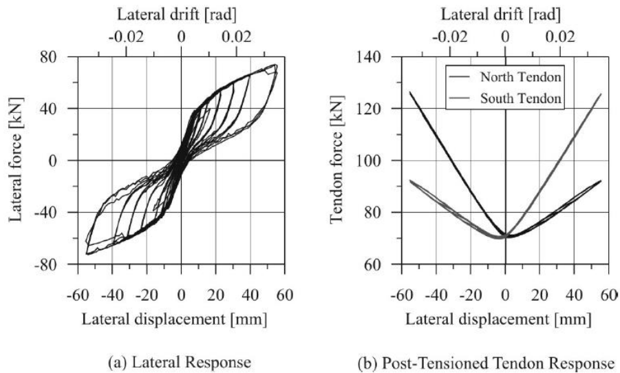
Figure 29. Data from cyclic testing by Marriott et al. (2009)
