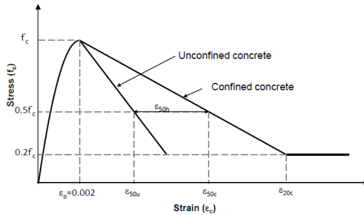
Figure 7 Modified Kent and Park model (Scott et al. 1982)
