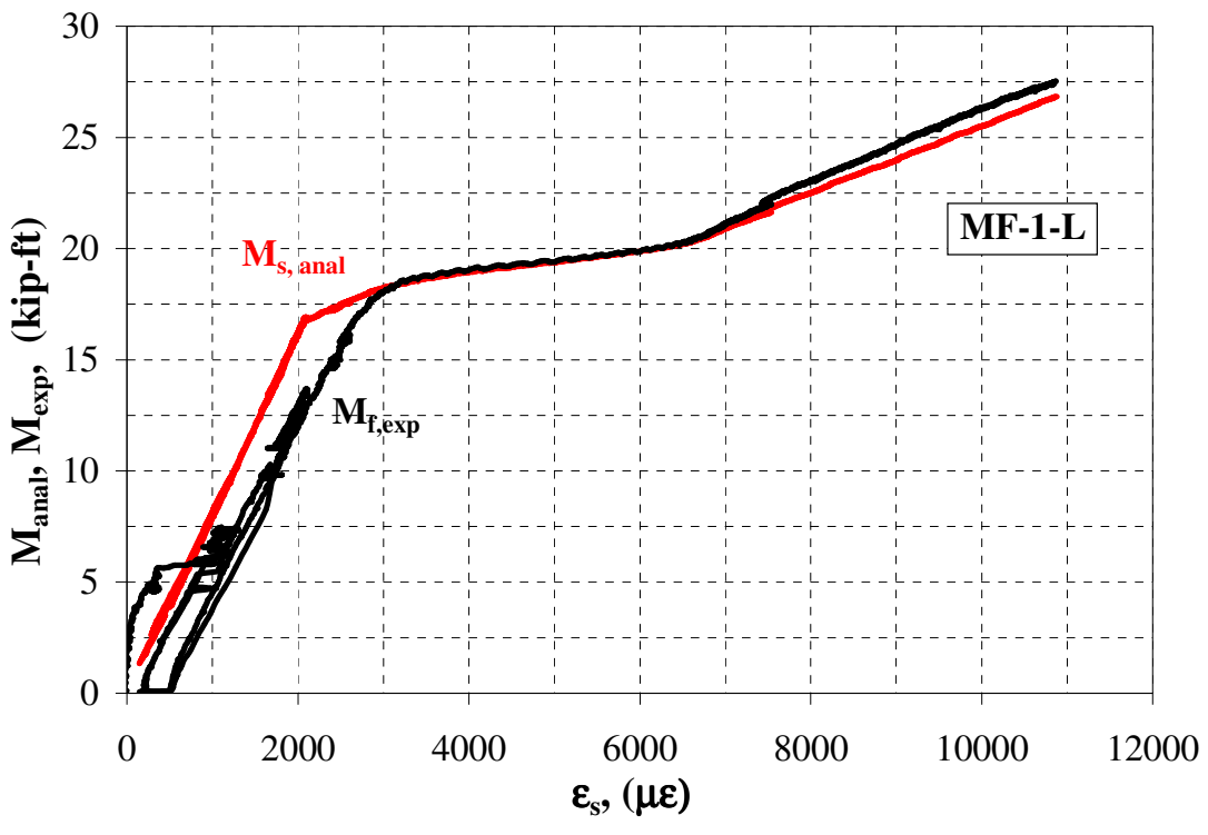
Figure 4.22 – Analytical and experimental moments vs experimental steel strain
