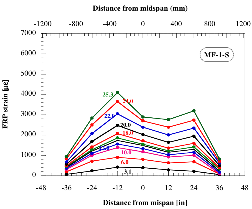
Figure 4.13 – FRP strain profile: slab MF-1-S (Moment in kip-ft: 1 kip-ft=1.356 kN m)
