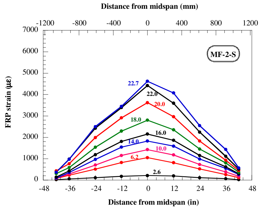
Figure 4.17 – FRP strain profile: slab MF-2-S
