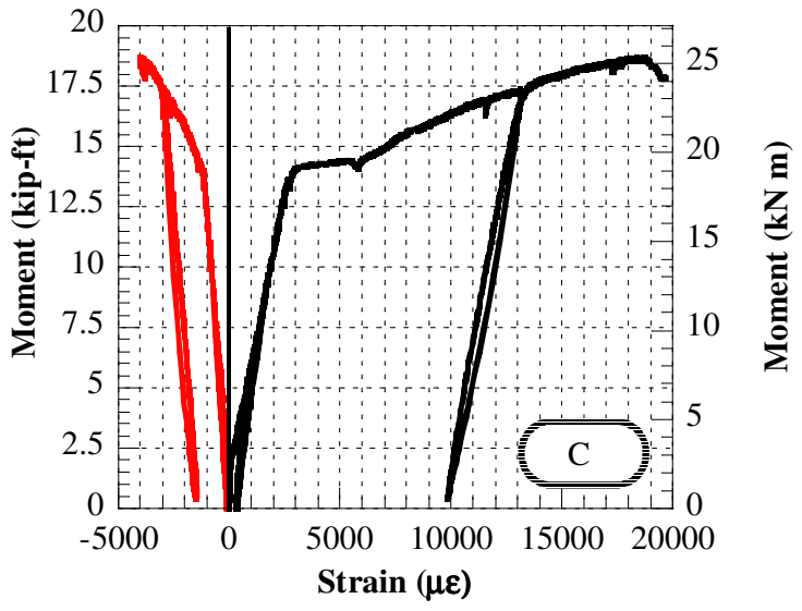
Figure 4.7 – Strain in concrete and steel: slab C
