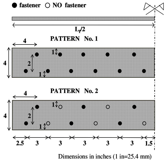
Figure 3.3 – Selected MF FRP fastener layouts
