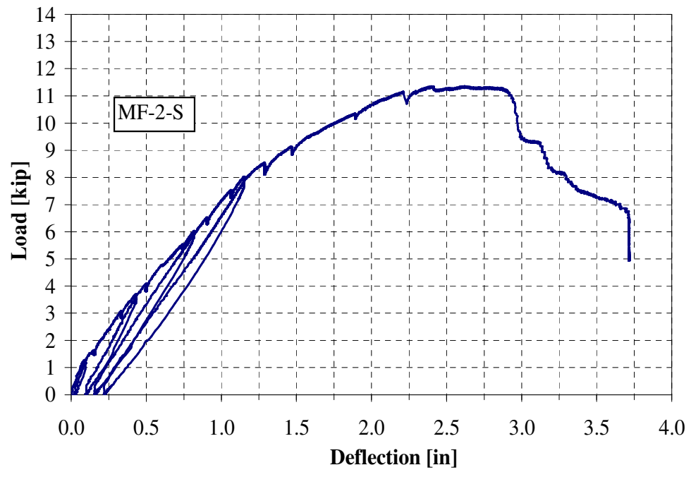
Figure A6 – Load-deflection curve at midspan: slab MF-2-S
