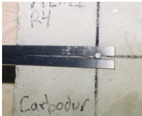
Figure 2.1 – Splitting Failure for existing FRP Laminates (Lamanna 2002)
