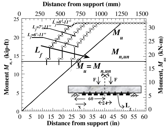
Figure 3.5 – Selection of FRP Laminate length: Pattern No. 1
