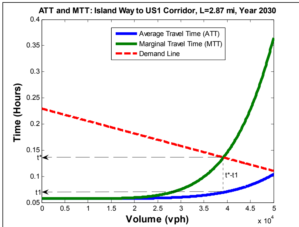
Figure 5.4: 2030 Marginal & Average Travel Time, Demand Function, Equilibrium Points
