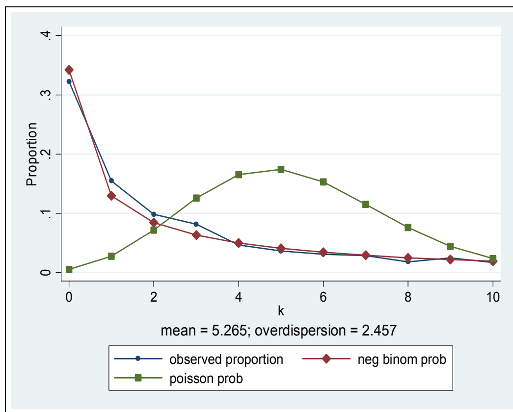
Figure 4.2: Comparison of Observed, Poisson, NB and Overdispersion
