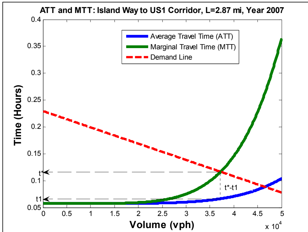
Figure 5.2: 2007 Marginal &amp; Average Travel Time, Demand Function, Equilibrium Points
