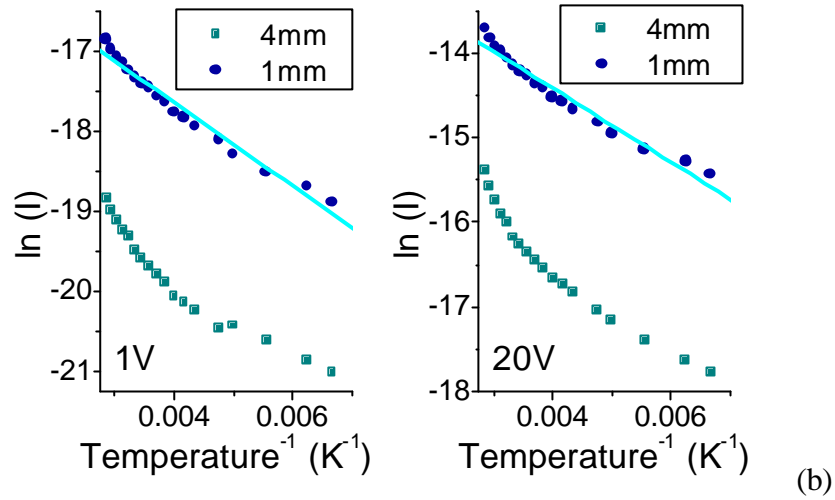
Figure 2-27 (a) \ln\left(I/T^{3/2}\right) versus 1/T plots and (b) \ln(I) versus 1/T plots of the data from the I - T characteristics at 1 and 20 V for electrode separations of 1 and 4 mm
