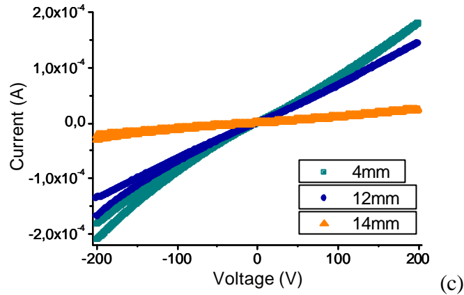
Figure 2-12 In-plane IV characteristics for (a) 5 bi-layers LbL network with electrode separations of 4, 5, 7, 8 and 14 mm. (top) Bias from -200 to +200 V (bottom) bias from -20 to +20 V (b) 10 bi-layers LbL network with electrode separations of 4, 5, 6, 7, 8, 10 and 14 mm (c) 20 bi-layers LbL film with electrode separations of 4, 12 and 14 mm
