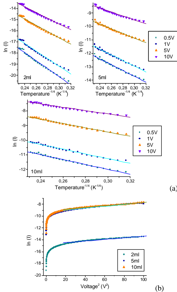
Figure B-5 (a) \ln(I) versus T^{-1/4} plots of the IT plots at 0.5, 1, 5 and 10 V and (b) \ln(I) versus V^2 plots of I - V characteristics for 2, 5 and 10 ml pyridine-SWCNT networks
