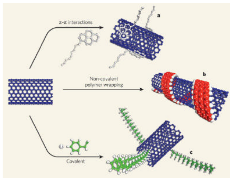
Figure 1-3: Chemical modification of carbon nanotubes. a, Aromatic molecules can be appended to nanotubes using certain non-covalent interactions (known as p - p interactions). b, Non-covalent interactions (including p - p interactions, van der Waals forces and charge-transfer interactions) can be used to wrap polymers around nanotubes. c, Chemical groups can be covalently attached to nanotubes. 52 Reprinted by permission from Macmillan Publishers Ltd: Nature 447, 7148 p.1066, copyright 2007
