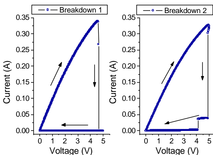
Figure A-9 Typical current breakdowns during I-V measurements at room temperature on 20 bi-layers SWCNT LbL film
