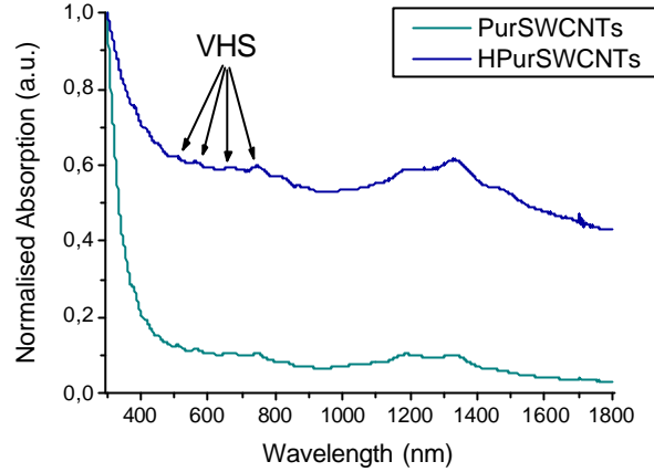
Figure 3-4 Normalised absorption spectra of saturated solutions of purified and purified then annealed SWCNTs in DMF at a nominal concentration of 1:10 mg/ml
