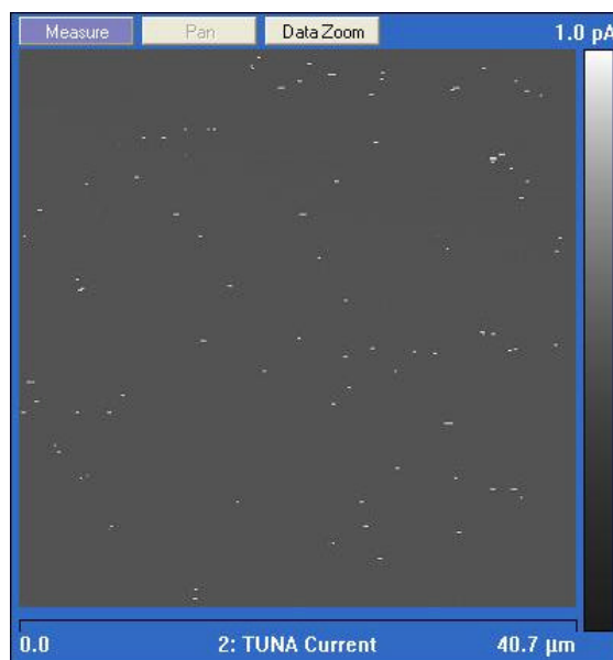
Figure 2-7 Electrical AFM picture of a 5 bi-layers LbL thin film without SWCNTs, 10 V applied
