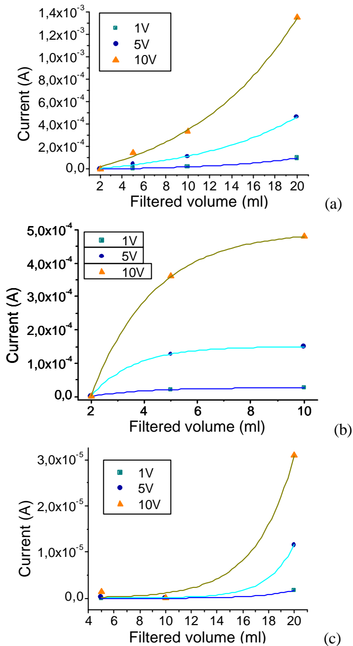
Figure 3-20 Current versus filtered volume plots at 1, 5 and 10 V for (a) idobenzene-SWCNT networks (b) pyridine-SWCNT networks and (c) Sonogashira-SWCNT networks
