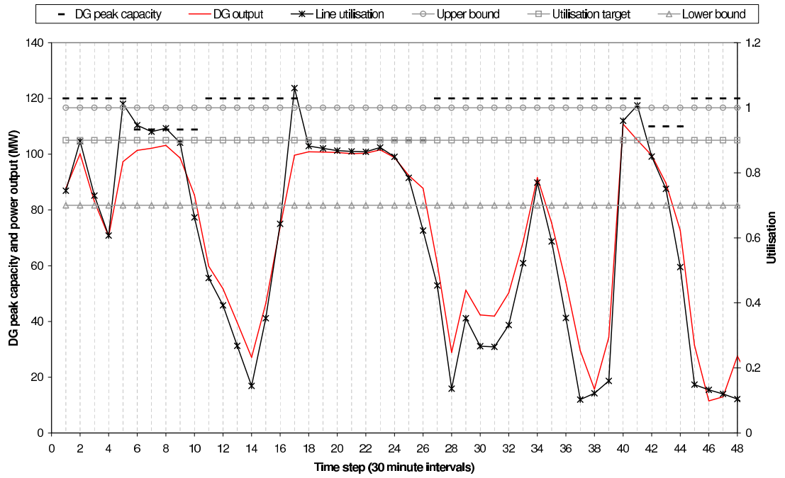
Figure 13.10: Off-line closed loop DG output control
