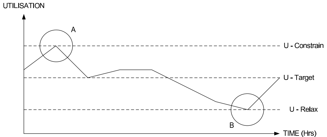
Figure 8.3: Three-rule inference engine
