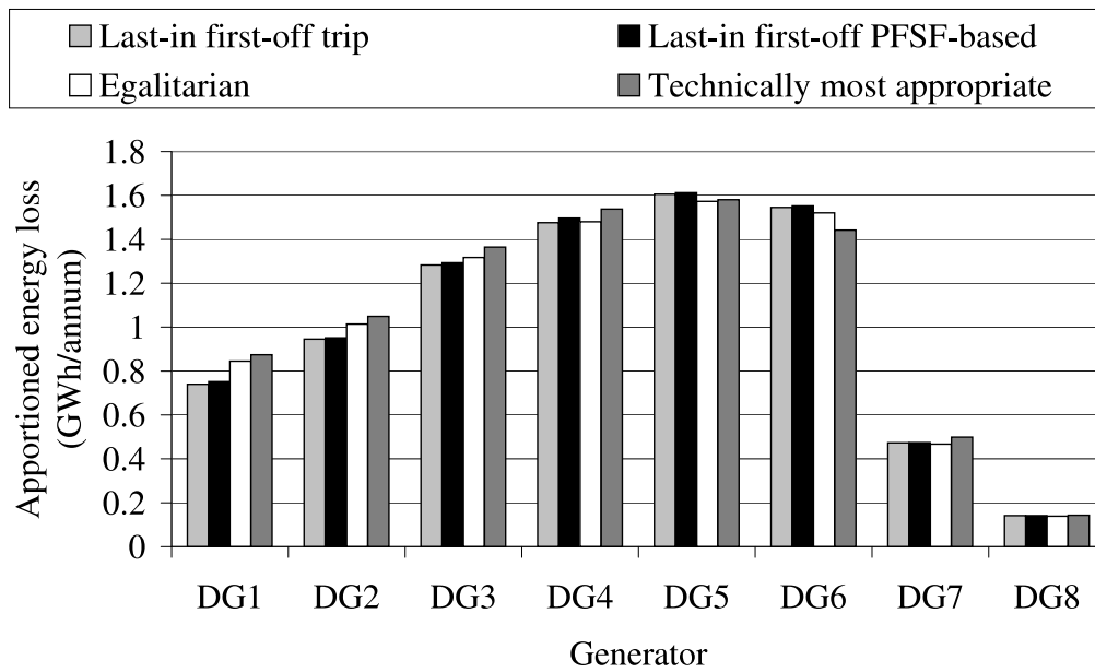
Figure 12.11: DG apportioned annual energy losses resulting from candidate control strategy deployments with component real-time thermal ratings
