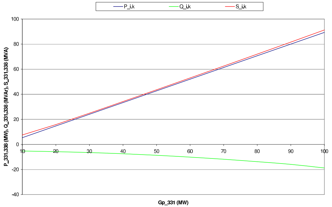
Figure 6.7: Variation of power flows from node 331 to node 338 due to real power injection at node 331 in UKGDS C
