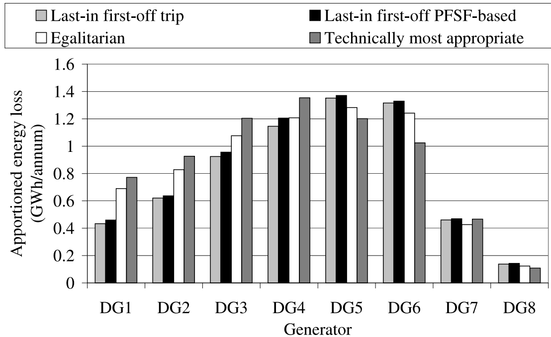
Figure E.6: DG apportioned annual energy losses resulting from candidate control strategy deployments with component seasonal thermal ratings
