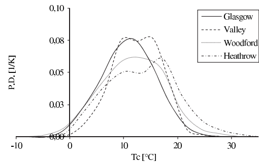
Fig. 4 Air temperature PD
