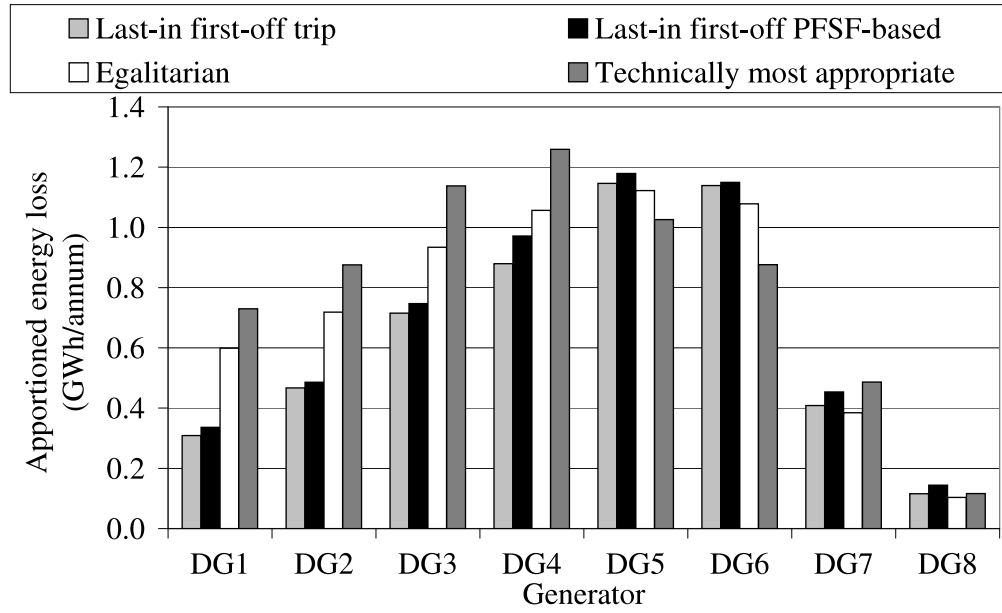
Figure 12.10: DG apportioned annual energy losses resulting from candidate control strategy deployments with component static thermal ratings
