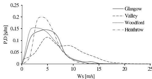
Fig. 3 Wind speed PD
