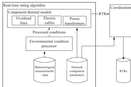
Fig. 2 Simulation scheme
