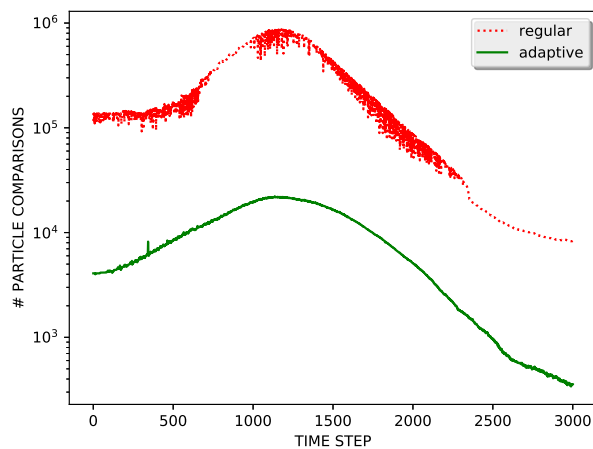
Figure 6.10: Particle comparisons of the hopper (1k particles) flow simulation using regular and adaptive grids. The regular grid make use of more cells/vertices than the adaptive variant and it refined uniformly on the whole domain. The adaptive grid refines only on the areas of particles thus the number of grid vertices is reduced significantly (and grid overhead), this also reduces the number of comparisons required as there are fewer vertices to compare at collisions areas. During the peak of hopper flow particle clustering phase (step 1200), the regular grid performs 850,000 comparisons while the adaptive grid only 25,000, this translates to 34 million versus 1 million triangle comparisons for granulates of 20 triangles for around 2000 actual collision points.
