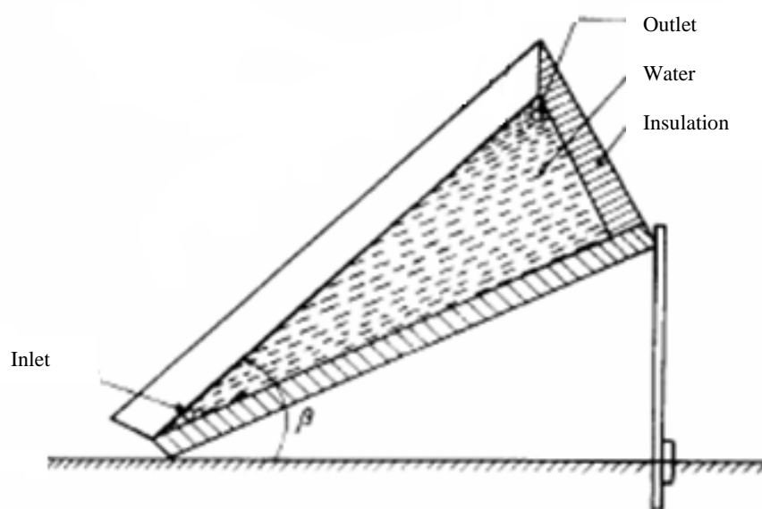
Figure 2.9d A triangular built-in-storage solar water heater [58].
