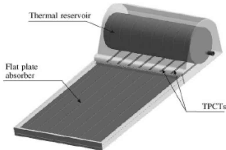
Figure 2.9g TPCT module [61].
