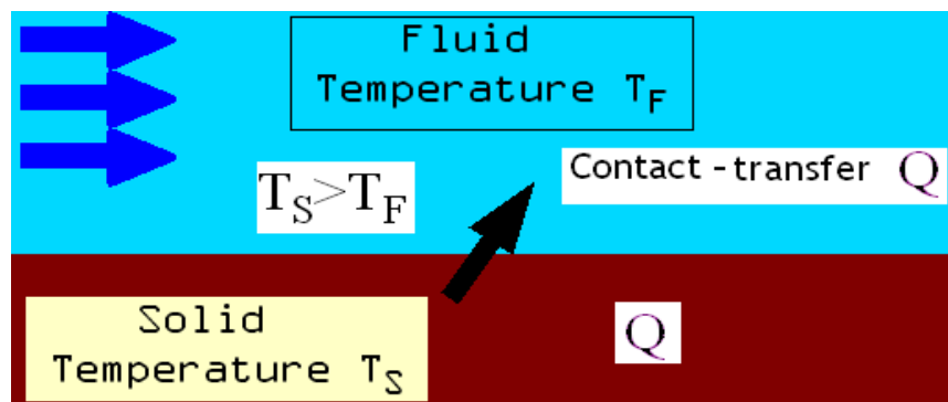
Figure 3.2b Convection heat
