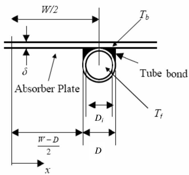
Figure 3.13a Fin and Tube dimensions.
