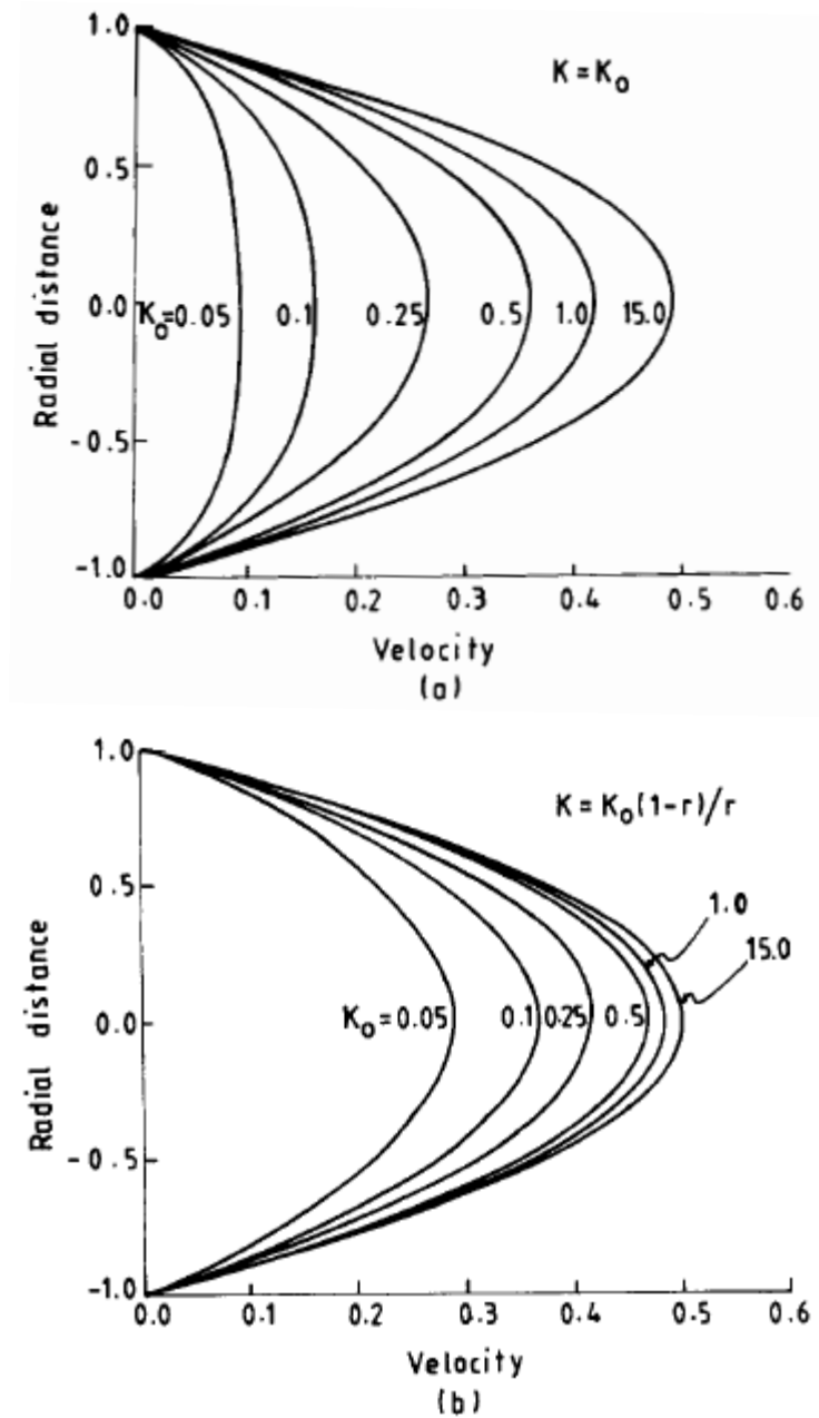
Figure 3.6d Velocity distribution for different values of K_o [79].
