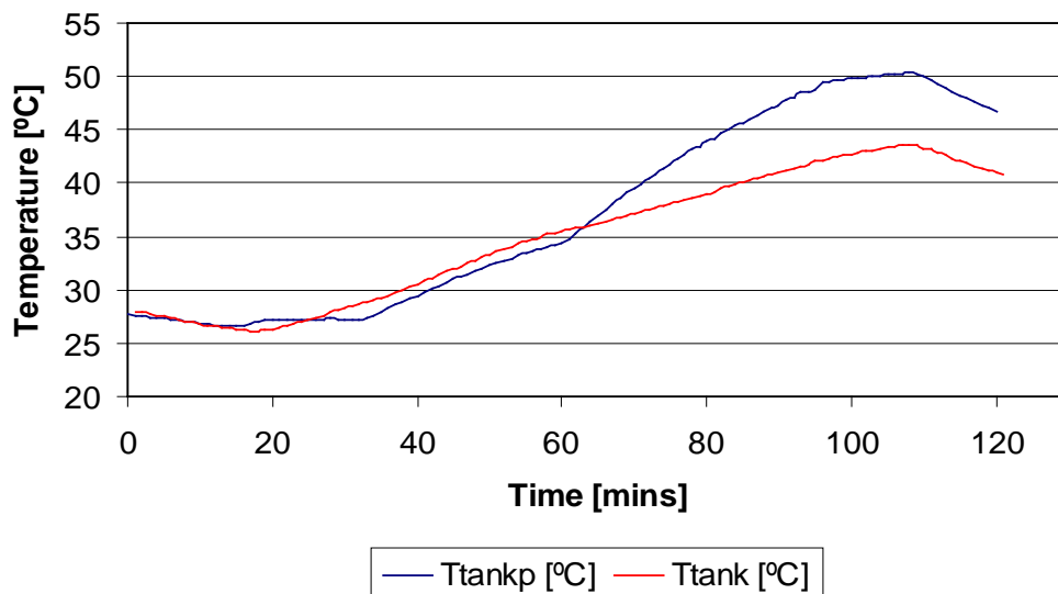
Graph 6.3.1c Temperature versus time in the water jackets.
