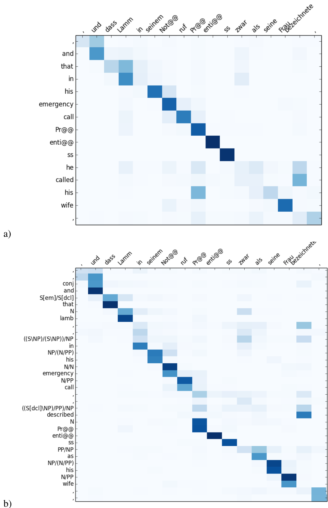
Figure 6.7: Comparison of alignment matrices for a) the baseline NMT system and b) the SNMT system with target syntax. The alignment matrices are cropped and correspond to the subordinate clause in the example b) in Figure 6.5.
