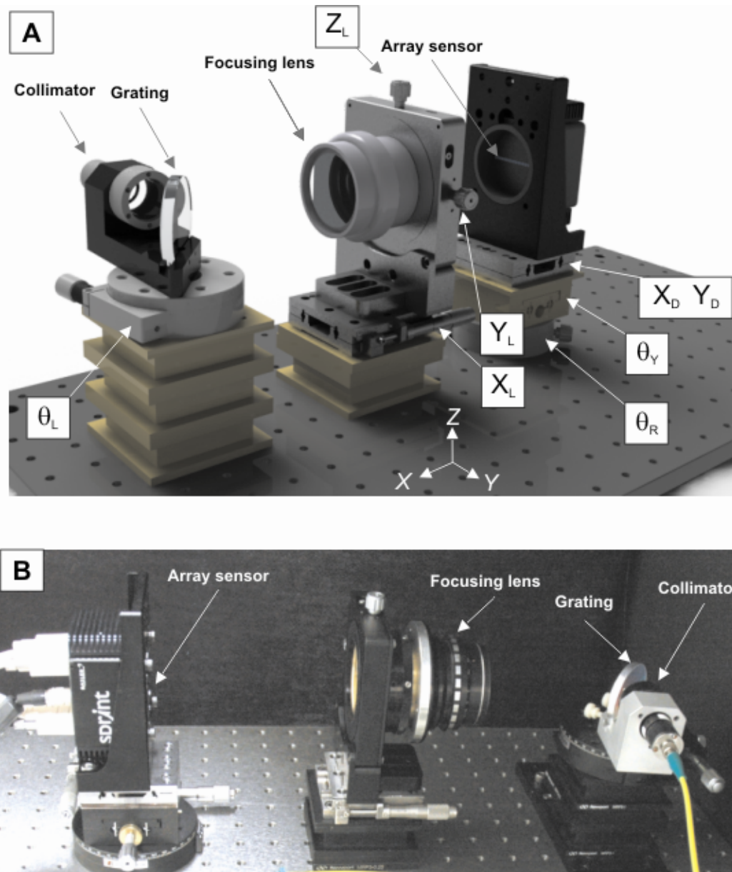
Figure 4.16: (A) Design of the spectrometer with the associated optical components: collimator, grating, lens and array sensor. Three rotation stages adjust for the parameters: \theta_L, \theta_R, \theta_Y while five translation stages adjust for the parameters: X_L, Y_L, Z_L, X_D, Y_D . (B) Photograph of the spectrometer setup.
