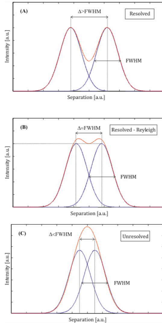
Figure 3.6: Large separation between the Gaussian lineshapes (blue lines). The peaks are resolved (red line) (A) . Rayleigh condition. The separation between the Gaussian lineshapes (blue lines) is equal to their FWHM. The peak are resolved (red line) (B) . The separation between the Gaussian lineshapes (blue lines) is smaller than their FWHM. The peaks are not resolved (red line) (C) .
