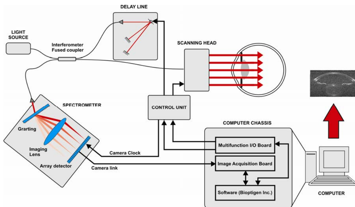
Figure 4.26: Configuration and connections of the SD-OCT system.
