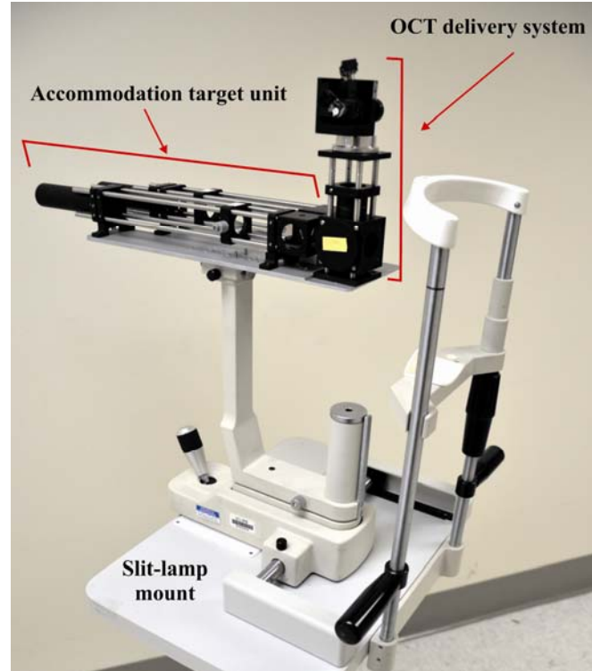
Figure 5.16: Photograph of the accommodation target unit coupled to the OCT delivery system and mounted on a slit-lamp stand.
