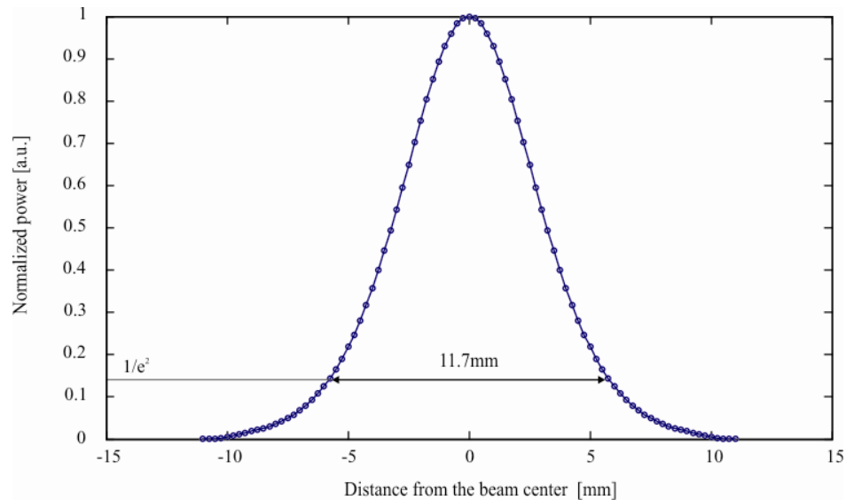
Figure 4.18: Measured intensity distribution of the collimator beam along a horizontal axis.
