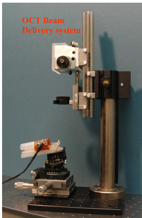
Figure.16. The beam delivery system of OCT and the heated cylindrical holder mounted on 6-axis positioner. (Uhlhorn SR, Borja D, Manns F, Parel JM. Vision Research 2008; 48:2732-2738)
