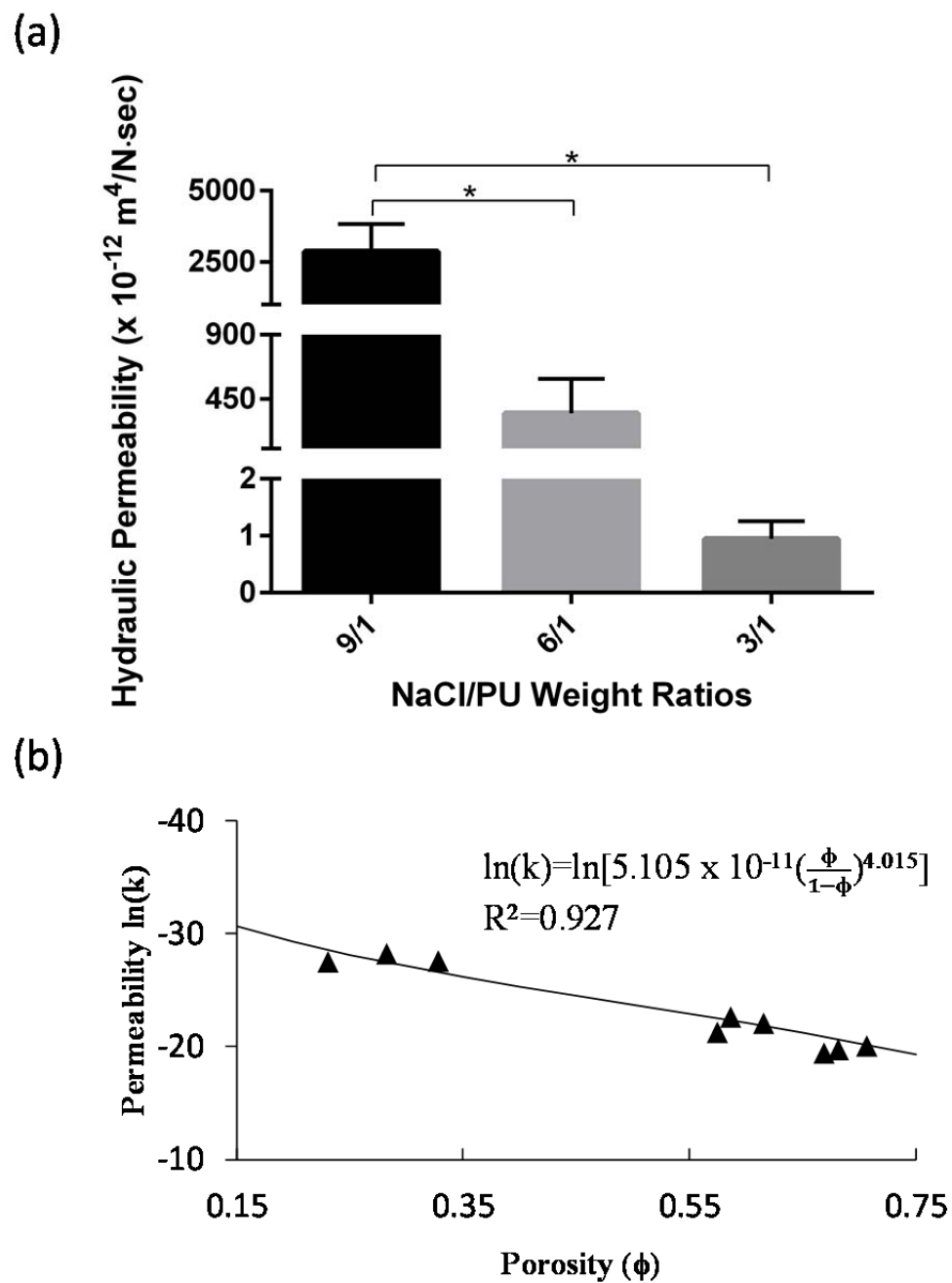
Figure 3-6. (a) The hydraulic permeability of the PU scaffolds with different NaCl/PU ratios fabricated using 25% PU. (b) The relationship between the porosity and hydraulic permeability of the PU scaffolds. (* indicate p-values < 0.05)
