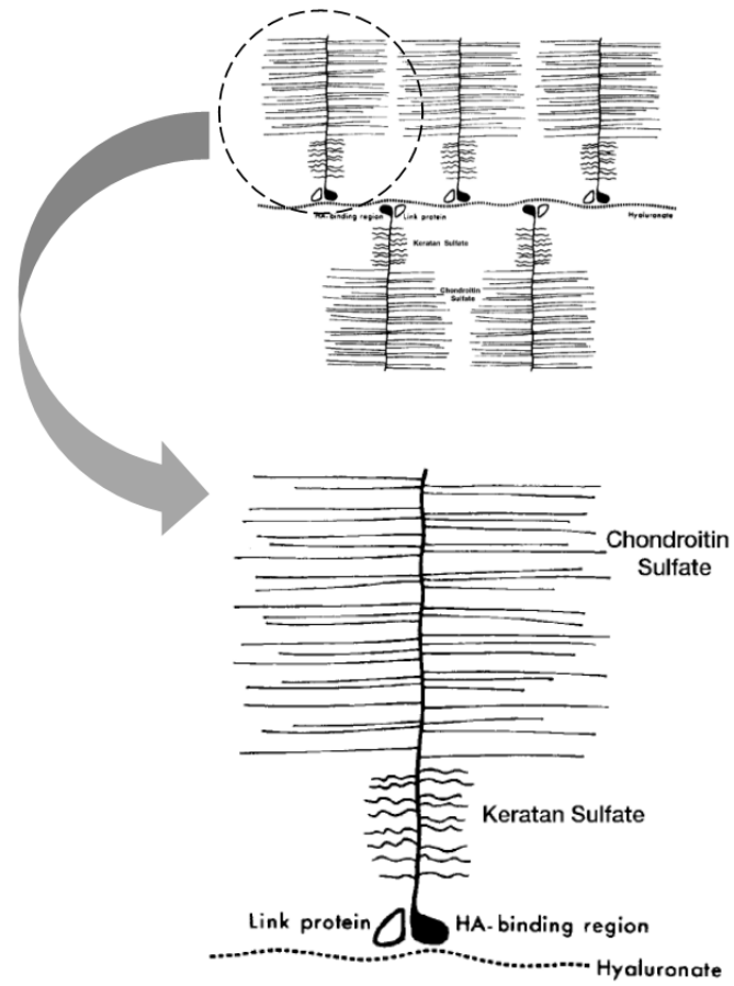
Figure 2-2. Schematic view of a proteoglycan unit. [39]
