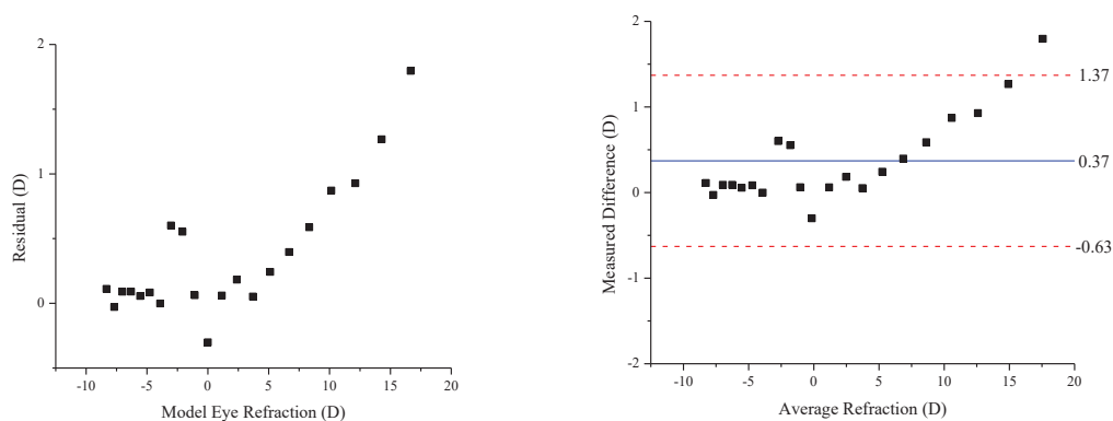
Figure 3.24: (Left) Residuals plot of the linear regression shown in Figure 3.23. Measured values are within \pm 1.8 D of the regression. (Right) Bland-Altman plot of the model eye refraction measurements.
