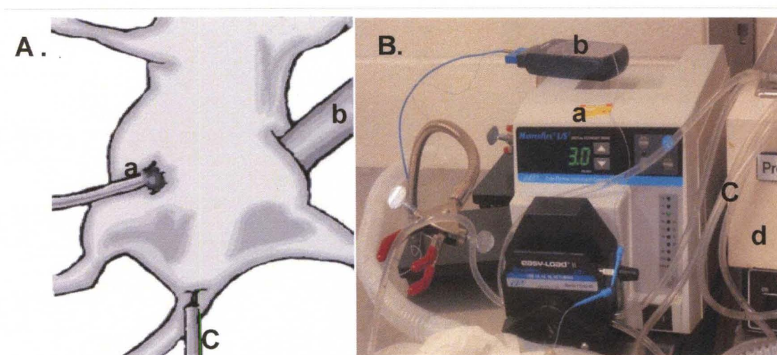
Figure 15. Murine hyperthermic intraperitoneal chemotherapy model. A. Drawing of tumor bearing mouse undergoing HIPEC. Depicted are inlet (a) and outlet (b) ports and anal temperature probe (c) to monitor internal temperature of mouse during perfusion. B. Photograph showing perfusion pump (a), temperature monitor (b), flow tubes (c) and heating bath (d). Mice were perfused for 1 h at the rate of 3 mL/min with cisplatin (3 mg/kg) \pm sodium arsenite (26 mg/kg) at 37 or 43 °C.
