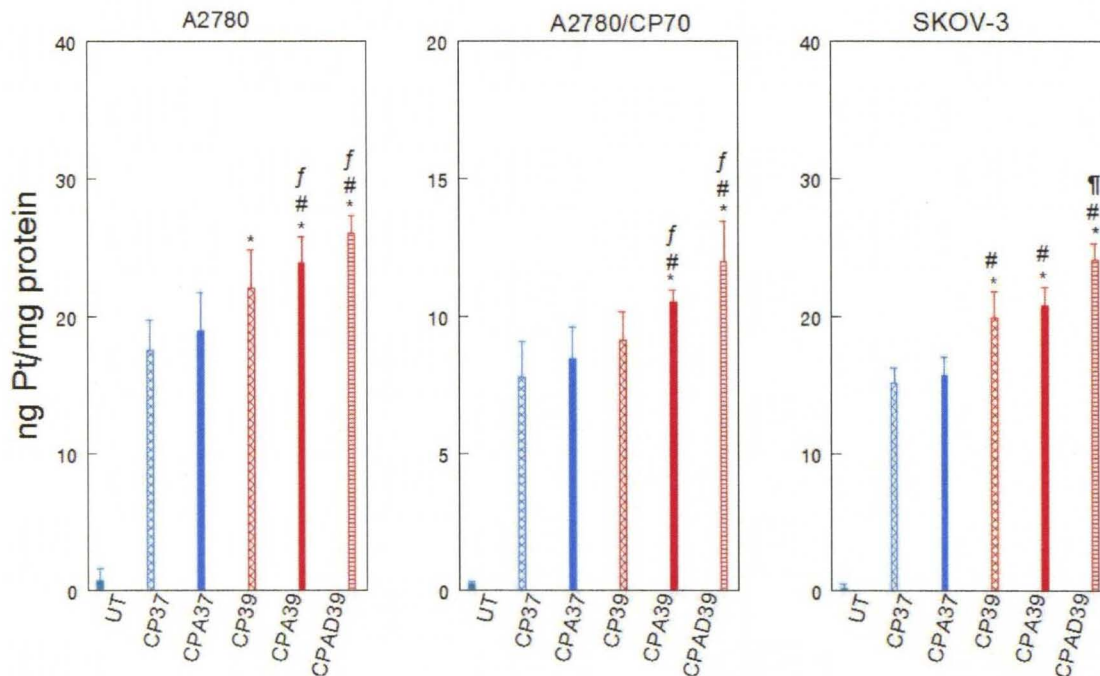
Figure 31. ICP- MS analysis of cellular platinum accumulation. A2780, A2780/CP70 and SKOV-3 cells were treated with 40 \mu M cisplatin (CP37 and CP39)) \pm 20 \mu M sodium arsenite (CPA37 and CPA39) and/or 100 nM of 17-DMAG (CPAD39) at 37 or 39 ^{\circ} C for 1h. Cells were harvested immediately after treatment for total cellular platinum determination. Data are means \pm SD from 3 independent experiments. N = 3, P<0.05. * compared with CP37, # compared with CPA37, f compared with CP39 and ¶ compared with CPA39.
