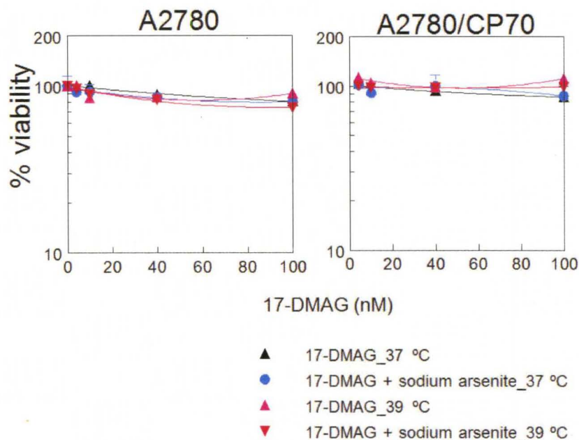
Figure 29. Cell viability effect of 17-DMAG on sodium arsenite \pm
