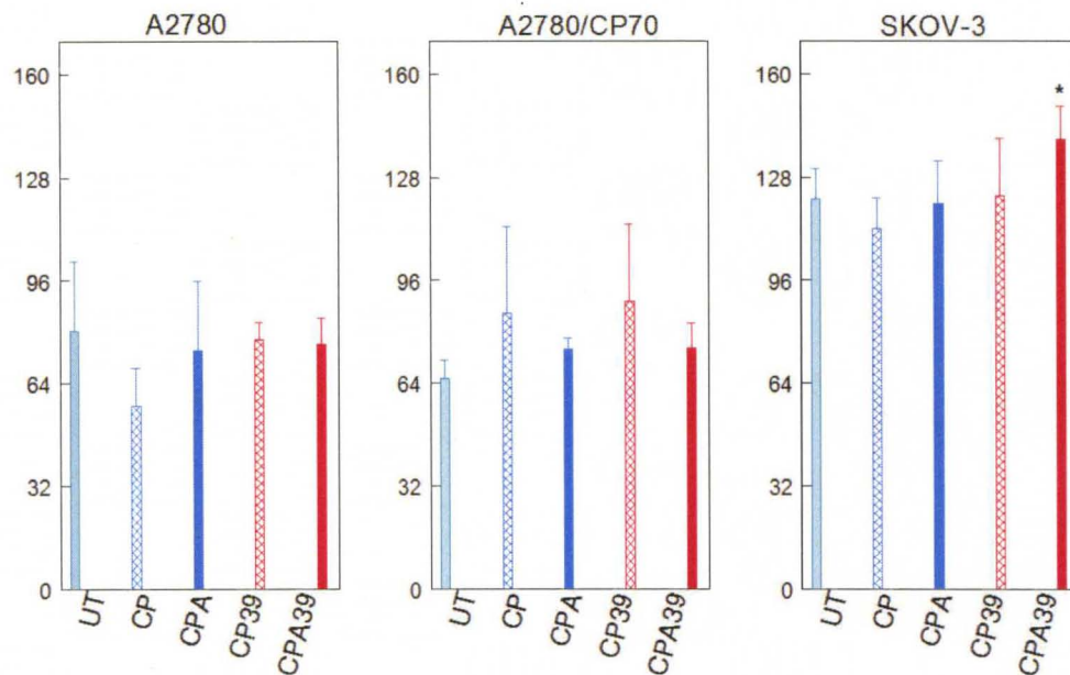
Figure 11. Total GST activity determination. A2780, A2780/CP70 and SKOV-3 cells were treated with 40 \mu M cisplatin (CP) or CP plus 20 \mu M sodium arsenite (CPA) at 37 ^{\circ} C (CP or CPA) or 39 ^{\circ} C (CP39 or CPA39) for 1 h. Cells were harvested immediately after treatment for total GST activity determination. Data are means \pm SD from triplicate biological experiments. P < 0.05 . * compared to untreated cells (UT).
