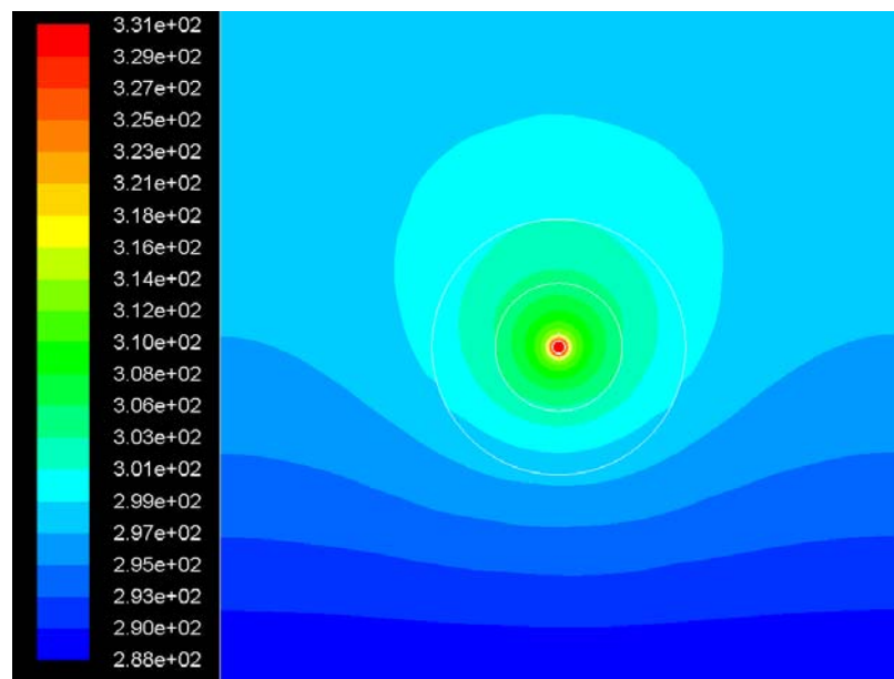
Fig. 8.25d The temperature (K) distribution in and around the underground cable surrounded by the soil domain with the high moisture content
