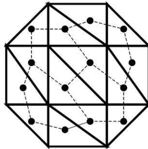
Figure 2-10 Dual Graph
