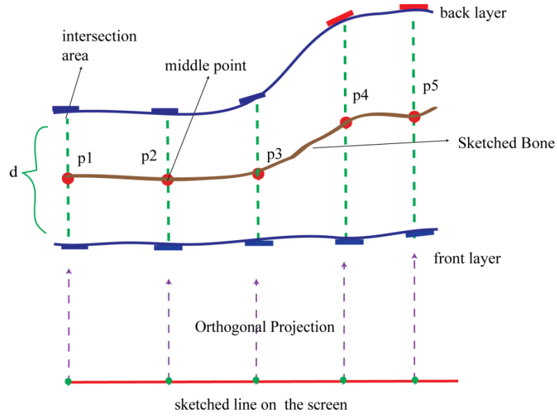
Figure 4-4 Projection Optimization
