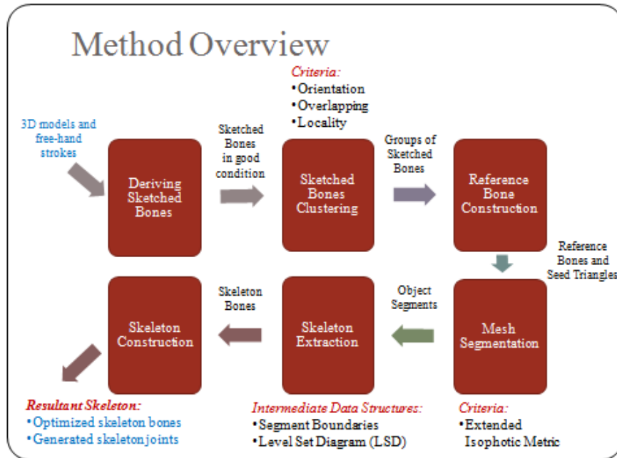
Figure 3-1 Method Overview
