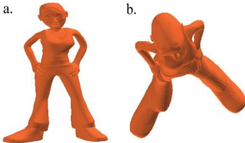
Figure 4-5 Viewpoint Examples
