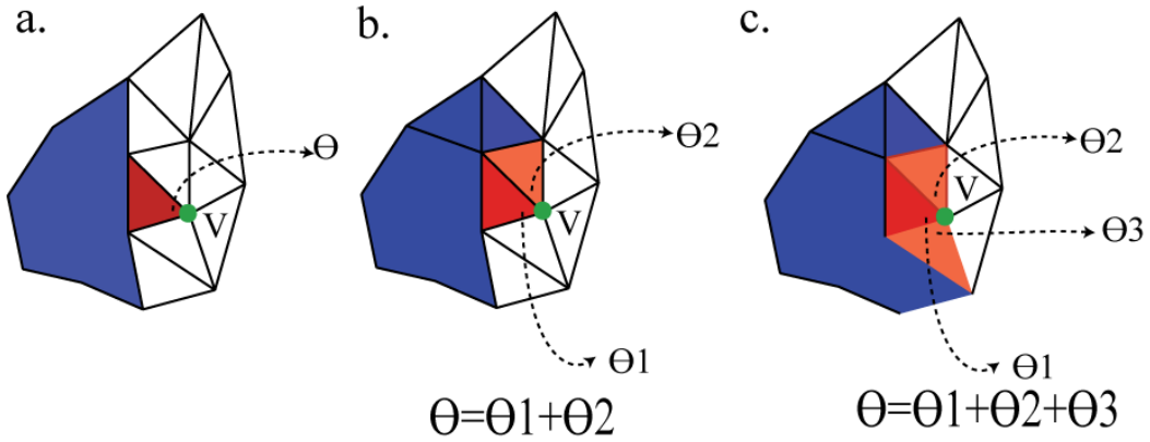
Figure 5-11 Local Boundary Curvature Check
