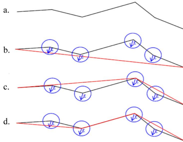
Figure 4-7 Douglas-Peucker Algorithm Procedures [97]
