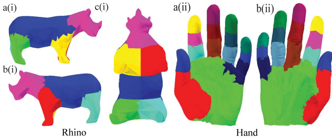
Figure 5-5 Level 1 - Segmentation Results for Simple Mesh Models
