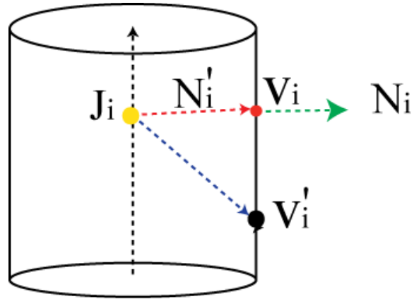
Figure 6-19 Concept of Bone Evaluation
