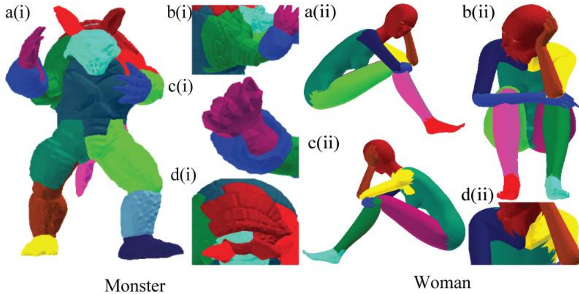
Figure 5-7 Level 3 – Segmentation Results for Complex Models
