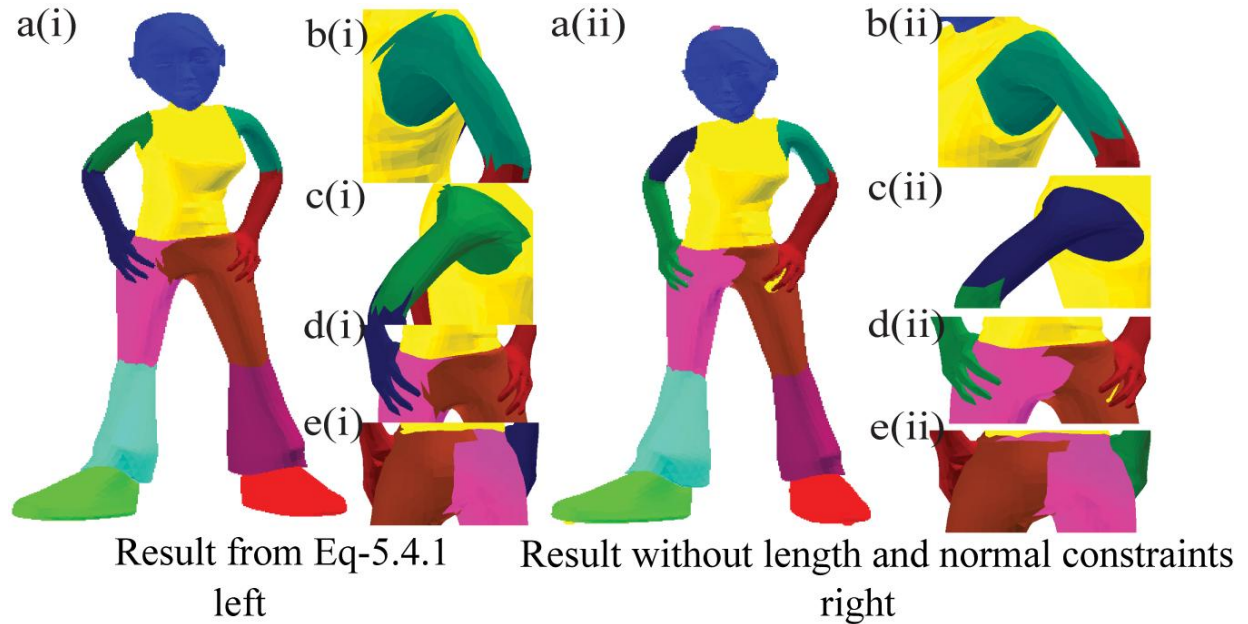
Figure 5-8 Importance of Length and Normal Constraints
