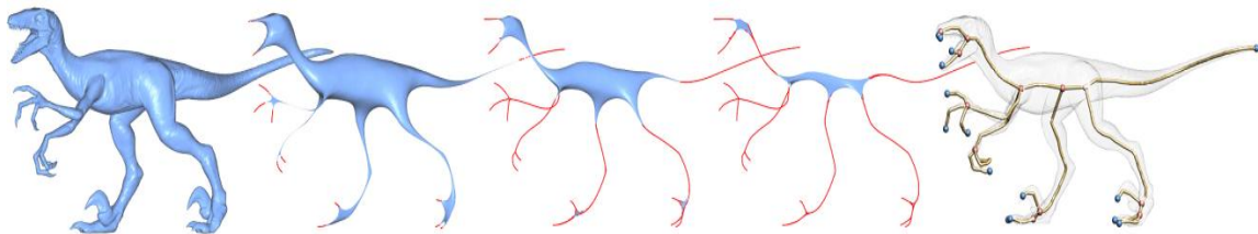
Figure 2-5 Mesh Contraction Method from Au [17]
