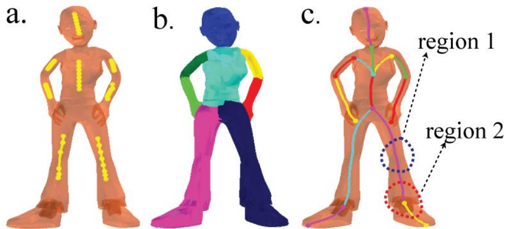
Figure 4-8 DP Algorithm in Skeleton Construction
