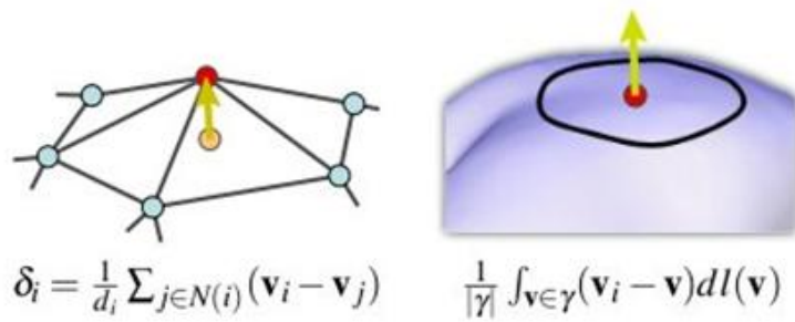
Figure 2-14 Differential Coordinates from [6]
