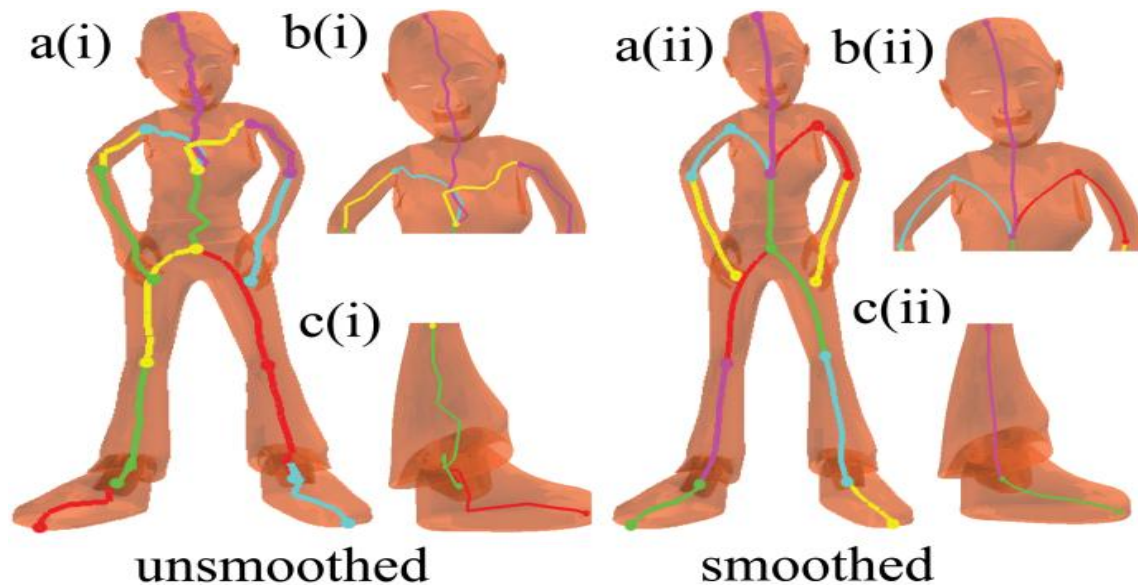
Figure 6-5 Skeleton Smoothing
