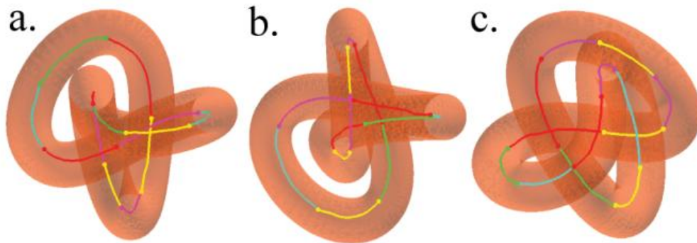
Figure 6-9 3D Donut
