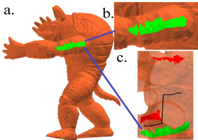
Figure 4-3 Projection Problem
