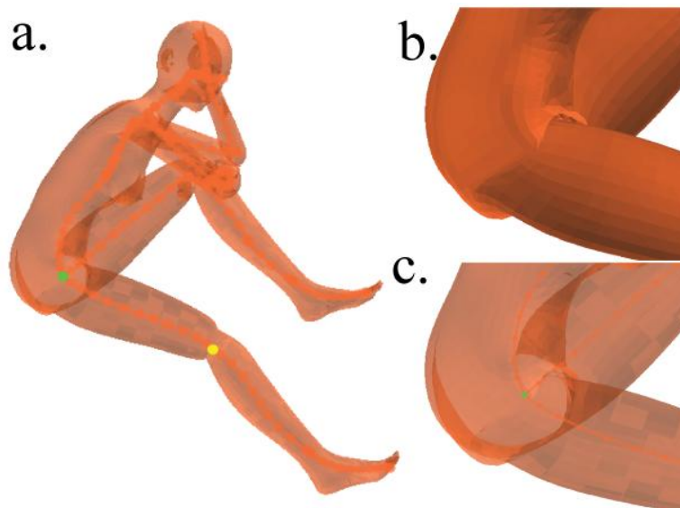
Figure 7-5 Laplacian Deformation with LBS result as constraints
