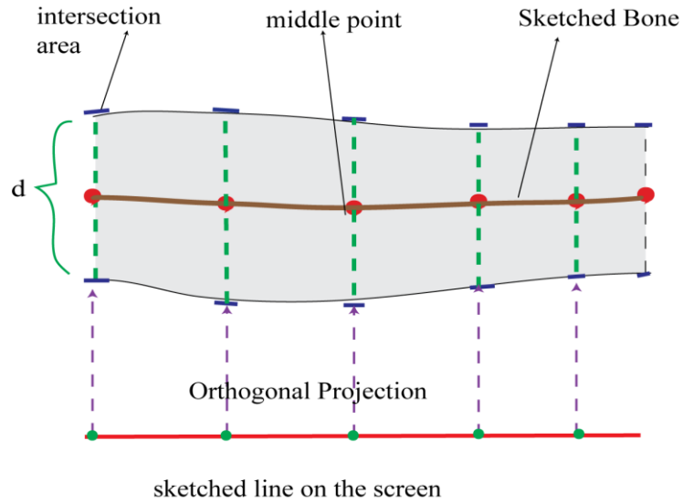
Figure 4-2 Our Projection Method
