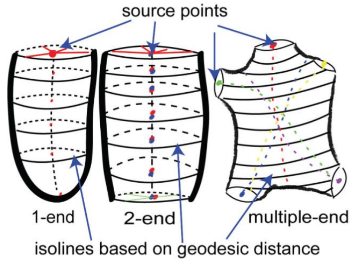
Figure 6-4 LSD Method
