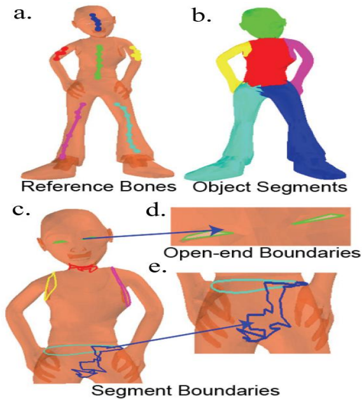
Figure 6-2 Segmentation Boundaries
