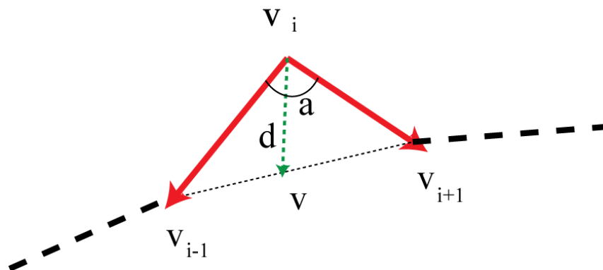
Figure 4-6 Smooth Operation
