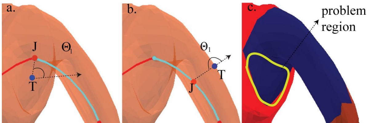
Figure 5-10 Segmentation Directions
