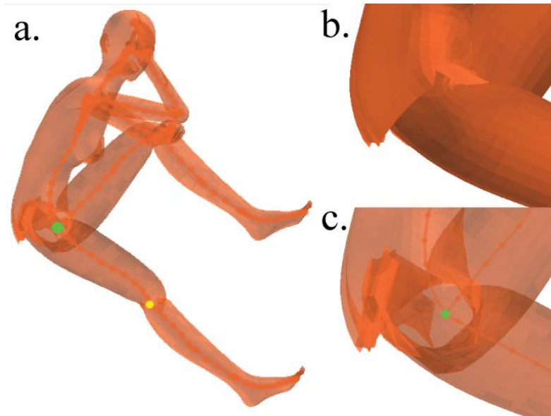
Figure 7-4 Self-Intersection Problem
