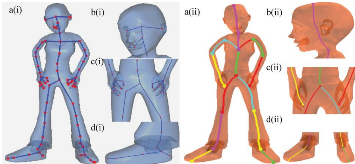
Figure 6-21 Resulted Skeleton from the Girl Model
