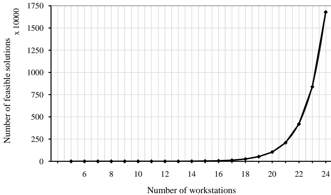
Figure 1.2: Growth of allocation of inspection stations problem search space. The horizontal axis is the number of workstations in an allocation problem. The vertical axis is the number of feasible solutions that have to be considered. The figure shows an exponential growth in search space size against problem size.
