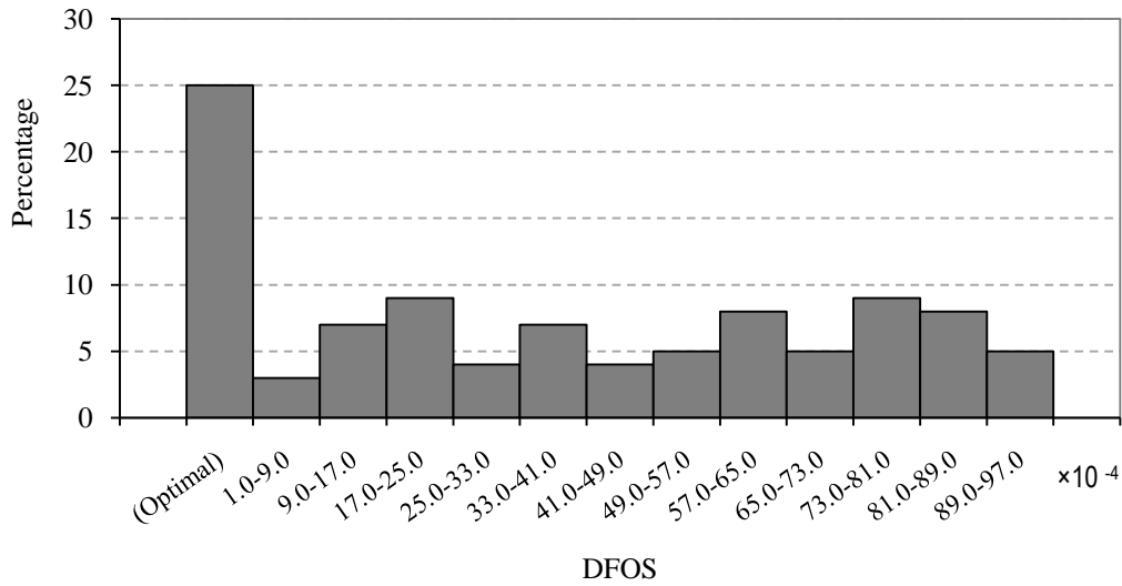
Figure 10.8: Percentage of DFOS histogram for GA
