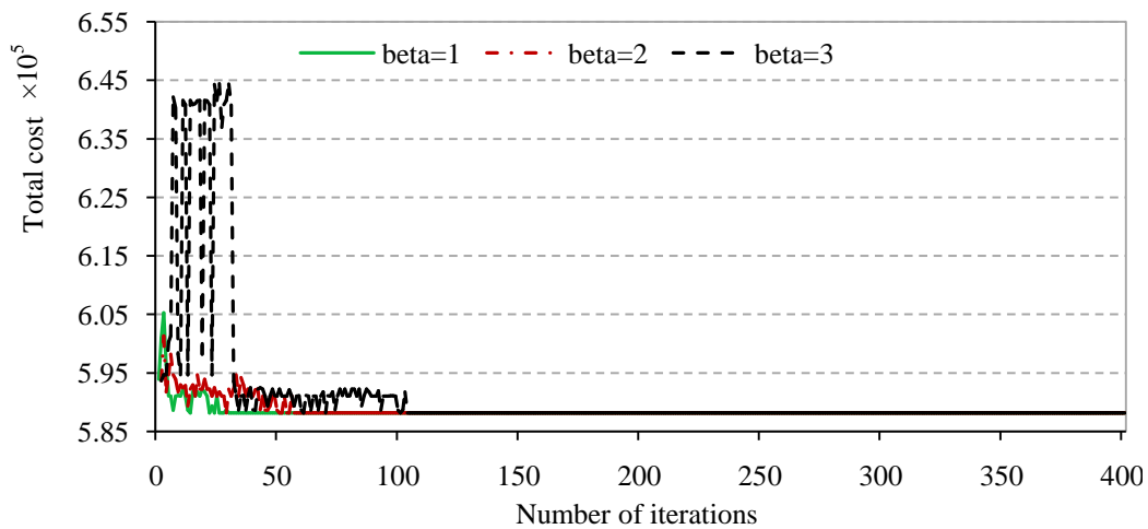
Figure 9.8: Comparing the convergence of MMAS under parameter settings \alpha = 2, \rho = 0.05
