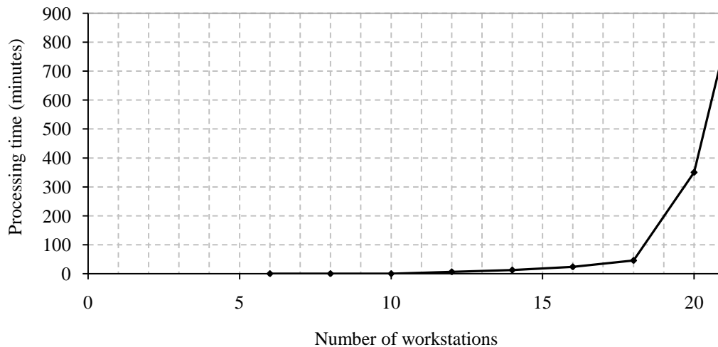
Figure 3.4: Schematic showing the duration of computational time against the number of workstations.
