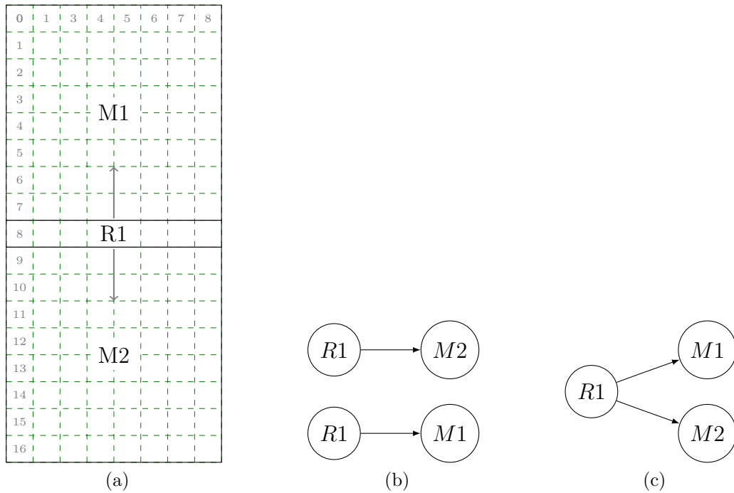
Figure 5.15: Modelling Rule Replication: the redundant block R1 can be placed in either M1 or M2. In part 5.15b this block has been incorrectly represented twice; the model of part 5.15c shows the correct representation.
