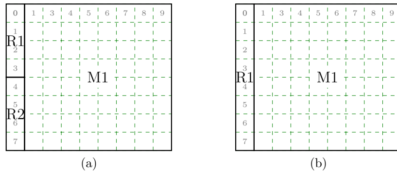
Figure 5.16: Modelling Rule Allocation: memory M1 has a single redundant column at x = 0 . Figure 5.16a incorrectly represents this as two redundant elements which must be allocated together. The correct representation as one redundant element is shown in 5.16b.
