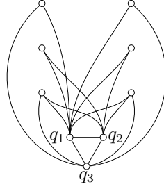
Figure 3.2: The graph G .
