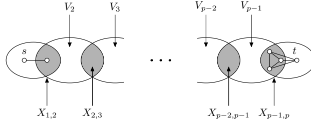
Figure 6.6: Structure of the graph G with respect to the clique separator decomposition \mathcal{C} .
