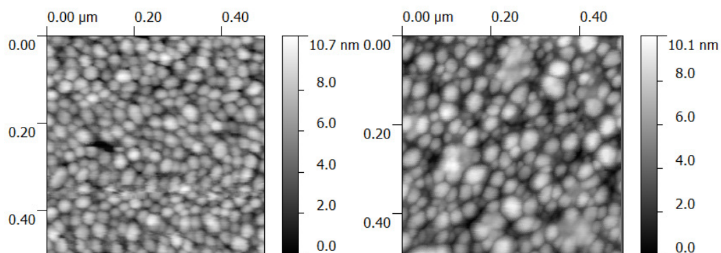
Figure 4.11 AFM of gold NPs on top of FET channel with (a) 25Å (b) 5Å of HfO 2 thickness
