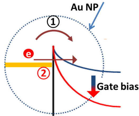
Figure 3.6 band diagram of plasmon FET a) with/Without gate voltage. With the applied gate voltage. Quantum tunneling effect in Au/ZnO/SiO 2 structure increases because gate voltage causes thinner barrier and enhances the tunneling efficiency.
