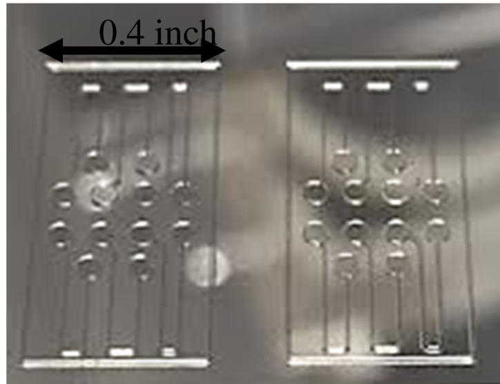
Figure 4.16 the fabricated microfluidic channel mold with Su-8 2075
