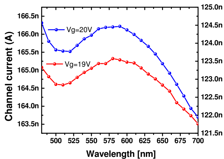
Figure 5.6 plasmon FET channel current using direct measurement
