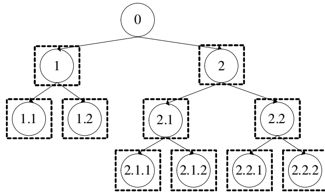
Figure 3.5: Local classifier per node. Circles represent classes and each dashed square encloses the classes predicted by a binary classifier.
