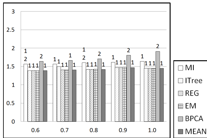
(c) NORM_missingX6_marX7
