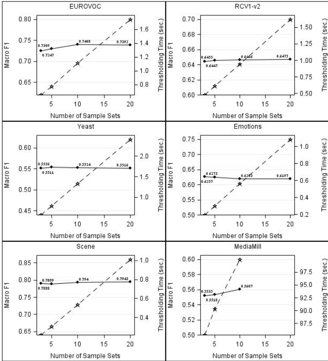
— Average Macro F1 - - - Average Thresholding Time
