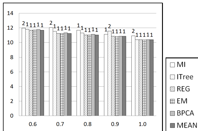
Figure A.4: Average RMSE of six imputation methods at different levels of missing probability on lognormal distribution data (LOGN) . X-axis is the probability of missing and Y-axis is the average RMSE. The number above each bar provides ranking of the performance.
