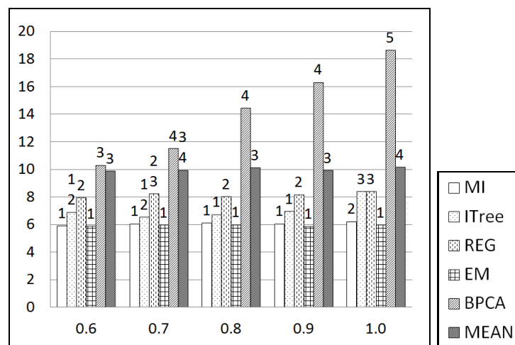
(b) PIMA_missingBMI_marSF
