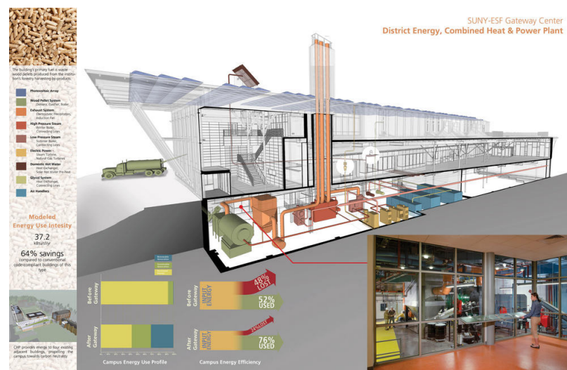
Figure 29: Diagram of Power Plant inside the Gateway Center. Courtesy of AIA.org
