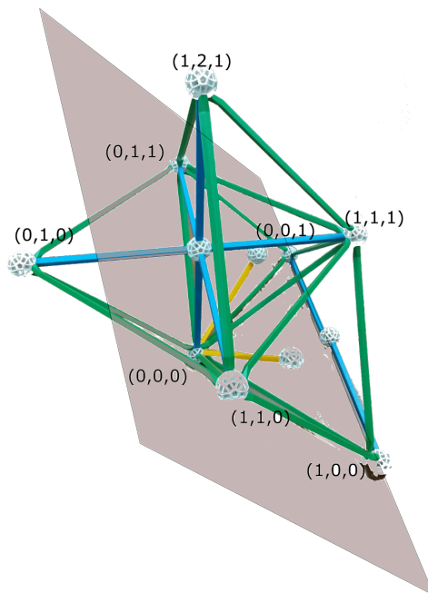
Figure 3.1: The Meinrenken tile for \mathfrak{S}_3 and the hyperplane corresponding to reflection R from Theorem 3.2.
