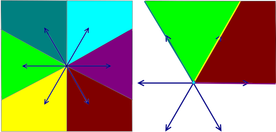
Figure 9: The chambers of the Coxeter arrangement for A_2 are on the left, and the corresponding Waldspurger decomposition is on the right. In the Waldspurger decomposition, three of the chambers collapse to rays, and the fundamental chamber collapses to a point at the origin.
