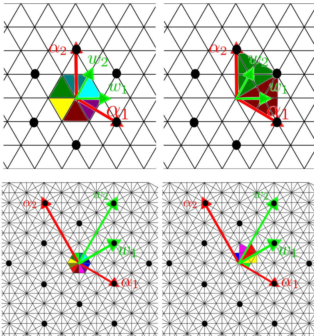
Figure 10: The subfigures on the left show a classical fundamental domain for the action of the coroot lattice in \tilde{A}_2 (on top) and \tilde{G}_2 (on bottom). On the right are the corresponding Meinrenken tiles. The Meinrenken tile for \tilde{A}_2 consists of a vertex at the origin, three open line segments, and two triangles. The Meinrenken tile for \tilde{G}_2 consists of a vertex at the origin, six open line segments, and five triangles. (See chapter 2 for types B and C pictures)
