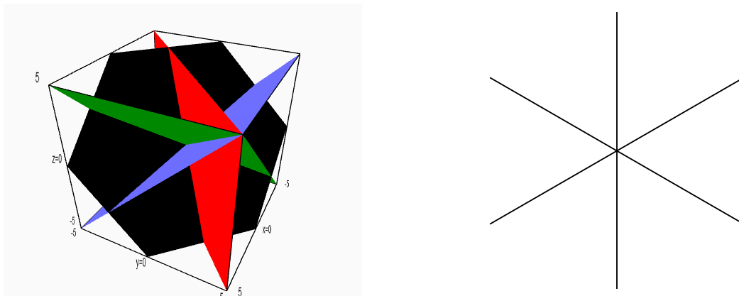
Figure 2: The Weyl group for A_2 is a finite real reflection group of rank 2, but its defining representation is of rank 3, generated by the hyperplanes x - y = 0 and y - z = 0 . Restriction to the hyperplane (1, 1, 1)^\perp yields the reflection representation.
