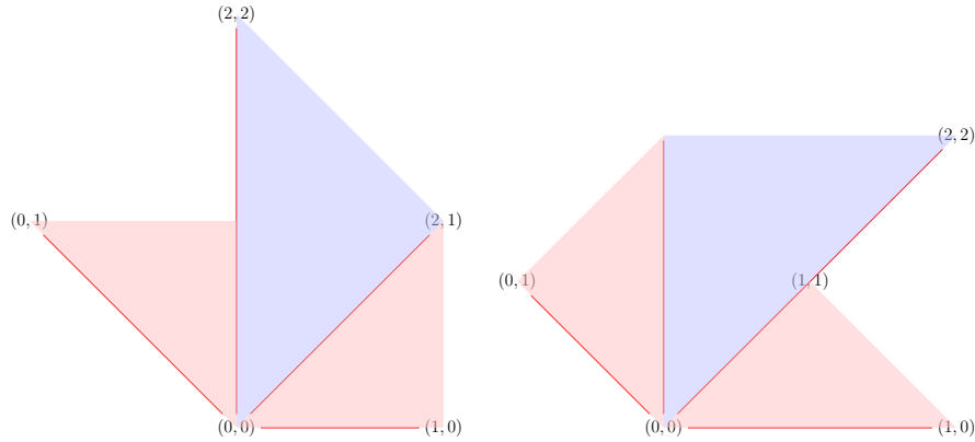
Figure 2.5: The Meinrenken tiles for C_2 and B_2 respectively
