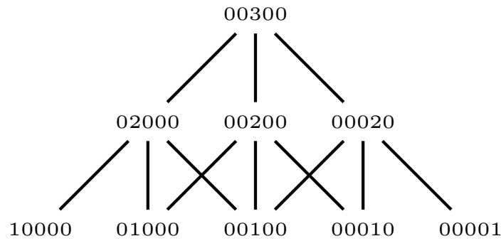
Figure 1.14: The lattice of M vectors of length five ordered componentwise is isomorphic to the lattice of order ideals in this poset
