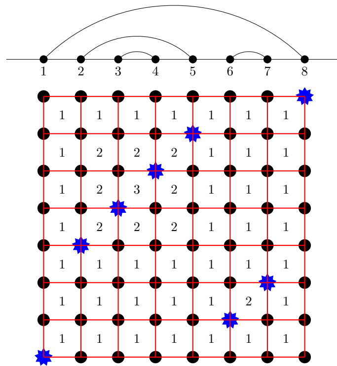
Figure 1.13: The permutation 85432761 is the unique permutation \pi \in \mathfrak{S}_8 with cycle decomposition a non-crossing pairing, and with \text{diag}(\mathbf{WT}(\pi)) = 1232121 .
