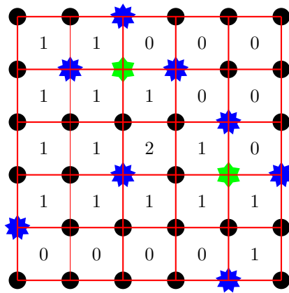
Figure 1.6: An ASM and corresponding monotone triangle, reduced monotone triangle, and generalized Waldspurger matrix. (The blue 9-sided stars represent 1's, and the green six-sided stars represent -1's in the transformation diagram.)
