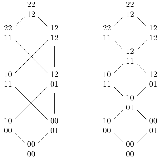
Figure 2.6: In the case of C_2 , (and B_2 , though it is not shown here) Waldspurger order is exactly Bruhat order, and componentwise comparison of folded centrally symmetric ASMs is exactly its Dedekind-MacNeille completion.
