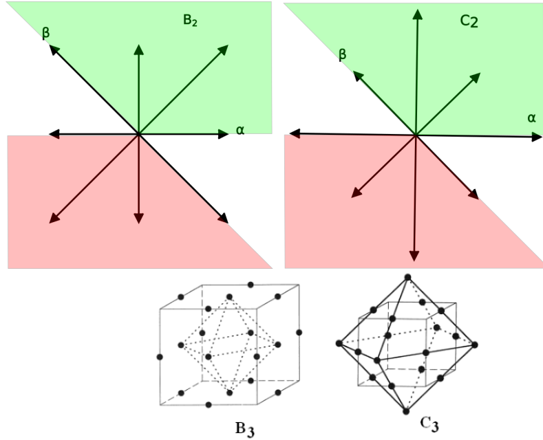
Figure 4: The regular hypercube and regular cross polytope have the same group of symmetries, but they give rise to non-isomorphic crystallographic root systems in all dimensions greater than two.
