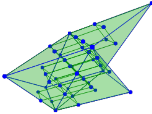
Figure 1.12: There are 38 lattice points in the permutohedron and 42 Alternating sign matrices in this dimension. Four of the interior points have multiplicity two.
