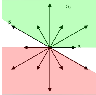
Figure 3: The G_2 root system with a choice of \alpha and \beta simple roots. The positive cone is in green, and the negative cone is in red.
