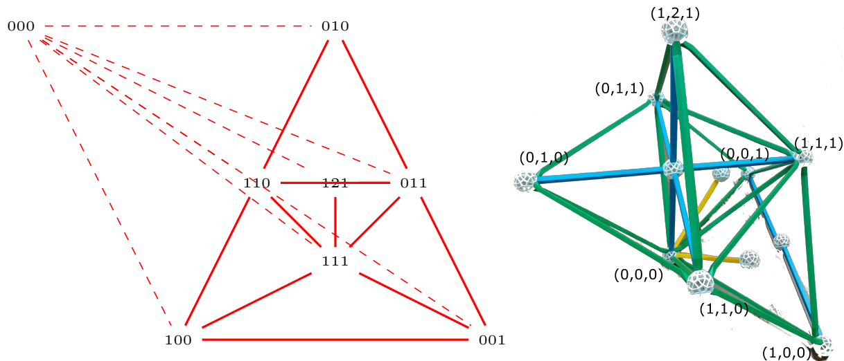
Figure 1.3: Waldspurger’s theorem decomposes the A_3 root cone (on the left) into a point at the origin, 6 one-dimensional cones (dotted rays), 11 two-dimensional cones, and 6 three-dimensional cones. Points are labeled in root coordinates. The A_3 Meinrenken tile is shown on the right constructed with Zometools. (The two yellow edges and one blue edge coming out from the origin are the fundamental weights.)
