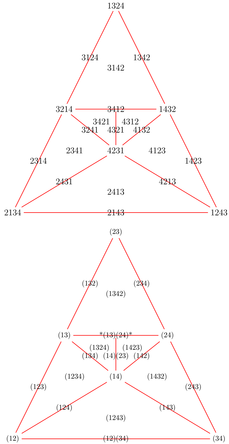
Figure 1.4: A slice of the Root cone A_3 = \mathfrak{S}_4
