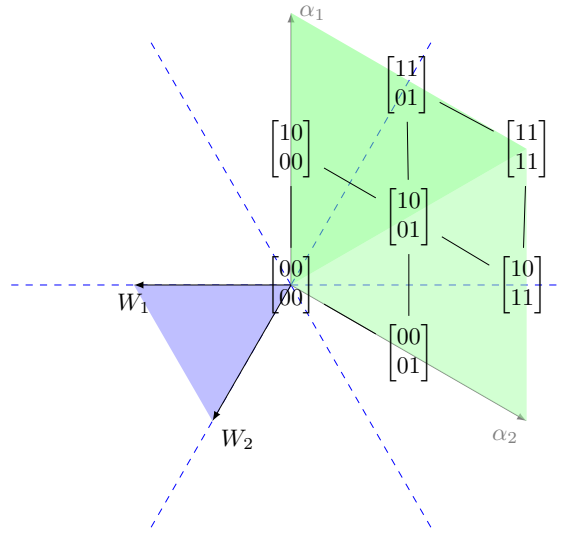
Figure 1.11: Place \mathbf{WT}(M) at the baricenter of \Delta_M for each M \in ASM to get a geometric realization of the Hasse diagram inside the Meinrenken tile
