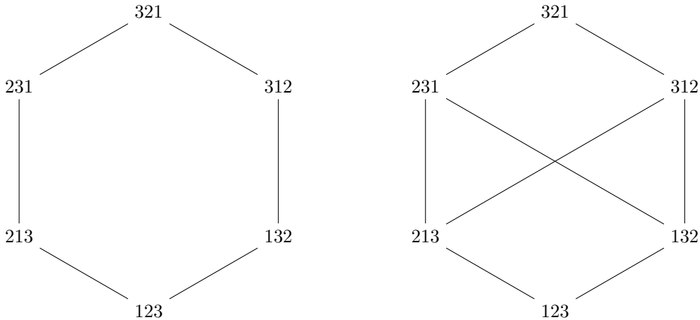
Figure 7: The hasse diagrams of the weak order and the (strong) Bruhat order for the Weyl group of A_2 .
