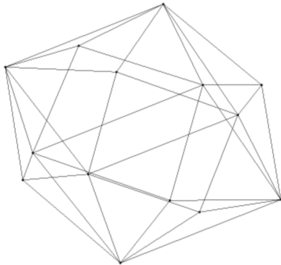
Figure 1.1: The polytope polar to the type A_3 permutohedron has 24 facets, each corresponding to a permutation of 4. It will tile \mathbb{R}^3 when translation by (co)root vectors.
