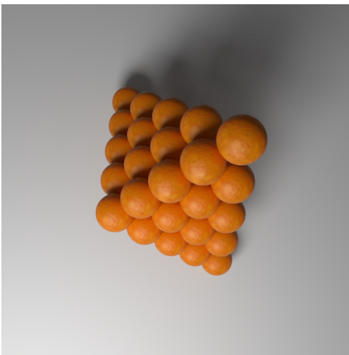
Figure 1.10: A tetrahedron of oranges sitting on its edge and viewed from on top. Stable configurations of oranges correspond to Waldspurger matrices, with the full tetrahedron corresponding to the Waldspurger matrix from Figure 1.9.
