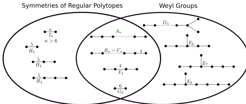
Figure 1: A subscript in the notation indicates the rank of the reflection group, which is the dimension of the representation. ( I_n is an exception. As the group is the symmetries of a regular n -gon, and is always rank 2.)
