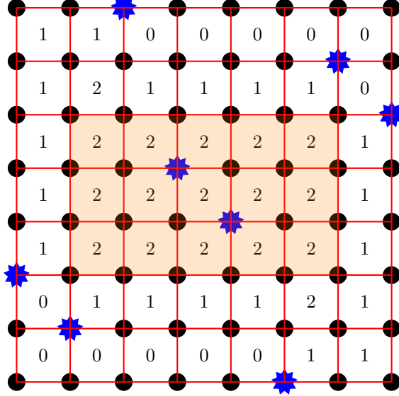
Figure 2.4: The transformation diagram for the join-irreducible J_{\Delta}((5, 2, 2), (3, 6, 2)) in BASM_4
