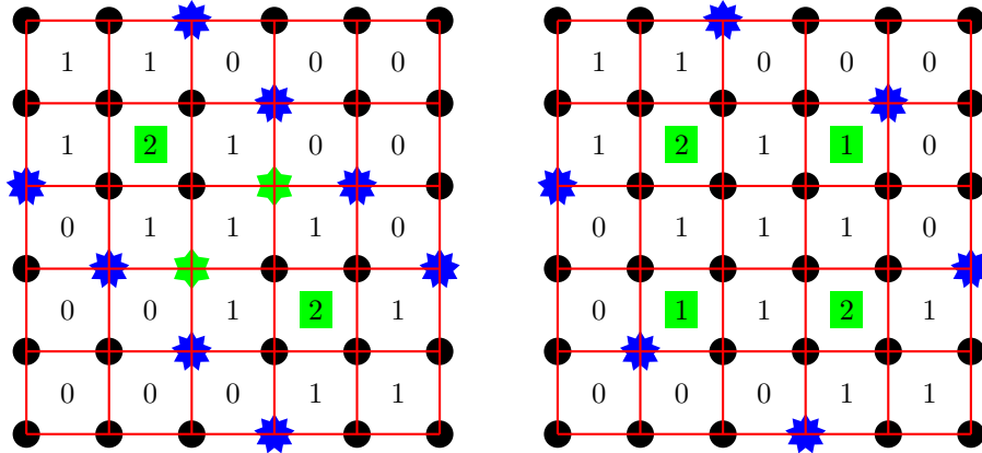
Figure 2.2: The transformation diagram for J_{\Delta}((2, 2, 2), (4, 4, 2)) in \mathbf{WT}(HTASM_6) on the left and for J_{\Delta}((2, 2, 2), (4, 4, 2), (6 - 2, 6 - 2, 1), (6 - 4, 6 - 4, 1)) on the right. These correspond to elements of P_1 and P_2 respectively. The left shows the smallest centrally symmetric ASM Waldspurger matrix with (2, 2) entry a 2. The right shows the smallest centrally symmetric (permutation) Waldspurger matrix with the (2, 2) entry a 2. It follows from Proposition 0.7 all of the elements in P_2 must come from permutations.
