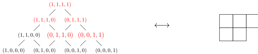
Figure 1.5: Abelian ideals in the nilradical of the Lie algebra \mathfrak{sl}_n correspond to certain order filters in the poset of positive roots and to Ferrer's shapes with hooklengths less than or equal to n . In this figure, each of the positive roots are given as vectors in simple root coordinates.
