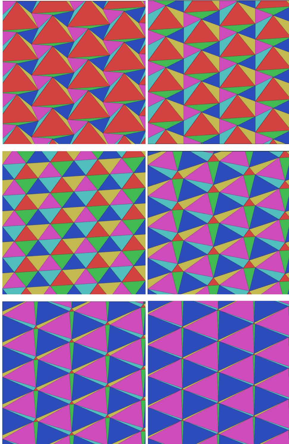
Figure 5: Each triangle in each figure is (S - w)A for A the fundamental alcove and w some element of the affine symmetric group, \widetilde{\mathfrak{S}}_3 . The six figures correspond to six different S , each a scalar times the identity. Reading left to right and top to bottom, the six scalar values are -0.8, -0.5, 0, 0.5, 0.8, 0.9 .
