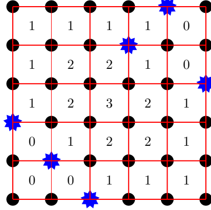
Figure 1.2: The transformation diagram for the permutation 456213 \in \mathfrak{S}_6 . The columns vectors give root coordinates for six points over which C_{456213} is a cone. A_{456213} is the convex hull of these vectors and zero.
