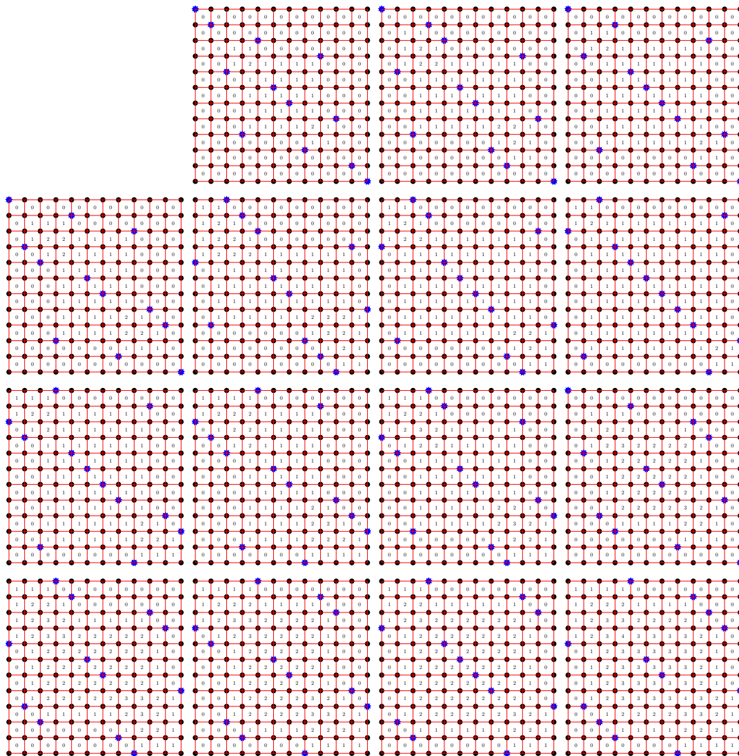
Figure 4: There are \binom{6}{4} = 15 Bigrassmannian elements in the Weyl group B_6 which are not join-irreducible in the Dedekind-MacNeille completion of Bruhat order. Here are the transformation diagrams for the corresponding centrally symmetric permutations in \mathcal{CS}_{12} .
