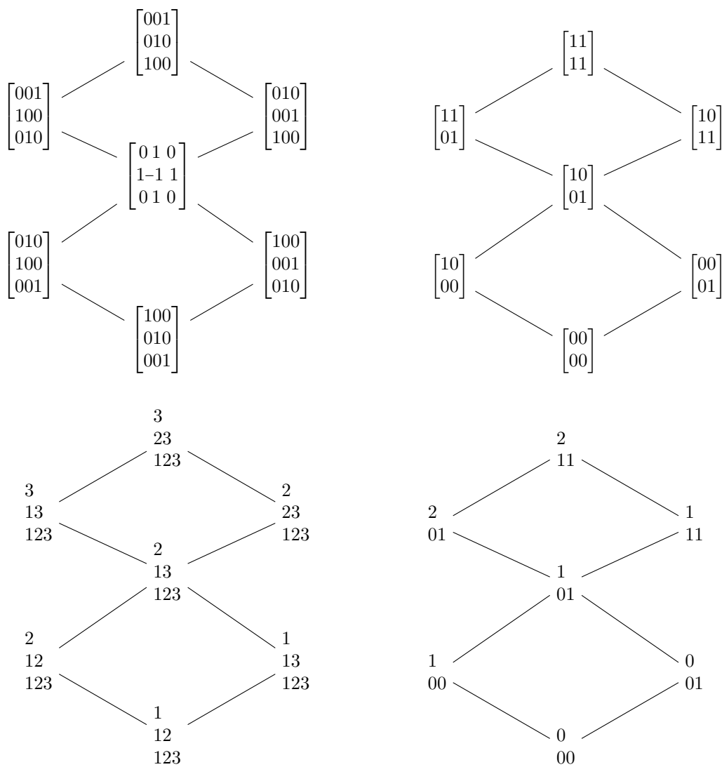
Figure 1.7: The Dedekind-MacNeille completion of Bruhat order A_2 viewed as ASMs, Generalized Waldspurger Matrices, monotone triangles, and reduced monotone triangles
