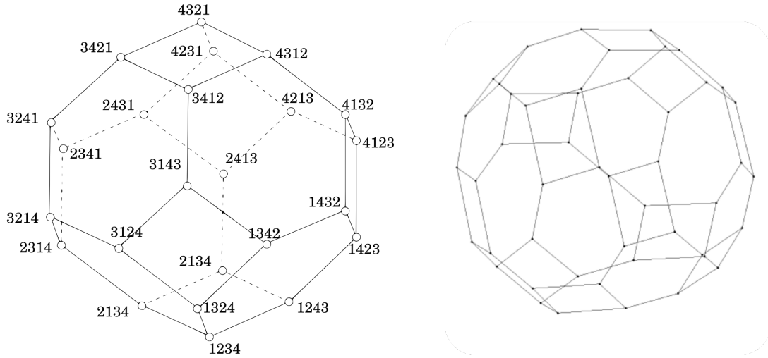
Figure 6: The graph of the Permutohedron of type A_3 is also the Hasse diagram of the weak order on the Weyl group of A_3 (i.e. the symmetric group \mathfrak{S}_4 ). The Permutohedron of type B_3 is shown on the right.
