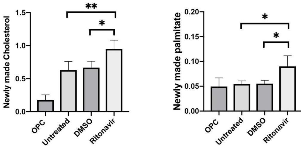
Figure 17: Ritonavir increased levels of newly synthesized palmitate and cholesterol. OPCs treated with DMSO (vehicle) with or without 3 \mu M of ritonavir for three days, ^{13} C acetate was added to the differentiation media for the last 24 hours of treatment. Both newly-made palmitate and cholesterol are increased in cells labeled with acetate compared to DMSO-treated or untreated groups. N=3, * P<0.05, ** P<0.01
