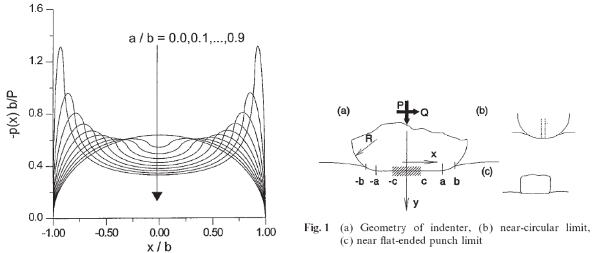
Figure 1. Contact Pressure Distribution [1]
