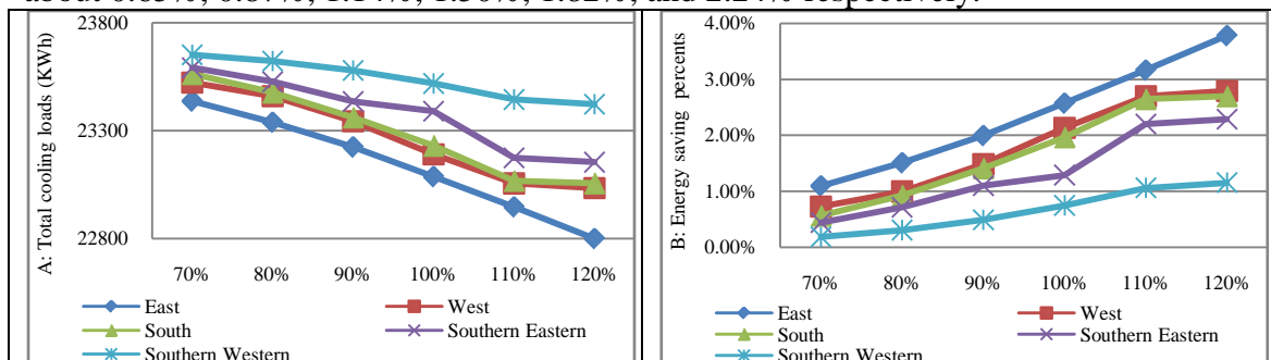
Figure (4.54): The effect of increasing crown size of vase tree on A: cooling loads, B: energy saving in summer
