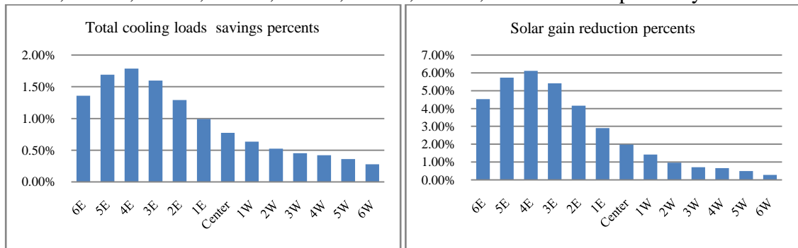
Figure (4.42): Energy savings percents in summer and solar gain reduction percents (in south façade)
