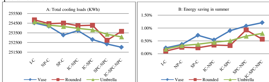
Figure (5.28): A: Total cooling loads amount (KWh), B: Energy saving percents for multiple street trees planting locations
