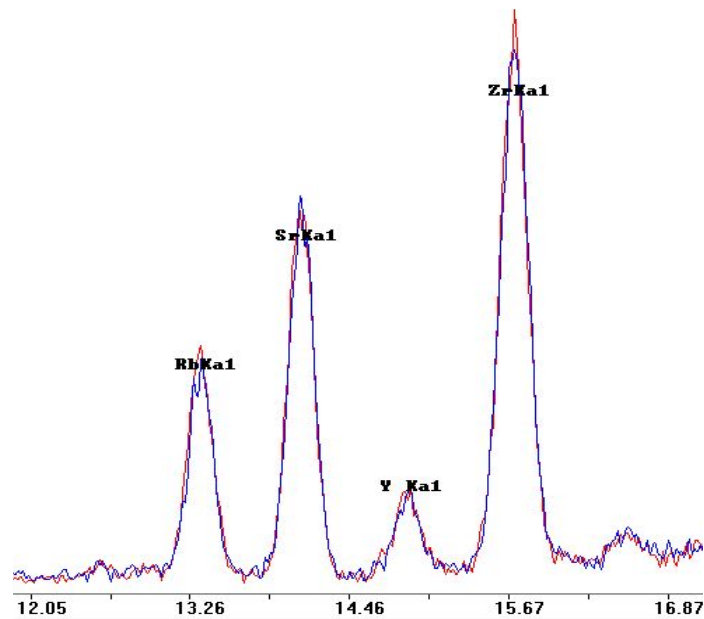
Figure 13. Spectra overlay of Ixtepeque obsidian. The blue spectrum represents the comparative samples while the red spectrum represents the study sample. Although the spectra do not align exactly the pattern of peaks is the same. Rb stands for rubidium, Sr stands for strontium, Y stands for yttrium, and Zr stands for zirconium. Image created by K. Johnson.
