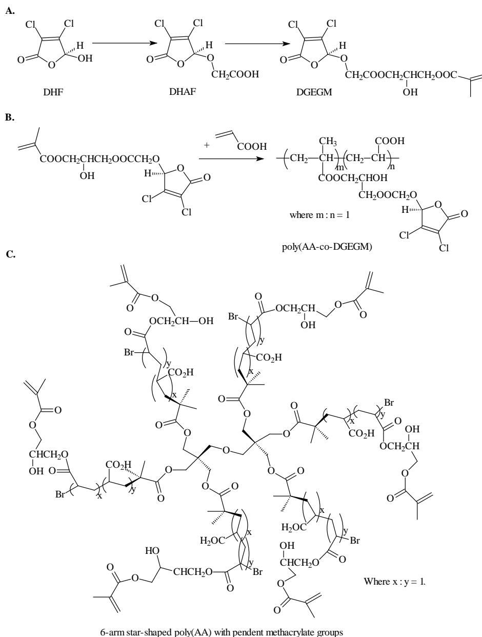
Figure 2.1 Synthesis schematic diagram for: A. DGEGM synthesis, B. poly(AA-co-DGEGM) synthesis, C. structure of the 6-arm star-shaped poly(AA) with pendent methacrylates.
