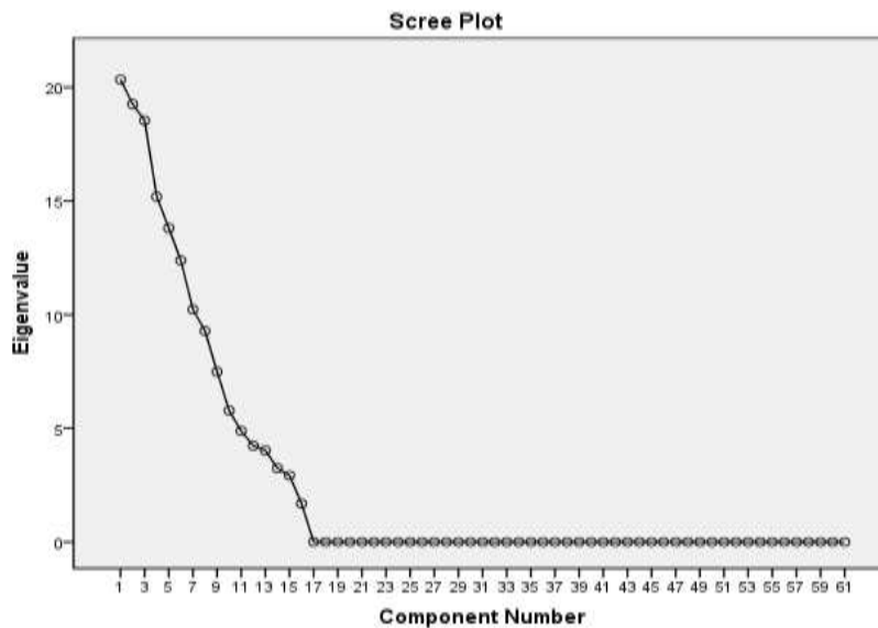
Figure 5.7 – Scree Plot Diagram
