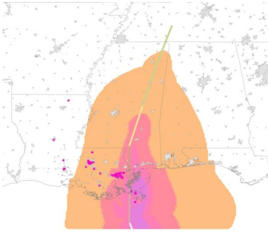
Figure Set B.4: Extent of Wind Grid
