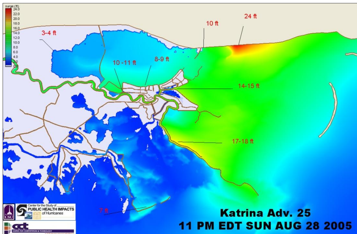
Figure 5.28: The maximum surge height of Hurricane Katrina based on an ADCIRC simulation (van Heerden, et al. 2007).
