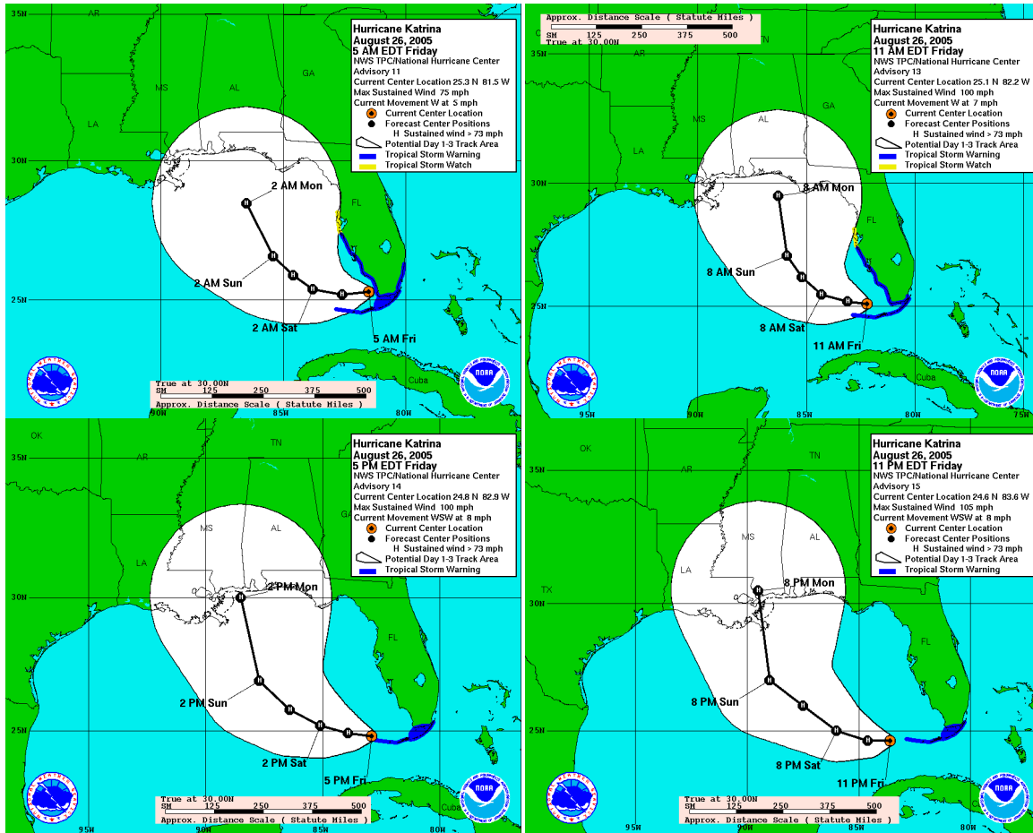
Figure 4.1: Katrina Advisories from Friday, August 26, 2005.
