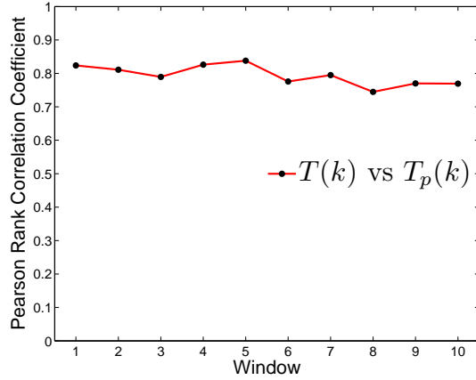
Figure 5.3: Correlation between topics' popularities at network level
