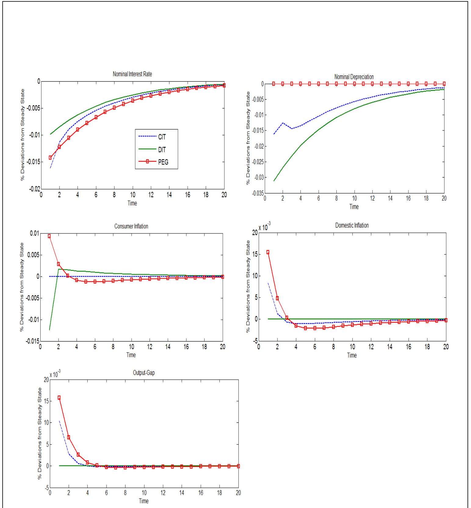
Figure 5 Impulse Responses to a Foreign Output Shock: Targeting Rules.
