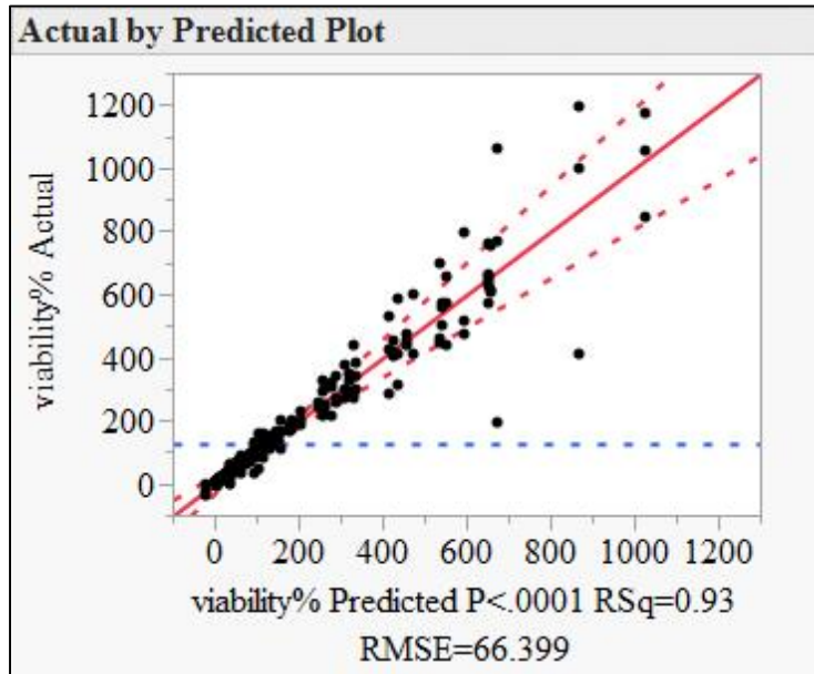
Figure 8a Statistical analysis of cell viability test setting a). Actual data plotted against predicted model as black dots against red line
