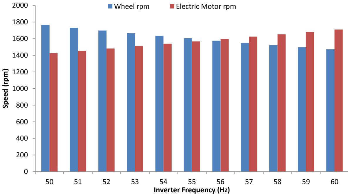
FIGURE 4.12: VARIATION IN SPEED AT DIFFERENT INVERTER FREQUENCY
