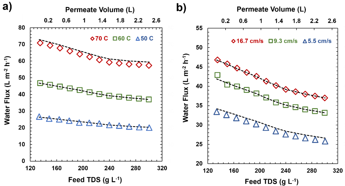
Fig. 4. Experimental and predicted water flux as a function of feed TDS and permeate volume for synthetic HFPW at a) different feed temperatures with flow velocity fixed at 16.7 \text{ cm s}^{-1} and b) different flow velocities at 60 \text{ }^\circ\text{C} feed temperature. Synthetic water, containing 135 \text{ g L}^{-1} sodium chloride in DI water, was used as feed and make-up water. Experiments were carried out with feed outlet line closed. Distillate stream was kept at 20 \text{ }^\circ\text{C} for all case studies.
