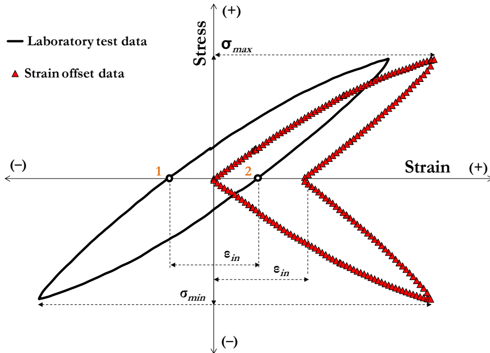
Figure 6.6. Illustrative cyclic stress-strain loading history of a symmetrically loaded LCF test. Here, \sigma_{max} and \sigma_{min} correspond to the maximum tensile and compressive stresses, respectively and \epsilon_{in} , the total inelastic strain accumulated till the end of the loading cycle under consideration.
