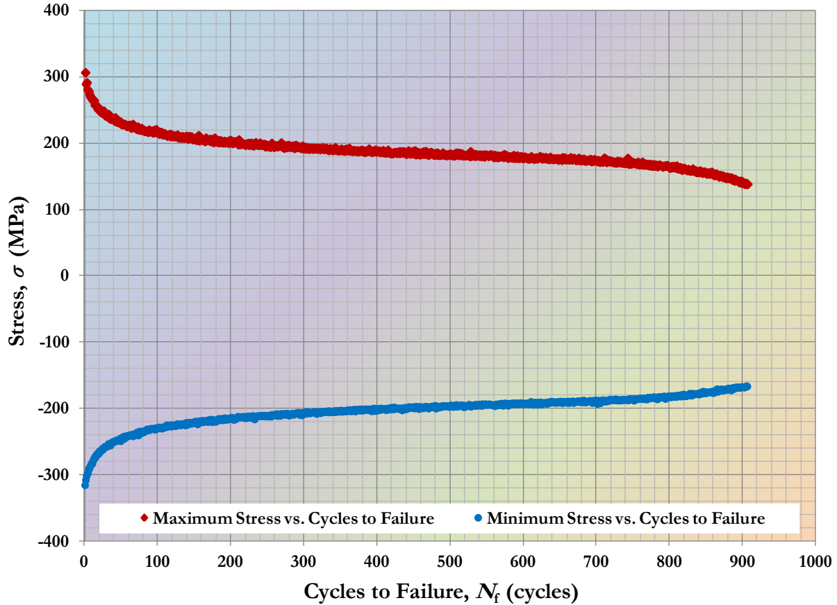
Figure 7.4. Typical variations in maximum and minimum stress with loading cycles as observed in cyclic deformation response of grade P91 steel without hold time (Data courtesy of one of the RR participants).
