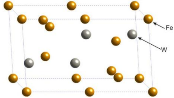
Figure 3.4. Schematic of HCP unit cell structure of \text{Fe}_2\text{W} precipitates [125].
