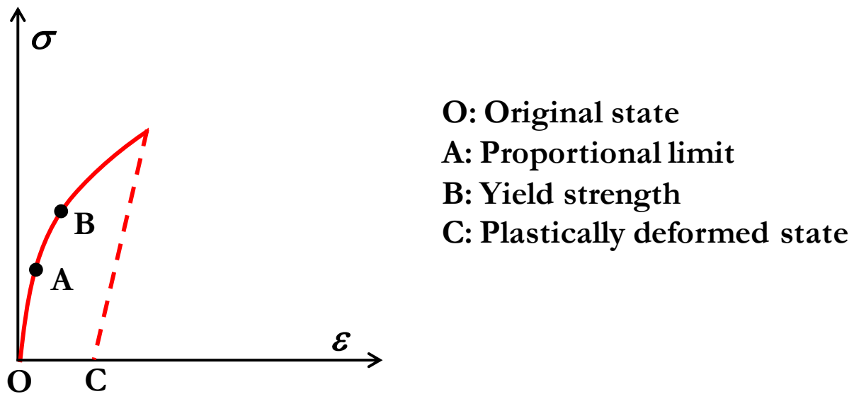
Figure 2.7. Typical stress-strain curve obtained for a uniaxial monotonic tensile test.
