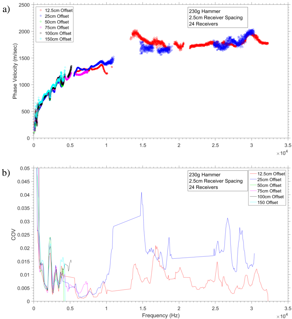
Figure 4-16. Comparison of the dispersion and COV curves for source offsets of 12.5 cm, 25 cm, 50 cm, 75 cm, 100 cm, and 150 cm at CTP Asphalt. A 230g hammer and a receiver array of 24 receivers with a 2.5 cm receiver spacing were used for the comparison.
