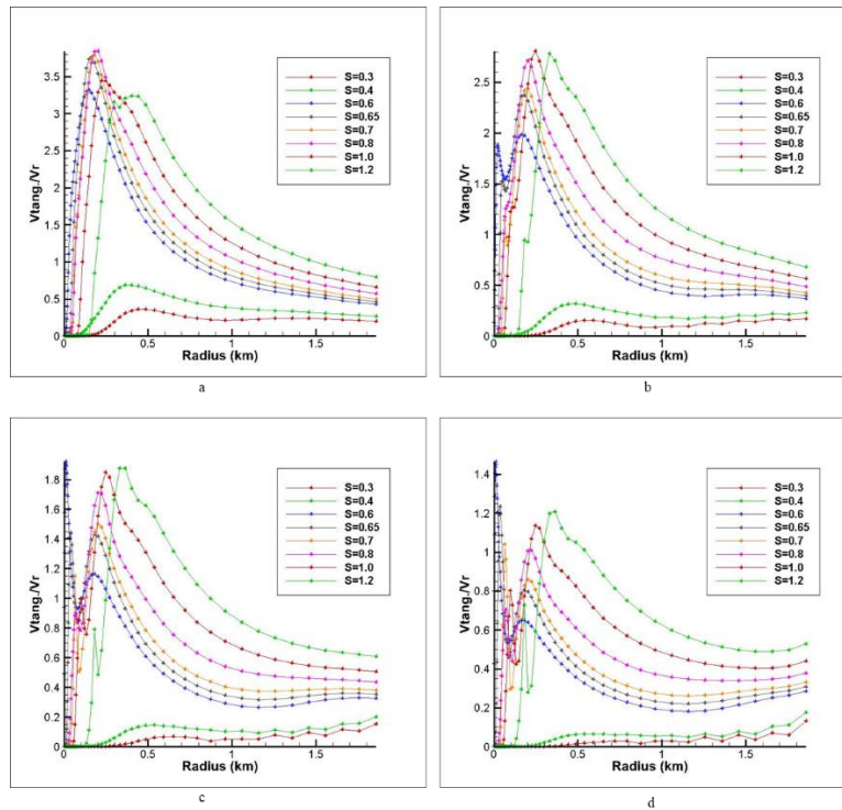
Figure 4.14. Radial V_\theta profile of different swirl ratios for r_0=1.8\text{km} . a) z=51\text{m} ; b) z=18.5\text{m} ; c) z=9.5\text{m} ; d) z=4.5\text{m}
