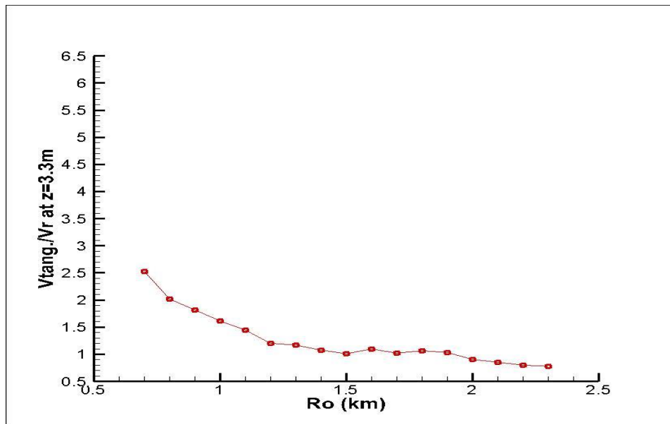
Figure 4.3. V_{\theta, \max} at z=3.3\text{m} for different r_0 radii ( V_{\theta, \max}/V_{r\infty} )
