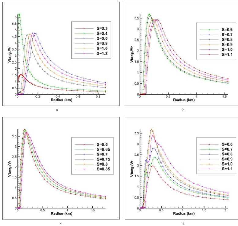
Figure 5.3. Radial V_{\theta} profile at z=51 m AGL. a) r_o=0.8 km; b) r_o=1.5 km; c) r_o=1.7 km; d) r_o=2.0 km
