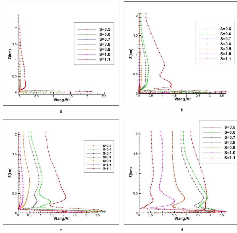
Figure 4.9. Vertical V_\theta profile of different swirl ratios for r_o=1.5\text{km} . a) r=33 ; b) r=88\text{m} ; c) r=r_c=148\text{m} ; d) r=245\text{m}
