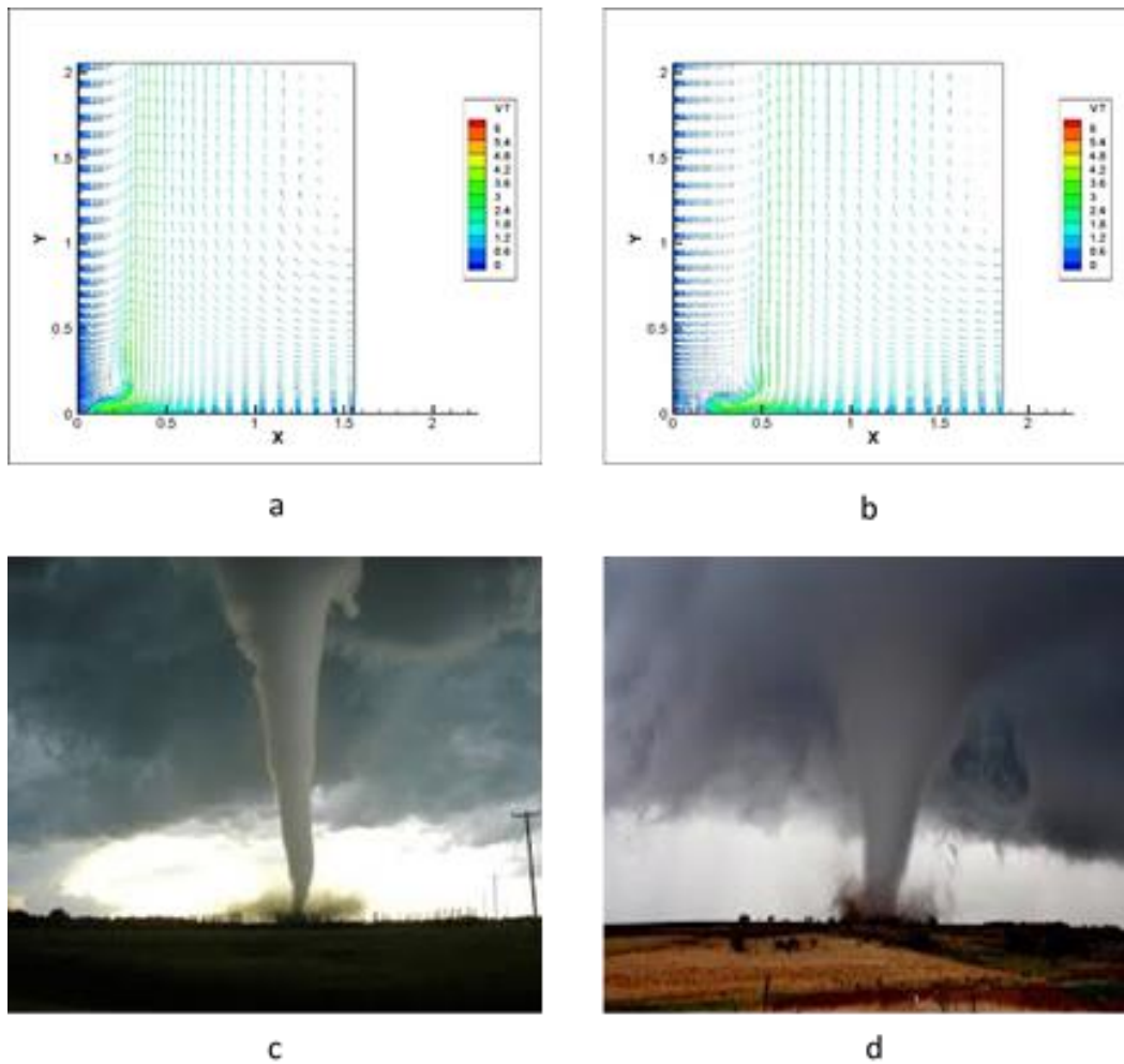
Figure 4.5. The outward expansion of tornados with larger r_0 . a) r_0=1.5 km; b) r_0=1.8 km; c) actual tornado with small radius; d) actual tornado with large radius
