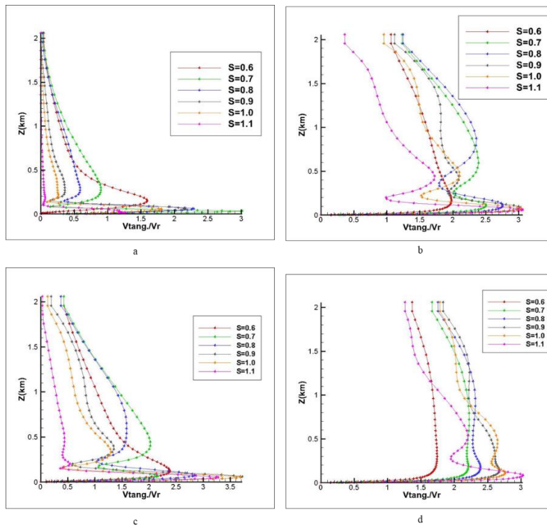
Figure 4.10. Vertical V_\theta profile of different swirl ratios for r_o=2.0\text{km} . a) r=50 ; b) r=150\text{m} ; c) r=r_c=271\text{m} ; d) r=490\text{m}
