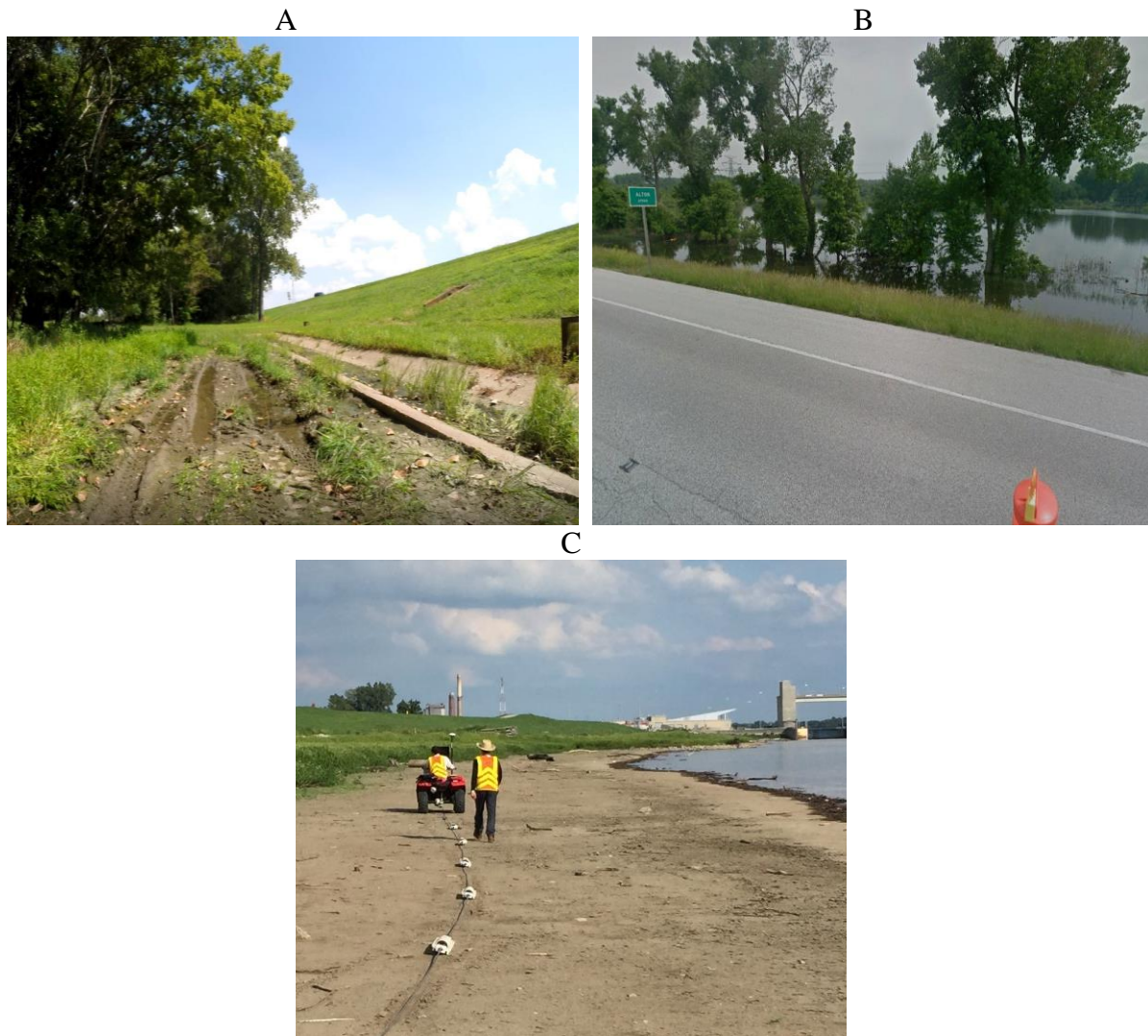
Figure 3-12. A) Visible surface water at landside of Mel Price Levee at sta. 123+00, B) View from top of road showing the pond along the landside of the Mel Price Levee at sta 95+00, and C) OhmMapper towed along riverside of Mel Price Levee at sta 82+00.
