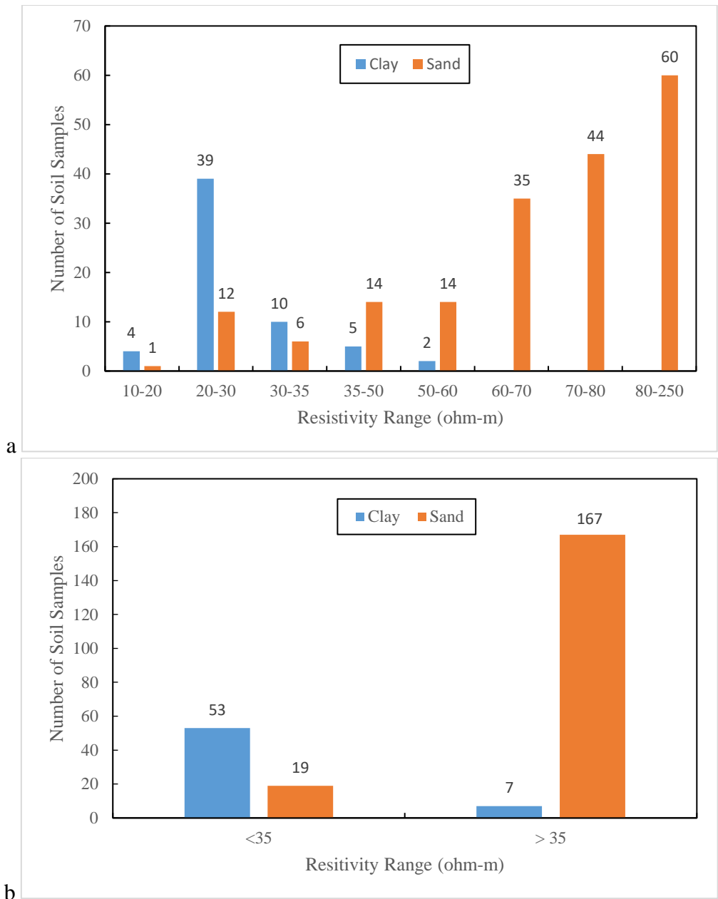
Figure 4-8. a) Distribution of soil samples b) Distribution of soil samples either side hypothetical resistivity separator between clay and sand samples based on their resistivity at landside of Mel Price site.
