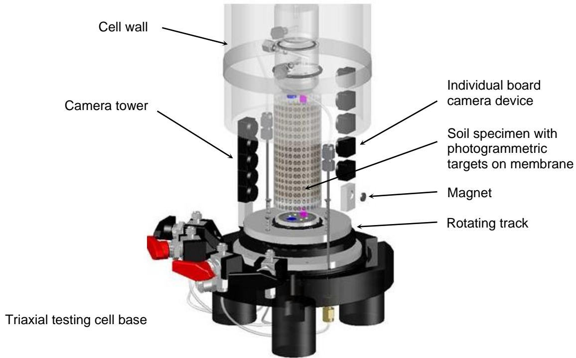
Figure 1.1. Exploded, transparent view of the major components of the internal camera-based photogrammetry system (note: shown with piezoelectric transducer end caps).
