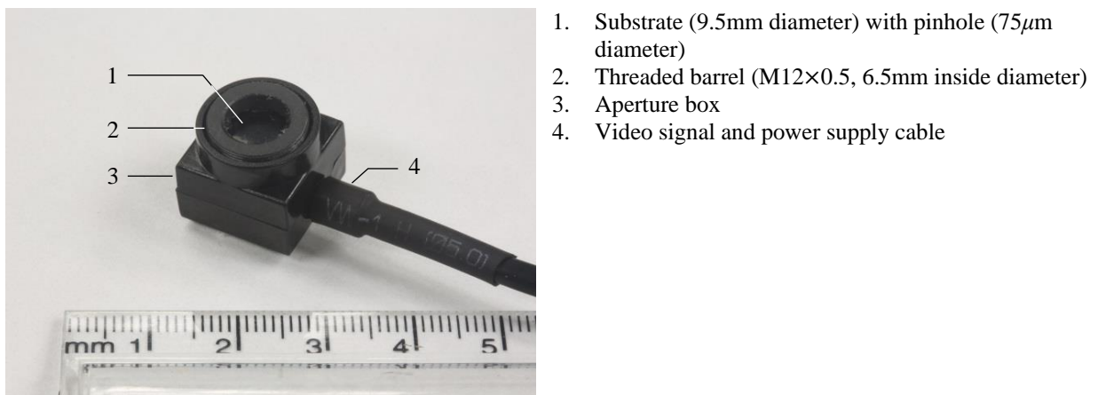
Figure 3.6. Photograph of one of the BCPAs utilized inside of the triaxial cell.
