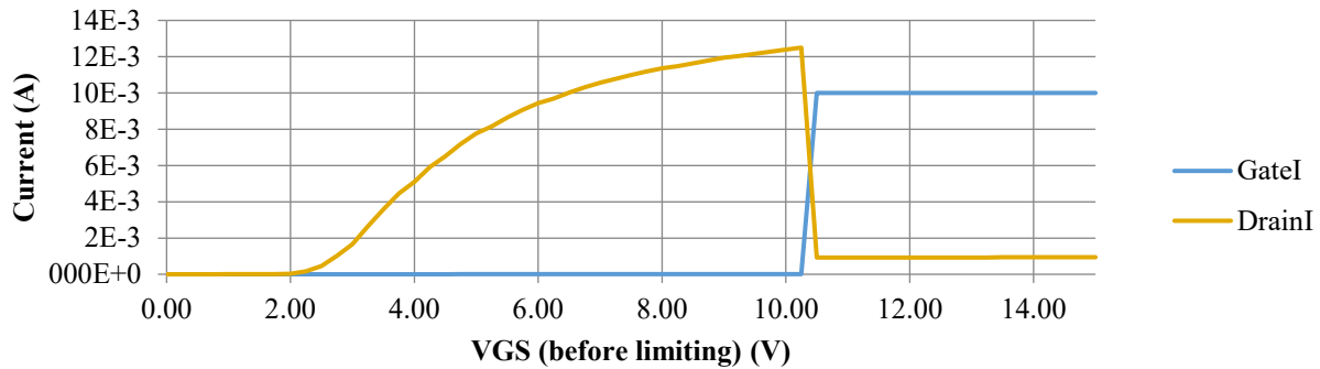
Fig. 6.2. Gate oxide breakdown on a 1.2\ \mu\text{m} channel length transistor during a V_{GS} sweep, with a V_{DS} of 0.1\ \text{V} . Breakdown occurs at a V_{GS} of 10.5\ \text{V} , and I_G reaches the programmed current limit of 10\ \text{mA} . Subsequent runs indicate a gate-source short of 375\ \Omega .
