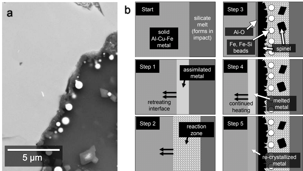
Figure 2.10: Redox reaction at metal-matrix interface. (a) BSE image showing close-up of Location f.8 (Fig. 2.2b). Metallic Fe beads occur mostly along interface between Al-Cu-Fe metal and glass. Spinel crust surrounds the Al-Cu-Fe metal grains. The Fe beads and spinel crust are the products of a redox reaction between Al-Cu-Fe metal and silicate melt. (b) Schematic illustration showing a proposed sequence of how the interaction unfolded between Al-Cu-Fe metal and silicate melt. The Start panel represents the initial contact between metal and silicate melt. In Step 1 , the metal is being partially assimilated into the melt, which leads to an enrichment of Al, Cu, and Fe in the melt. The metal-matrix interface retreats into the metal. In Step 2 , the interface continues to retreat, while the redox reaction occurs in the reaction zone, producing oxidized Al and metallic Fe and Si. In Step 3 , the interface stops retreating and the redox reaction stops, as various phases begin to crystallize, including a layer of Al-oxide (“Al-O”), spinel crystals, and Fe and Fe-Si beads. In Step 4 , the metal grains are still being heated. Some, like the one represented here, begin to melt, beginning at the metal-matrix interface. In Step 5 , the system cools, and the newly melted metal regions re-crystallize. This final panel reflects what is observed in (a).
