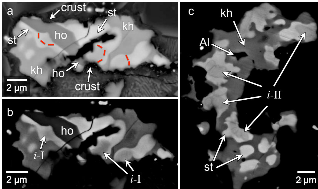
Figure 2.4: BSE images of Al-Cu-Fe assemblages with two generations of quasicrystals. Compositions for the metal phases shown here are listed in Table 2.1. Contrast in (b) and (c) has been stretched to emphasize compositional differences among the different metal phases. (a, b) Close up of Location 8 (Fig. 2.2a). This assemblage contains khatyrkite (“kh”), stolperite (“st”), hollisterite (“ho”), and icosahedrite (“i-I”). The red, dashed lines in (a) outline the icosahedrite grains to distinguish these grains from the neighboring phases; these sketches of the phase boundaries are based on higher contrast images of the same region, such as shown in (b). The upper and lower ends of the hollisterite grain terminate against the spinel crust (“crust”). We interpret this as a cross-cutting relationship that indicates the hollisterite and i-I are relict. The dark area in the center of the Al-Cu-Fe assemblage is a hole. (c) Close up of Location 10 (Fig. 2.2a). This assemblage contains quasicrystals (“i-II”) that are distinct from i-I. Surrounding i-II is stolperite, which is surrounded by khatyrkite. The dark area in the interior of this assemblage is metallic Al (“Al”). The dark area external to this assemblage contains silicate phases, which are not discernable in this image because of the high contrast.
