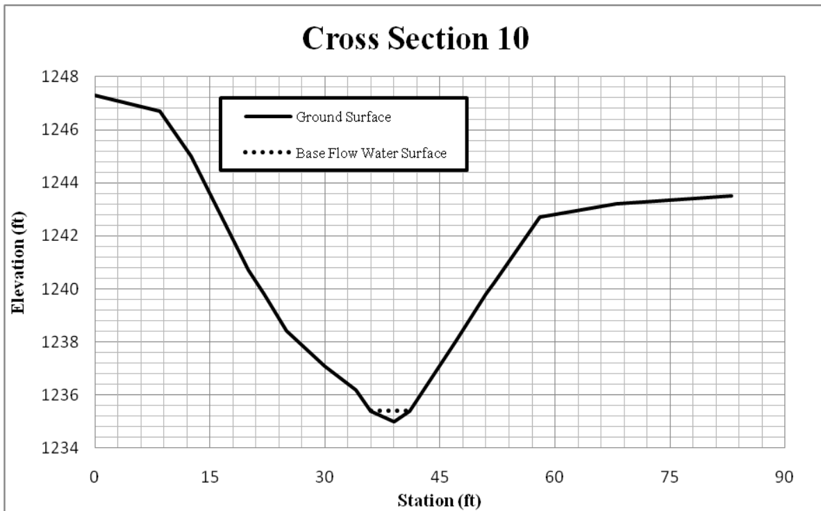
Figure I12. Cross-Section 10
