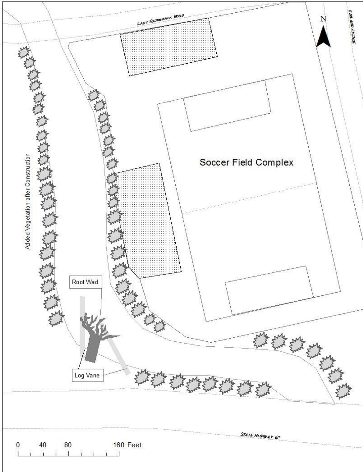
Figure 19. Log Vane and Root Wad Conceptual Design
