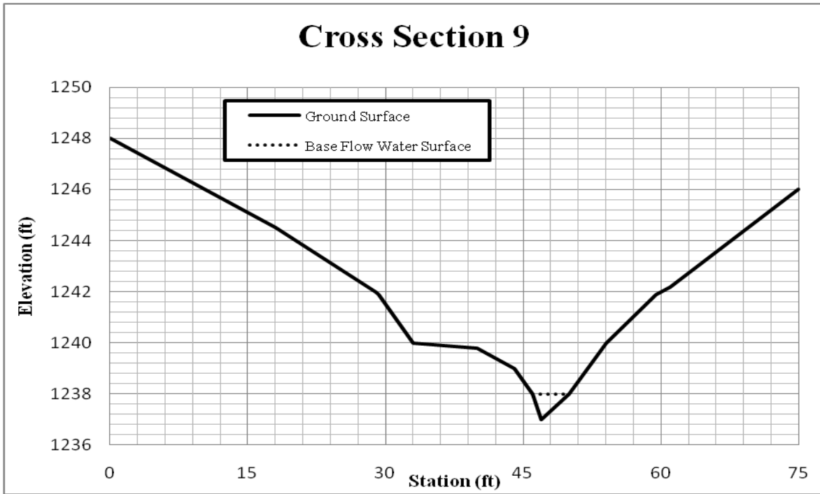
Figure I11. Cross-Section 9
