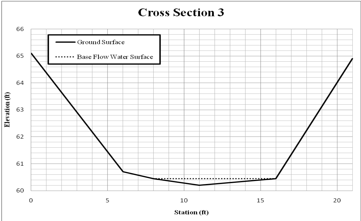
Figure I5. Cross-Section 3
